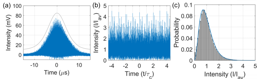
Fig. 5. (a) Intensity of a QS pulse. Gray trace: sech 2 profile, shifted upwards to ease the comparison. (b) Quasiperiodic intensity, relative to the mean intensity, extracted from the peak of a typical QS pulse. (c) Intensity probability density: Histogram, experimental data. Blue trace: Gamma distribution with m = 3.4 . In (b) and (c) the cavity's roundtrip time was \tau_c = 98.4 ns.
