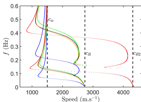
FIG. 3. (Color online) Group speeds of the first two modes vs frequency: in black, calculated with the physical parameters in Table I; in blue, with the parameters in Table I, but an ocean depth of h = 6000 m; in green, with the same parameters but a different sound-speed ( c_w = 1550 \text{ m s}^{-1} ); in red, with the parameters in Table I, but different seismic velocities in the crust ( c_P = 8100 \text{ m s}^{-1} , c_S = 4700 \text{ m s}^{-1} , c_{R2} = 4310 \text{ m s}^{-1} ); and in orange, with the parameters in Table I, but a crust of density \rho_s = 2700 \text{ kg m}^{-3} .
