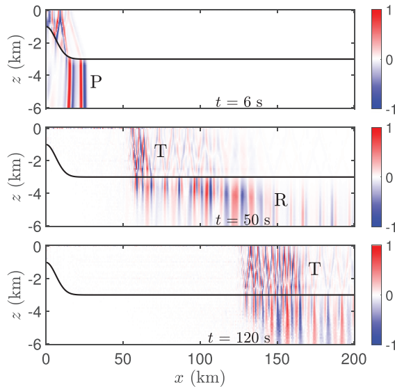
FIG. 5. (Color online) Snapshots of the acoustic pressure above and below the seafloor (black line), normalized by their maximum at each (x, z) point, at 6, 50, and 120 s since the beginning of the simulation (Configuration 2 with a 1 Hz-source). In the solid medium, the “pressure” is actually minus the third of the trace of the stress tensor. Capital letters denote the arrival fronts of P waves (P), precursory waves with a speed equal to c_R (R) and T waves (T).
