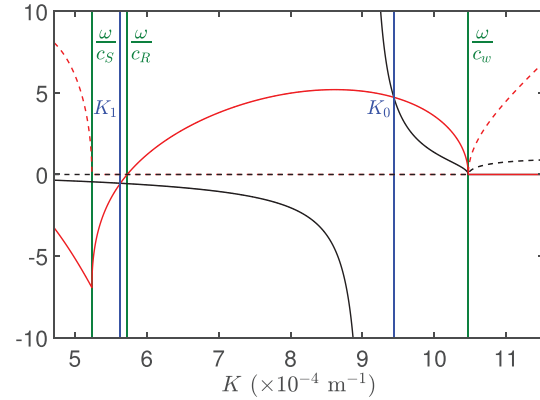
FIG. 1. (Color online) Wavenumbers of the modal solutions of Eq. (1) for the frequency f = 0.25 Hz (i.e., fh/c_w = 0.5 ). The right-hand member of Eq. (1) is plotted in red and the left-hand member \tan(lh) in black. The real part of each member of the equation is represented by the solid line and the imaginary part by the dashed line. The annotated blue lines show the two wavenumbers that verify Eq. (1) and the annotated green lines the wavenumbers corresponding to the phase speeds c_S , c_R , and c_w . Physical parameters are from Table I.
