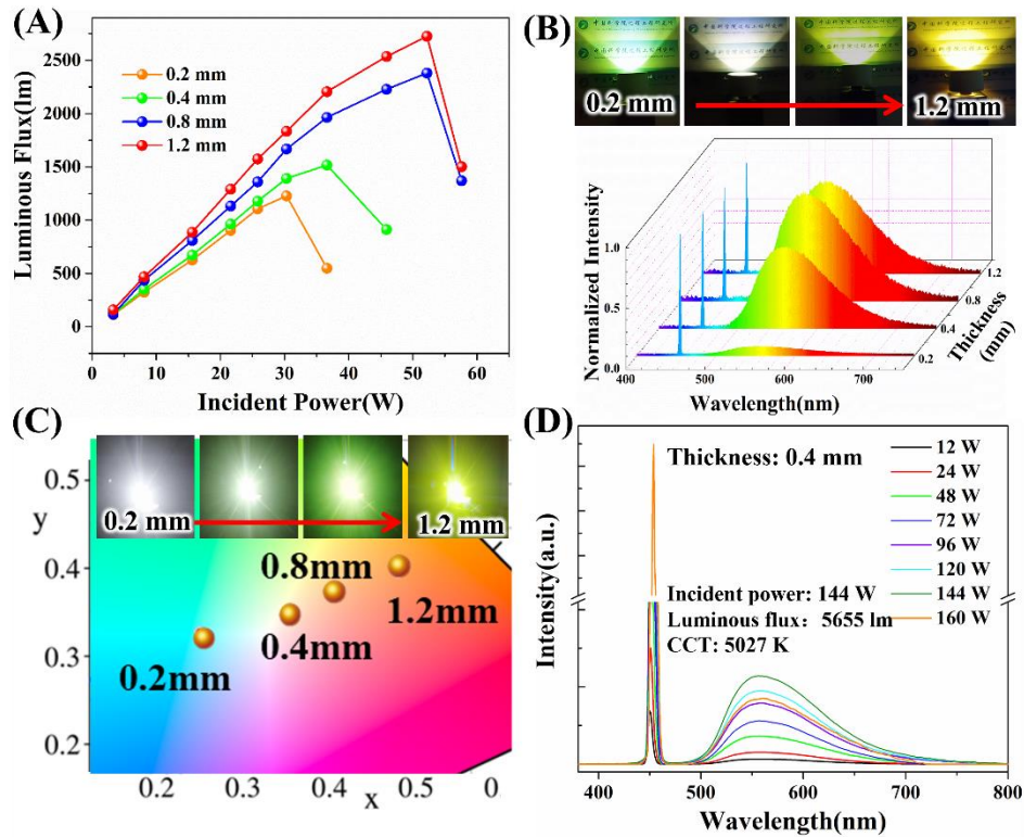
Figure 5. Optical performances of BP-LMAS:0.3% Ce 3+ transparent ceramics for LDs-driven lighting.
