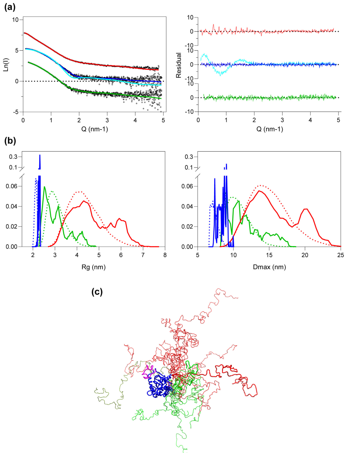
Figure 5. Flexibility modelling of the different entities (a) . Fit (left panel) and residual (right panel) obtained with corresponding experimental data (in black) for Knr4 ΔC (green), Knr4 ΔNΔC (blue) and Knr4 (red). The fit and residual with the crystallographic model without modelling of the missing residues are depicted in cyan. (b) . Histograms of the distribution of R_g and D_{max} values of the different entities obtained respectively from the ensemble selected by EOM (solid line) and the pool (dotted line). (c) . The hybrid model showing the most likely conformations aligned via their SD domain with the Knr4 ΔNΔC (SD) structure after modelling of the missing residues in blue, the N- and C-terminal domains in green and red respectively and the DL loop in magenta. The most populated conformation (21%) is represented by a thick line.
