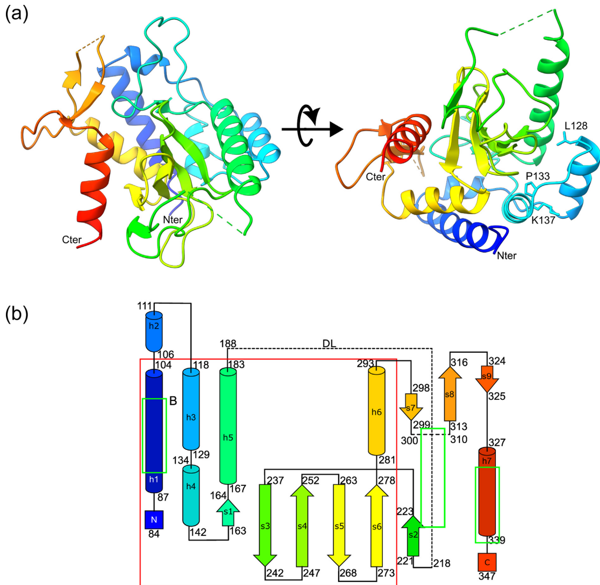
Figure 3. (a). Schematic representation of the structure of the ordered core of Knr4 SD. The structure is represented as a rainbow-colored ribbon, starting from blue for the N-terminal and ending in red for the C-terminal. Stretches of disordered residues with no associated electron density are represented with a discontinuous line. Conserved residues are depicted as sticks and labelled. (b). Topology of Knr4. \alpha -helices are symbolized with cylinders and \beta -strands with arrows. Boundaries of secondary structure elements and of disordered parts of the structure are indicated. Helices are named h1 to h7 and \beta -strands s1 to s9. Colour code is the same as in A. Red box indicates the fold common to the structure of the Smi1/Knr4-like fold. Identified MORFs are indicated with a green box.
