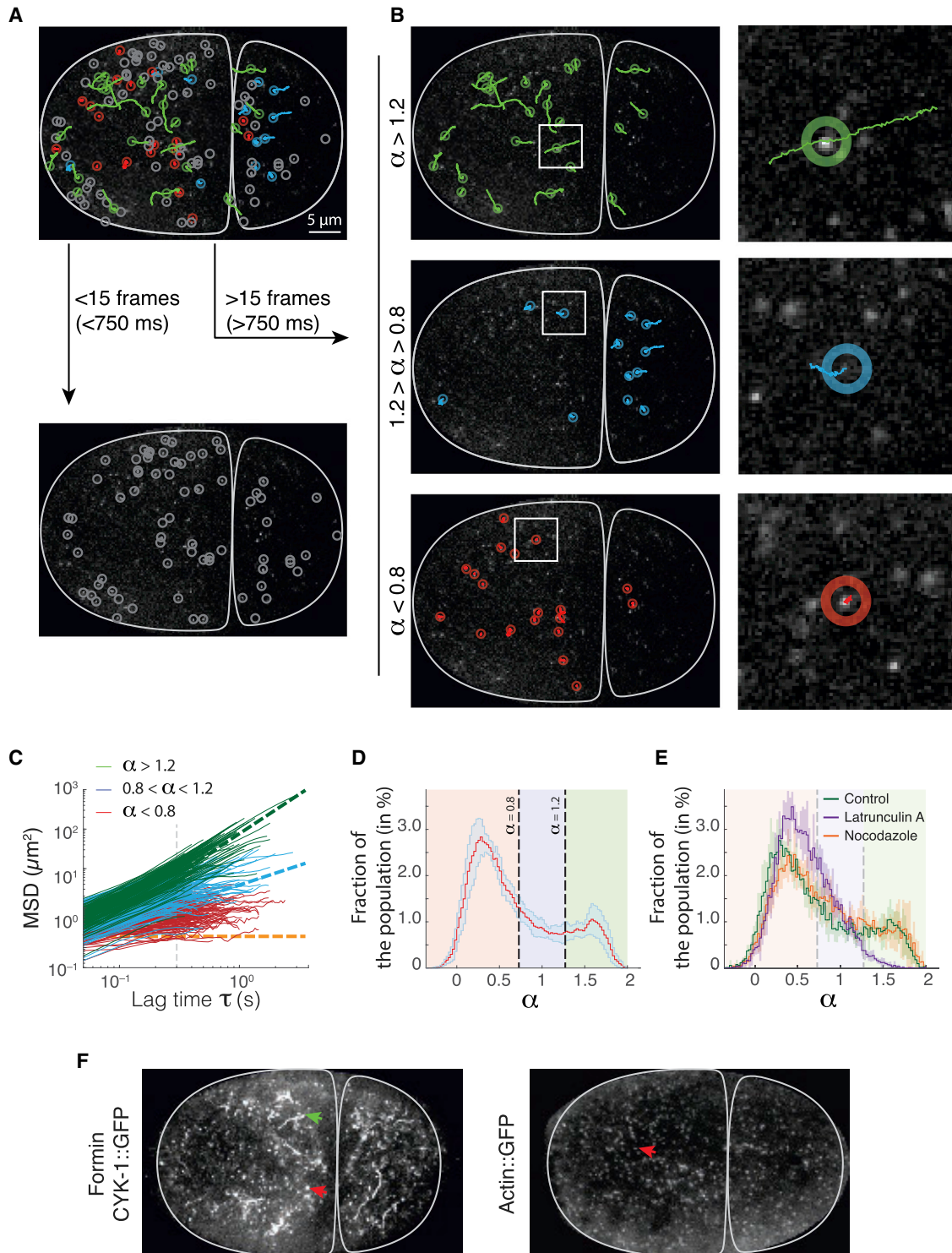
Figure 1. Anomalous diffusion of individual formin molecules identifies a subpopulation of actin-elongating formins
