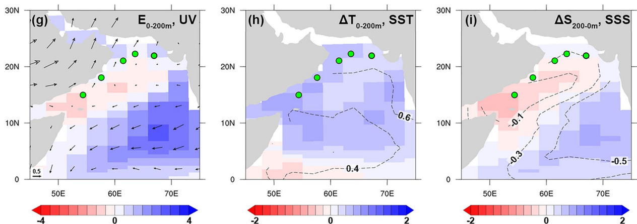
Figure 6. Differences of annual mean E_{0-200\text{ m}} ( 10^6\text{ m}^{-1} ), surface wind (vectors, \text{m s}^{-1} ), \Delta T_{0-200\text{ m}} ( ^{\circ}\text{C} ), and \Delta S_{200-0\text{ m}} (psu) between (a–c) Last Glacial Maximum (LGM; 21.5–21 ka) and late-Holocene (LH; 1–0 ka), between (d–f) HS1 (17–15.5 ka) and BA (14.7–13 ka), and between (g–i) Mid-Holocene (MH; 6.5–6 ka) and LH of TraCE-21.
