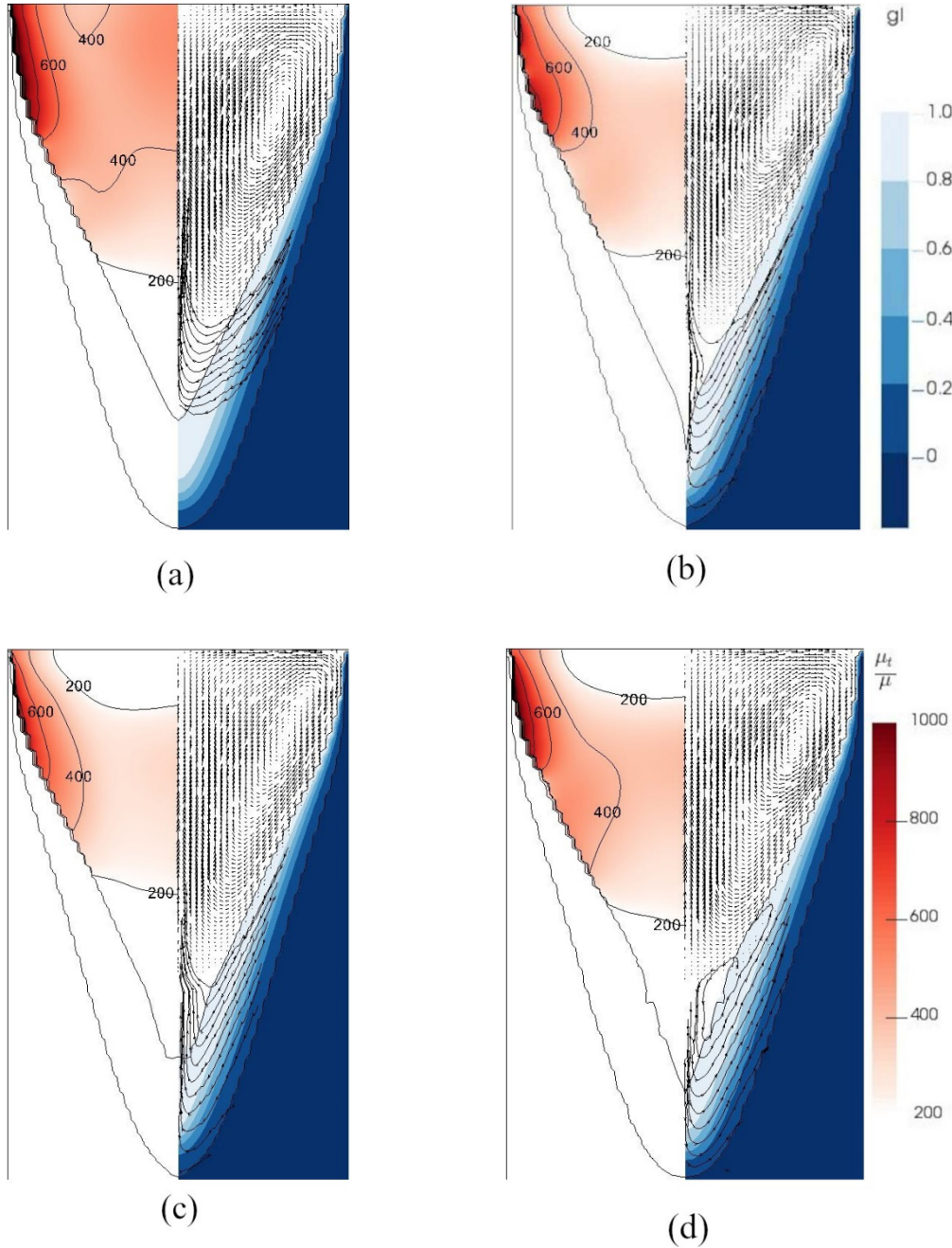
417 Fig. 9. Computed flow in the melt pool and mushy zone at time t_3 (continuous stirring, high 418 azimuthal velocity). Left side is the turbulence intensity and right side is the mean flow
