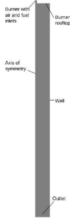
Figure 5: The simplified geometry of the 2D axisymmetric computational domain of the pilot-scale reactor
