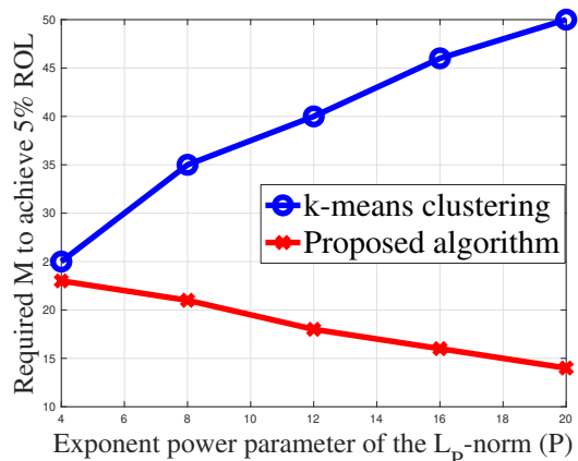
Fig. 3. Required number of cells ( M ) against the exponent power parameter of the L_P -norm ( P ) for the k -means and proposed algorithm. Proposed goal-oriented approach could largely reduce the number of cells especially for large exponent power.
