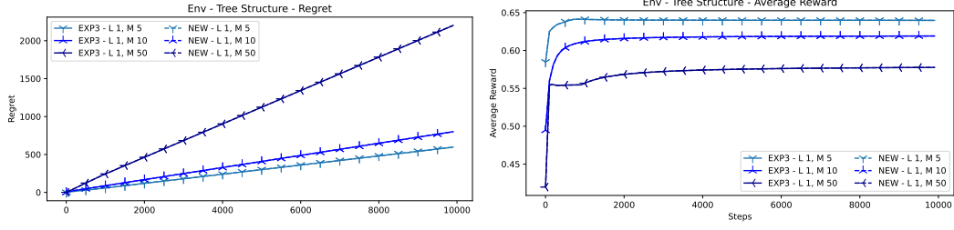
Figure 11: Regret and Average Reward of NEW and EXP3 on the synthetic environment where L = 1 .
