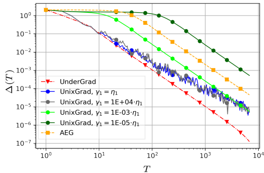
Figure 2: Convergence of UNDERGRAD and UNIXGRAD in the simplex setup with a perfect SFO. The y -axis corresponds to the differences between the f -value of the relevant point of each algorithm and \min f . The code is available at https://github.com/dongquan-vu/UnDerGrad_Universal_CnvOpt_ICML2022 .
