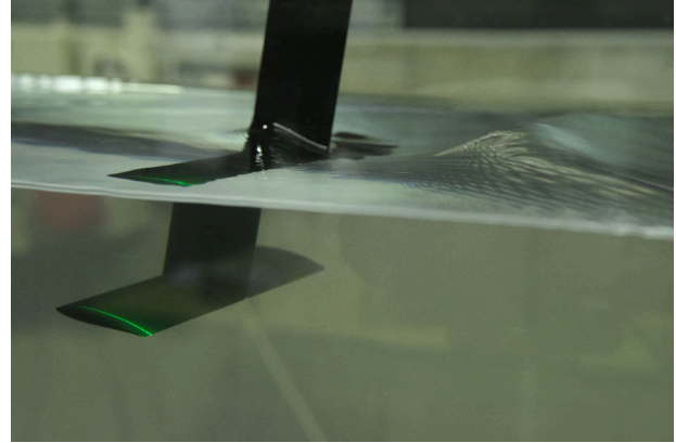
(b) 3D "T-shaped" hydrofoil
