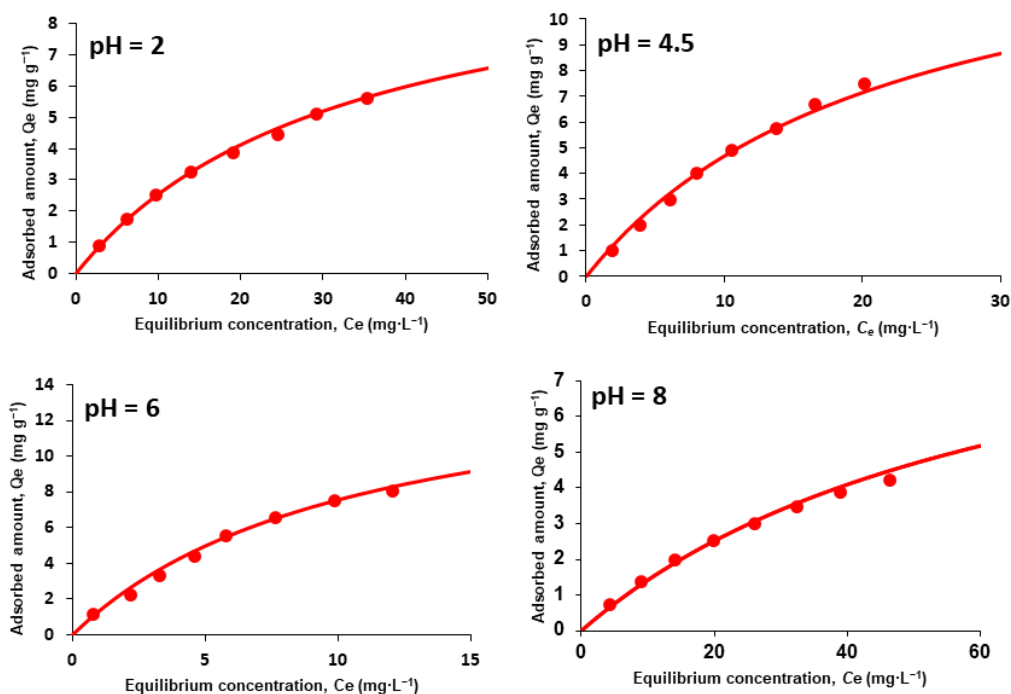
Figure 8. The fit of the bi-Langmuir model to adsorption isotherms of OTC onto POS-50 at various pH at 298 K.
