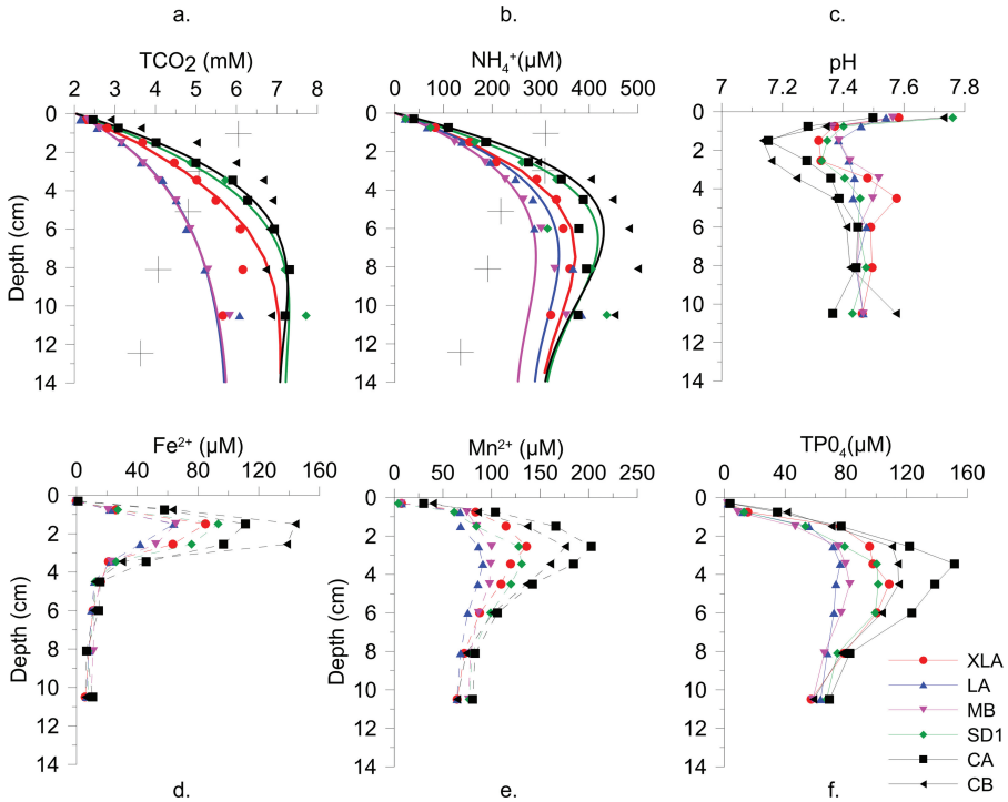
Figure 5. Vertical pore water profiles. (a) \text{TCO}_2 and (b) \text{NH}_4^+ pore water profiles at t = 0 (solid vertical bars) and after \sim 4 weeks in the experimental aquaria (symbol plotted at midpoint of sample depth interval). Transient nonlocal transport–reaction model profile fits are shown as solid lines for CA, S, M, L, and XL tanks. There was a \Delta t relative to initial profiles for CA (26 d), S (27 d), M (27 d), L (29 d), XL (27 d), and CB (32 d). 1-D profiles of reactive solutes distribution at the end of the experiment: (c) pH, (d) \text{Fe}^{2+} , (e) \text{Mn}^{2+} , (f) \text{TPO}_4 . The dashed curves are plotted to aid viewing of distributions.
