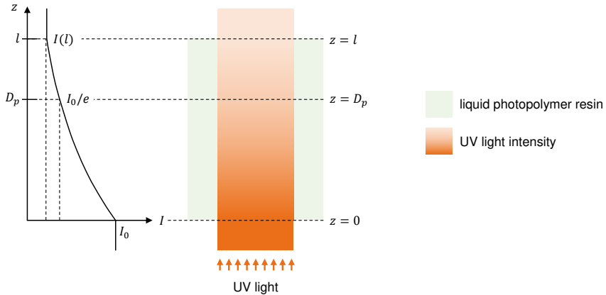
Fig. 3 Beer-Lambert attenuation of UV light intensity with respect to the travelled path in the liquid resin medium ( I_0 : incident light intensity, D_p : penetration depth at which the light intensity drops to e^{-1} , l : thickness of photopolymer liquid resin in order of 10-100 micrometers).
