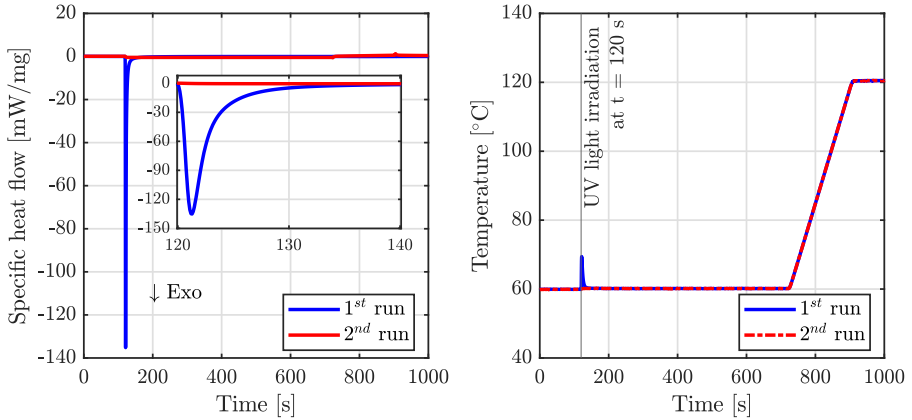
Fig. 9 Photo-DSC measurement for the determination of the total specific heat of reaction h_{tot} . Left: Specific heat flow measurements under the combination of isothermal and non-isothermal conditions with UV light irradiation. Right: Temperature profiles of the measurements.
