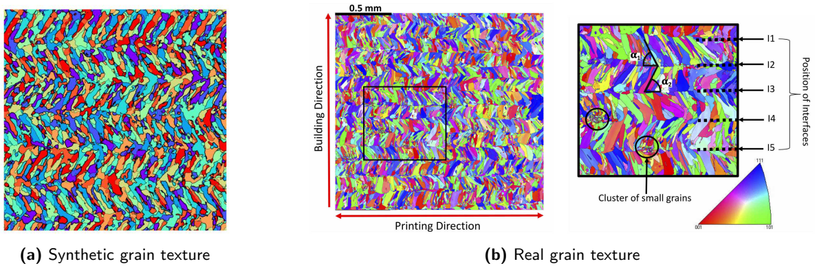
Figure 15: (a) Example of a synthetic multi-phase sample imitating polycrystalline grain texture in a manufactured material (not calibrated design parameters, 10 phases). (b) Electron Backscatter Diffraction of a specimen from bidirectionally-printed single-track thickness 316L stainless steel wall built by directed energy deposition (taken from [7]), and a zoom showing the interfaces between layers, cluster of small grains at interfaces and the morphological grain angles for both direction of printing.
