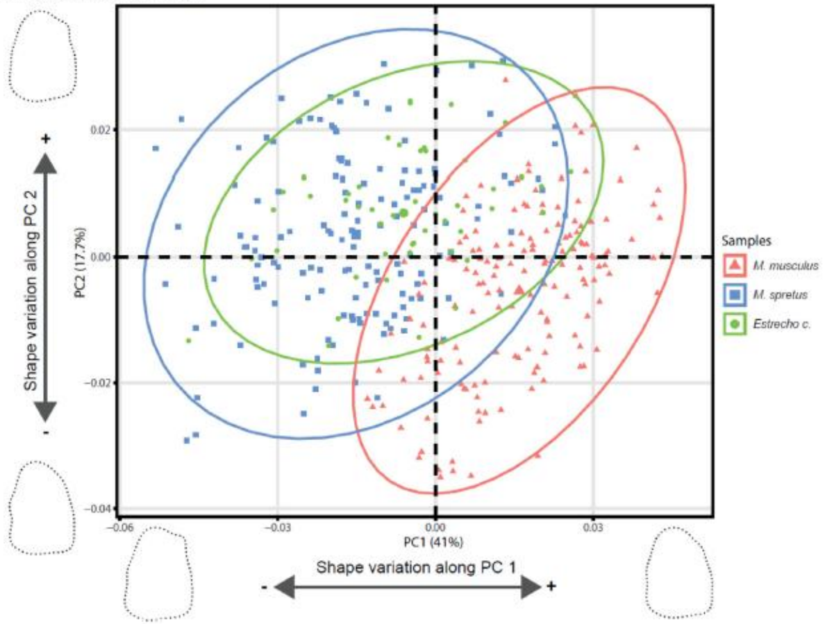
Principal Component Analysis
