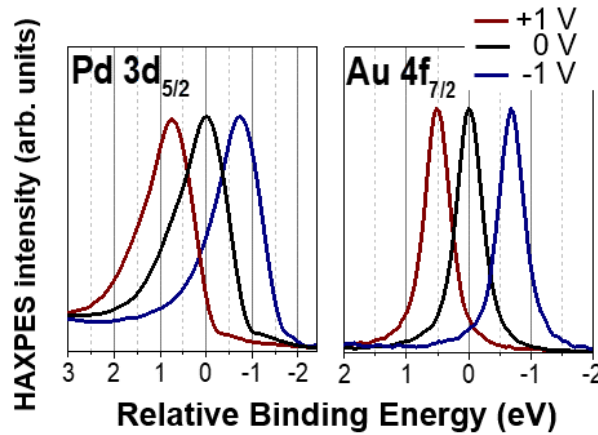
Figure 3 HAXPES shift of Pd 3d 5/2 and Au 4f 7/2 for the M/LaMnO 3+δ stacks (M=Au, Pd) for applied voltages of 0V and +/- 1V.
