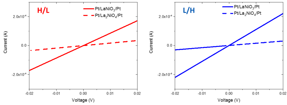
Figure S.4: I(V) curves measured between two Pt contacts placed either on the top \text{La}_2\text{NiO}_4 and on the bottom \text{LaNiO}_3 layers for the two cases: H/L and L/H bilayers (left and right, respectively). Regardless the deposition conditions, high or low p\text{O}_2 , the curves show a linear dependence indicating an ohmic behaviour of Pt/ \text{La}_2\text{NiO}_4 and Pt/ \text{LaNiO}_3 junction. Note that the corresponding resistances are about 100 \Omega and 500 \Omega , for \text{LaNiO}_3 and \text{La}_2\text{NiO}_4 , respectively. These values are much lower than those of the Pt/ \text{LaNiO}_3/\text{La}_2\text{NiO}_4/\text{Pt} bilayers (in Fig. S5) indicating the main contribution to the resistance of the bilayers does not correspond to the regions in contact with Pt.
