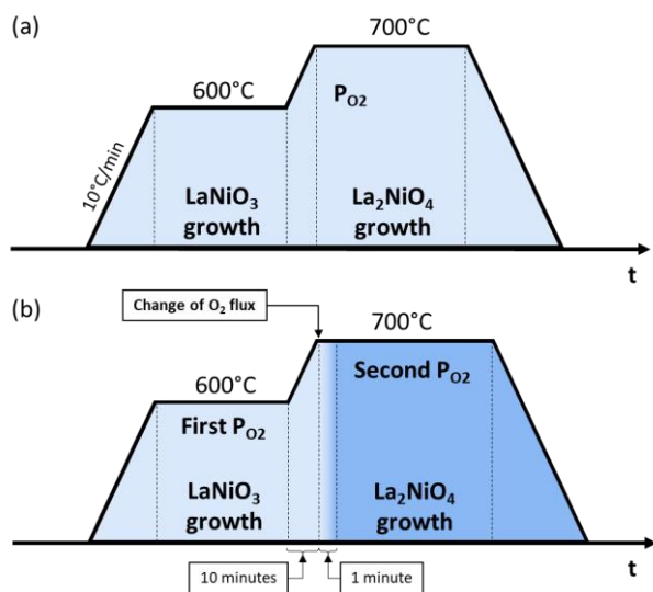
Figure S.1.: Scheme of the growth conditions depicting the deposition temperature profile and oxygen pressure during growth of (a) L/L and H/H samples, (b) L/H and H/L samples. Note that for the second layer deposition the pO 2 conditions are only established once the corresponding temperature is attained.
