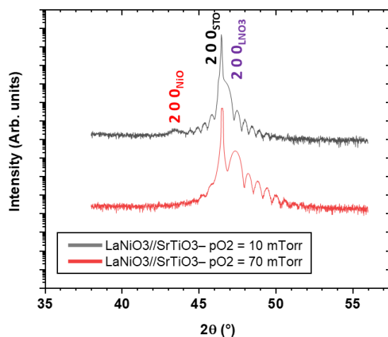
Figure S.2: High resolution XRD scans of \text{LaNiO}_3 single layers ( \sim 20\text{nm} thick) deposited at T=600^\circ\text{C} on \text{SrTiO}_3 under different p\text{O}_2 (70mTorr and 10mTorr). 200_{\text{LaNiO}_3} and 200_{\text{SrTiO}_3} peaks can be observed along with corresponding thickness fringes. The \text{LaNiO}_3 film deposited at low p\text{O}_2 shows a weak peak at 2\theta \sim 43^\circ close to that of the 006 reflection of c_{\perp}\text{-La}_2\text{NiO}_4 or 200 of \text{NiO} , which could correspond to an incipient decomposition of \text{LaNiO}_3 .
