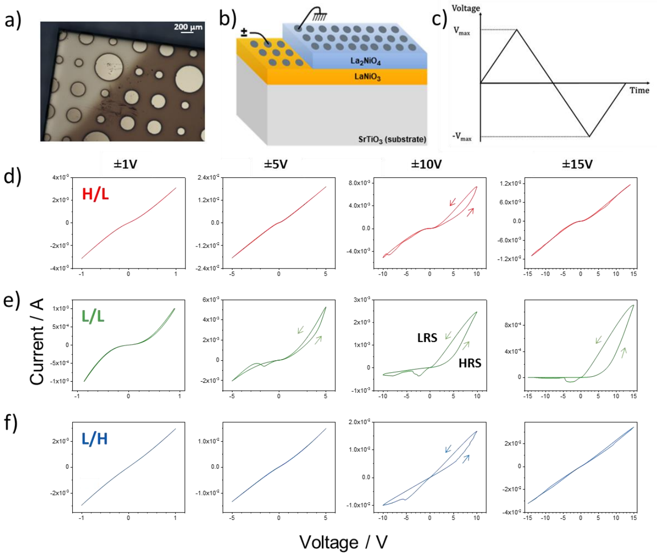
Figure 3. a) Optical Image of the top surface of the Pt/LaNO 3 /La 2 NiO 4 /Pt sample showing the circular Pt electrodes. b) Schematic of the measuring configuration from grounded top Pt electrode on the La 2 NiO 4 layer to biased Pt electrode on the LaNiO 3 bottom layer. c) Applied triangular voltage sweeps. d) to f) Evolution of the I(V) characteristics of the H/L, L/L and L/H bilayers, respectively, when increasing the maximum voltage from left to right ( \pm 1 V, \pm 5 V, \pm 10 V and \pm 15 V). The L/L sample shows clear analog-type switching characteristics. (Arrows indicate the direction of the voltage sweep)
