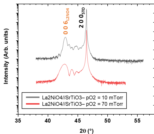
Figure S.3: High resolution XRD scans of \text{La}_2\text{NiO}_4 single layers deposited on \text{SrTiO}_3 under two different p\text{O}_2 (70mTorr and 10mTorr). 006_{\text{La}_2\text{NiO}_4} and 200_{\text{SrTiO}_3} reflections can be observed. In both cases the film grows with c_{\perp}\text{-La}_2\text{NiO}_4 orientation.
