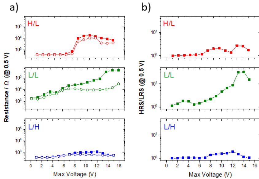
Figure S.5 Left: HRS (filled symbols) and LRS (empty symbols), measured at V=0.5 \text{ V} , for the three bilayers as a function of the maximum voltage amplitude. Right: Evolution of the HRS/LRS ratio (measured at V=0.5 \text{ V} ) as a function of the maximum voltage amplitude.
