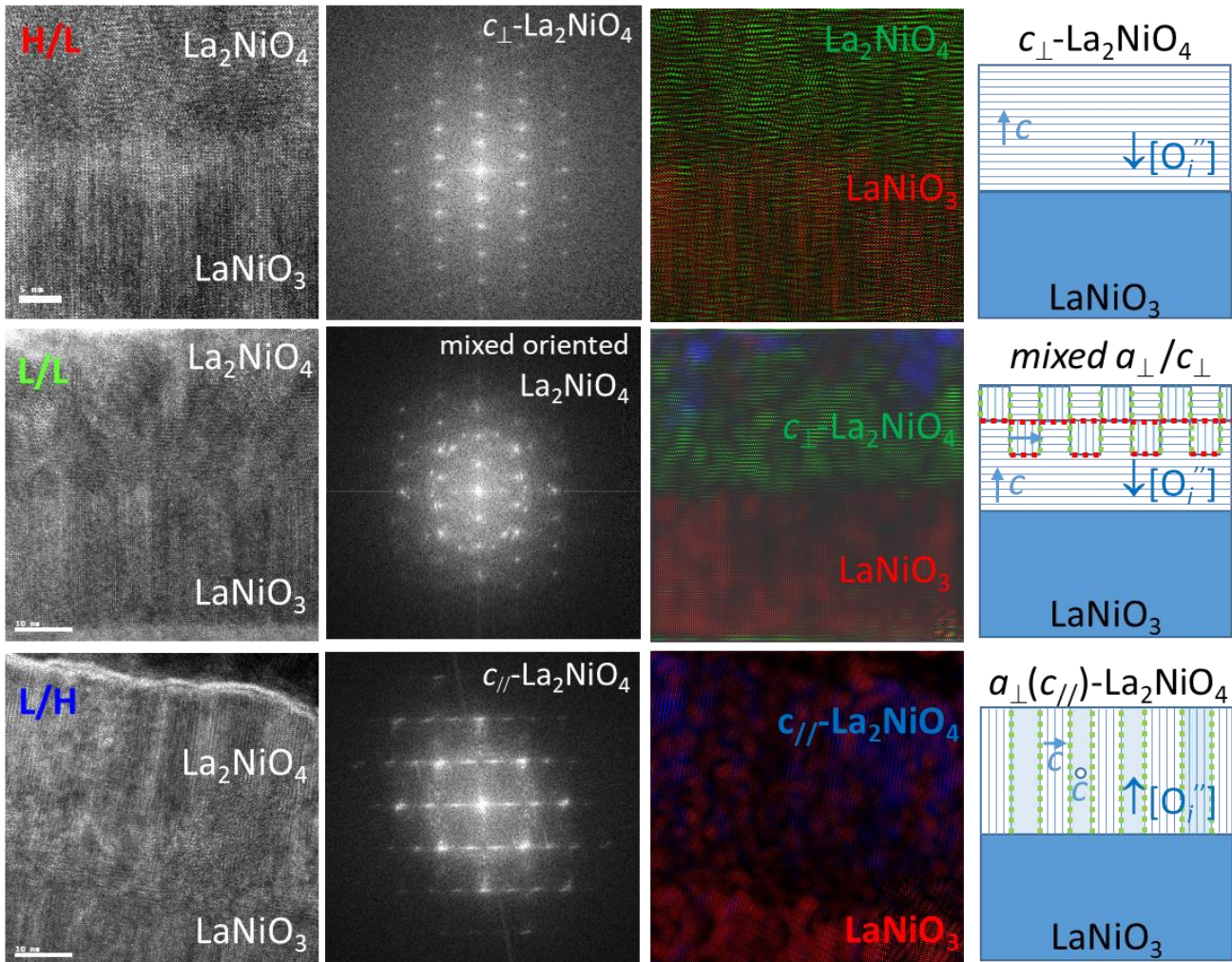
Fig. 2. HRTEM images (left column) of cross sections of the different bilayers from top to bottom: H/L, L/L and L/H \text{LaNiO}_3/\text{La}_2\text{NiO}_4 bilayers, as well as corresponding FFT patterns of the \text{La}_2\text{NiO}_4 layer (second column). The third column shows colour-filtered images for the selected spots in the FFT corresponding to cubic perovskite (red), c_{\perp} -Ruddlesden Popper (RP) (green), a_{\perp} -RP (blue). The column on the right shows a schematic of the film's microstructure and domain orientation (the c -axis is indicated with blue arrows) for the three types of samples, showing the formation of boundaries between a_{\perp} - and c_{\perp} -domains: perpendicular (marked in red colour) and parallel (green) to the vertical axis. It also shows the high concentration or low concentration of oxygen interstitials ( \text{O}'' ) in the initial state depending on the deposition conditions.
