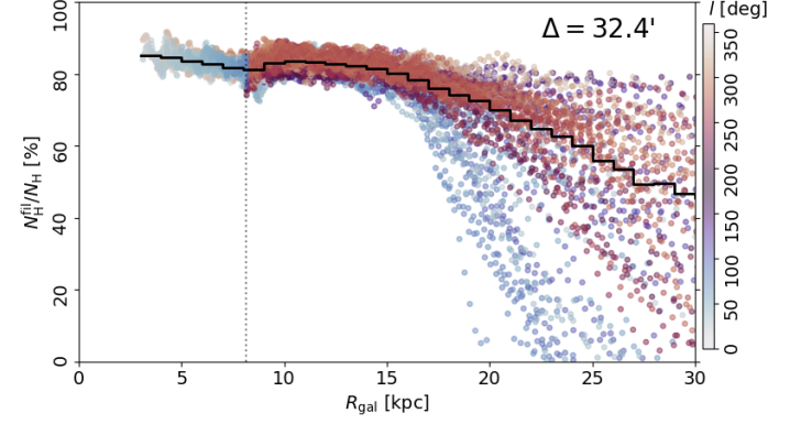
Fig. A.8: Same as Fig. 4, but for 32'4 and 48'6 FWHM derivative kernels, shown in the top and the bottom panels, respectively.
