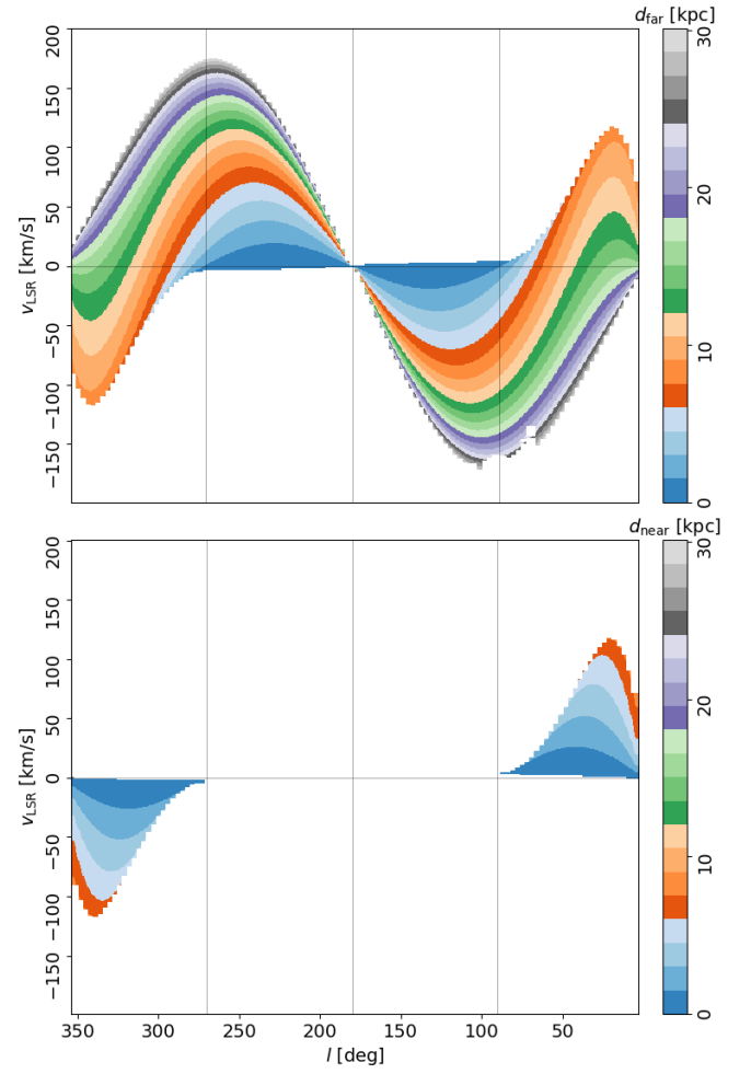
Fig. B.1: Near and far kinematic distances assigned to the 3^\circ \times 20^\circ \times 1.29 \text{ km s}^{-1} tiles used to construct the lv -diagrams in Fig. 1. These results correspond to the solutions of Eq. B.3 using the rotation curve presented in Reid et al. (2019).
