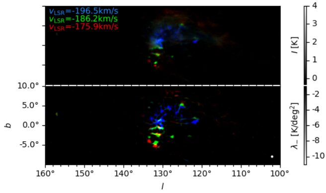
Fig. D.1: Atomic hydrogen (HI) emission (top) and filamentary structures identified using the Hessian matrix method (bottom) toward the HVC complex H.
