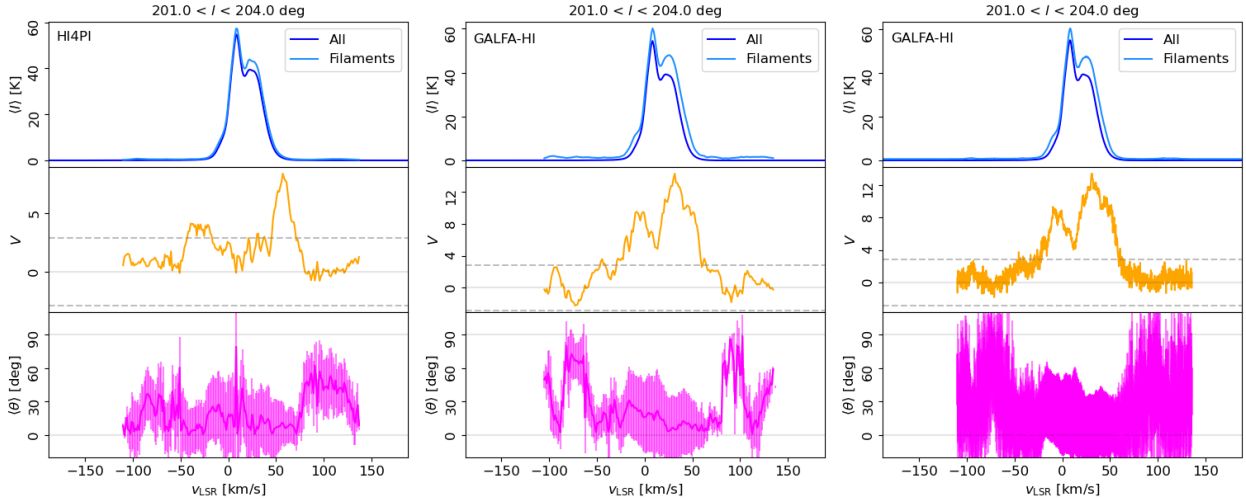
Fig. 16. Mean intensity ( \langle I \rangle , top ), projected Rayleigh statistic ( V , middle ), and mean orientation angle of the filaments ( \langle \theta \rangle , bottom ) for the tiles centered on l = 202.5 in the HI4PI and GALFA-HI. The left panel corresponds to the HI4PI observations analysis with a 18'' FWHM kernel for a 1.29\text{-km s}^{-1} velocity resolution. The center and right panels correspond to the GALFA-HI observations analysis with a 5'' FWHM kernel for 1.29\text{-km s}^{-1} and 0.184\text{-km s}^{-1} velocity resolutions, respectively.
