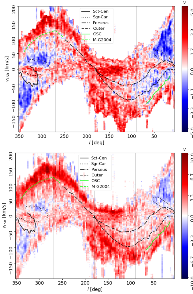
Fig. A.12: Same as Fig. A.10, but for \lambda_- < 0 (top) and a tile-dependent \lambda_- -threshold (bottom).
