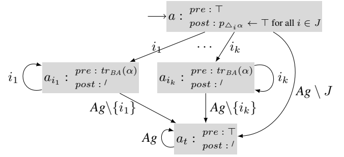
Figure 4: Action model \mathcal{A}_{+J\alpha}^{intr} that simulates adding \alpha in bases of agents in J = \{i_1, \dots, i_k\} in the introspective variant.
