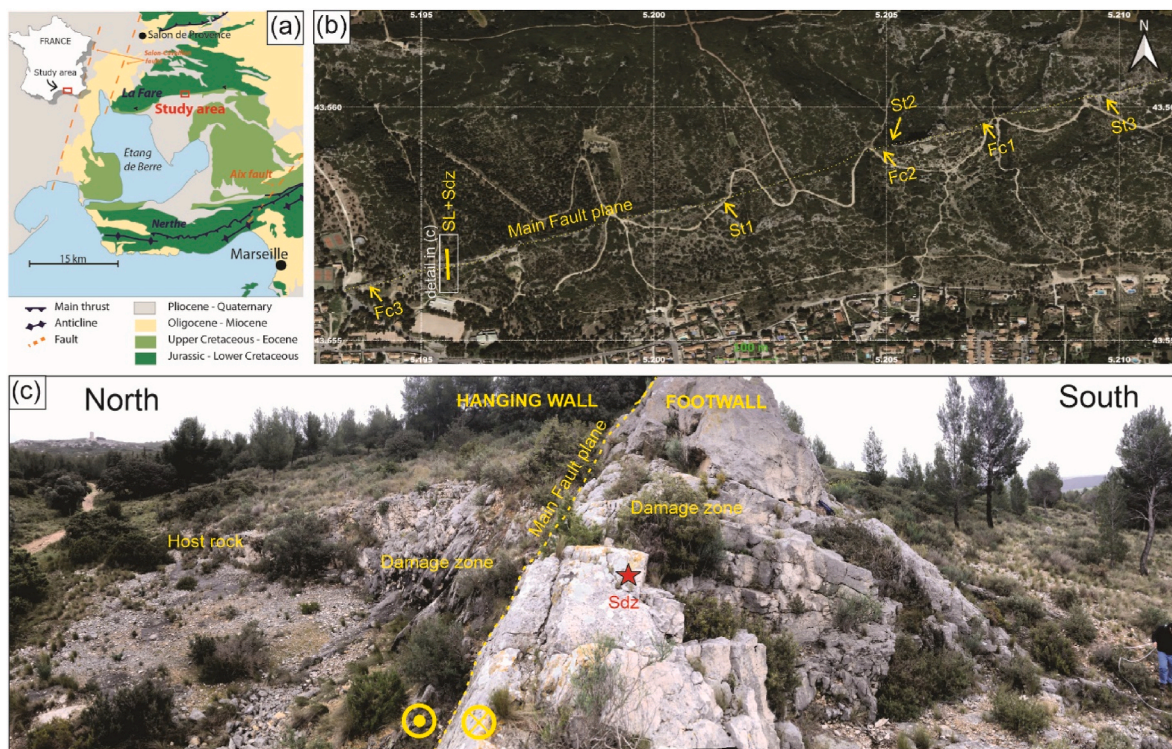
Fig. 1. Location and field photographs of the studied outcrop, near La Fare-les-Oliviers city, Southeast France ( 43^{\circ} 33' 23.947''N ; 5^{\circ} 11' 43.595''E ). (a) Simplified geological map (modified from Aubert et al., 2019). (b) Aerial image of the Castellás fault with sample and scanline locations. Average trend of the scanline is N15°E. (SL – Scanline trace, Fc – Fault core sample, St – Sampling transect). (c) Panoramic view of the outcrop showing the location of the main fault plane, damage zone and host rock, where the scanline was acquired (Sdz – Damage zone sample). Hanging wall on north side and footwall on south side.
