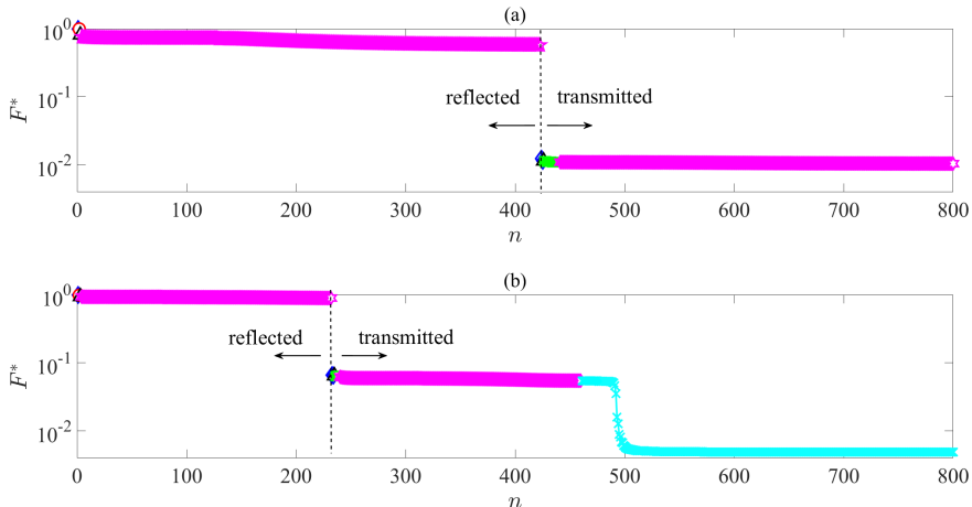
FIGURE 8. Evolution of the normalised objective function as a function of the number of modes: (a) vortex sheet, (b) finite-thickness model. Markers and colours are the same as those used to identify the modes in the eigenspectra in figures 3 and 5 for the VS and figures 4 and 6 for the F-T model.
