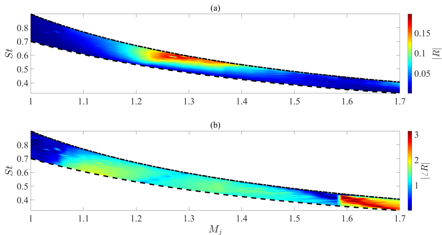
FIGURE 15. Evolution of the reflection coefficient as a function of Strouhal and jet Mach numbers for the finite-thickness model. Dashed and dash-dotted lines refer to the branch- and saddle-point locations, respectively. (a) amplitude, (b) phase.
