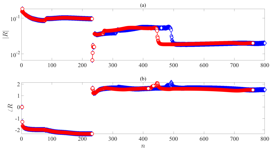
FIGURE 18. Evolution of the reflection coefficient as a function of the number of modes considered using the finite-thickness model: blue \diamond refer to results obtained including near-sonic, downstream-travelling acoustic modes, red \circ refer to results obtained artificially removing near-sonic acoustic modes ( k_{a_{MAX}}^+ = 3.2 ). (a) amplitude, (b) phase.
