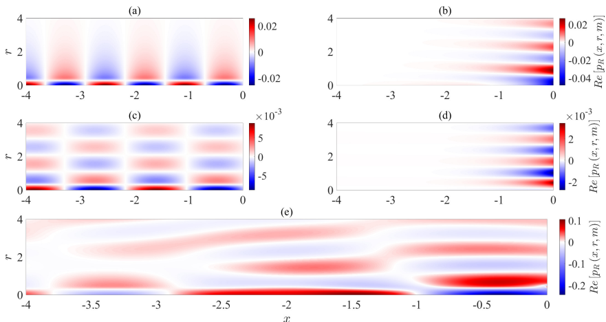
FIGURE 12. Reconstruction of the reflected fields in the x - r plane for a shock discontinuity located at x = 0 : (a) k_p^- mode with n_r = 2 , (b) k_p^- mode with n_r = 1 , (c) propagative k_a^- wave, (d) evanescent k_a^- wave, (e) total field.
