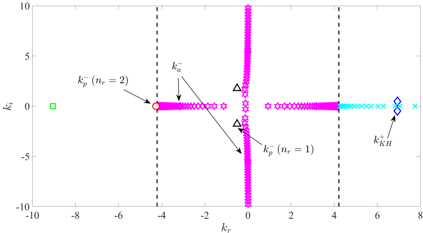
FIGURE 4. Eigenspectrum upstream of the shock obtained using the finite-thickness model for azimuthal mode m = 0 , T \approx 0.81 , M_{j1} = 1.1 and \omega \in \mathcal{R} . Markers and colours to identify the modes are the same used in figure 3 in the case of the VS. The modes that are only supported by the finite-thickness model, that is the k_{cr}^+ modes, are here indicated by cyan \times . Dashed lines refer to the sonic speed \pm c_\infty . Incident and reflected waves are indicated with arrows and labelled.
