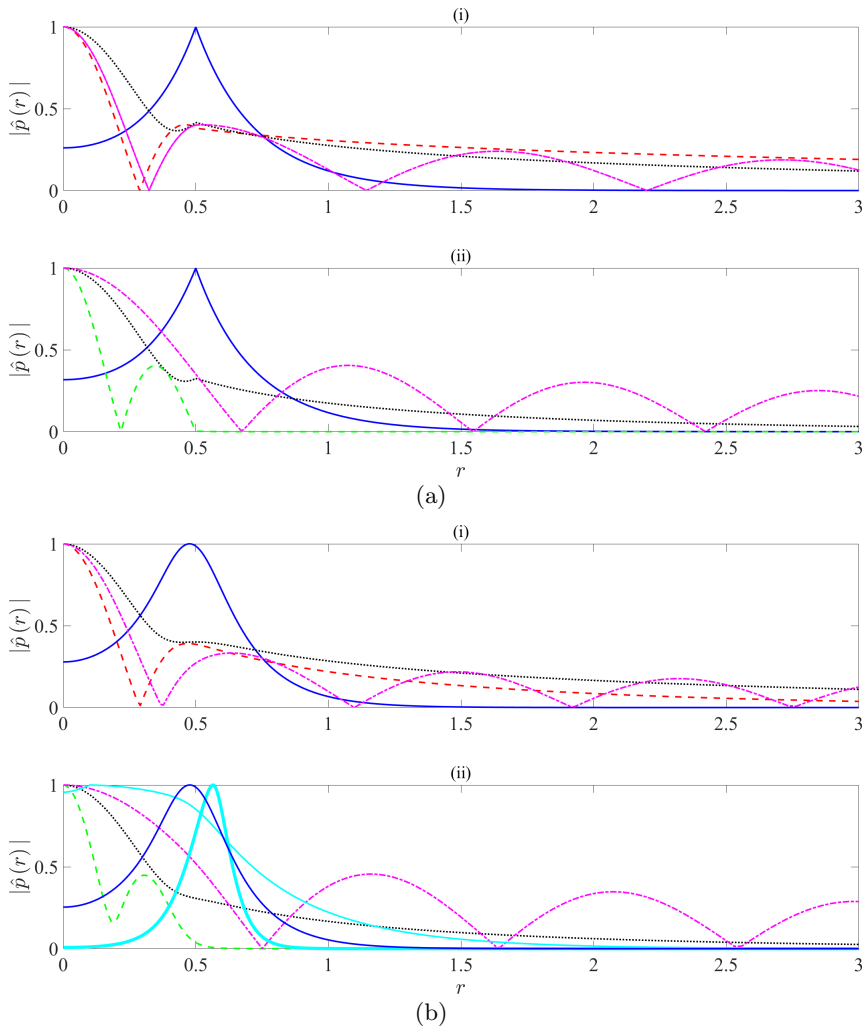
FIGURE 7. Pressure eigenfunctions for m = 0 and St = 0.68 computed using (a) the vortex-sheet model and (b) the finite-thickness model. The colours are the same as those used in figures 3, 4, 5 and 6 to identify the different mode families upstream and downstream of the shock, respectively. (i) incident and reflected waves upstream of the shock for M_j = 1.1 and T \approx 0.81 : solid blue line refers to the incident k_{KH}^+ wave, dashed red line to the propagative k_p^- wave with n_r = 2 , dotted black line to the evanescent k_p^- mode with n_r = 1 , dash-dotted magenta line to the propagative k_a^- wave. (ii) transmitted waves downstream of the shock for M_{j2} = 0.91 and T \approx 0.85 : solid blue line refers to the transmitted k_{KH}^+ mode, dotted black line to the evanescent k_p^+ with n_r = 1 , dashed green line to the evanescent k_p^+ with n_r = 2 , dash-dotted magenta line to the propagative k_a^+ wave, solid and bold cyan lines to k_{cr}^+ modes.
