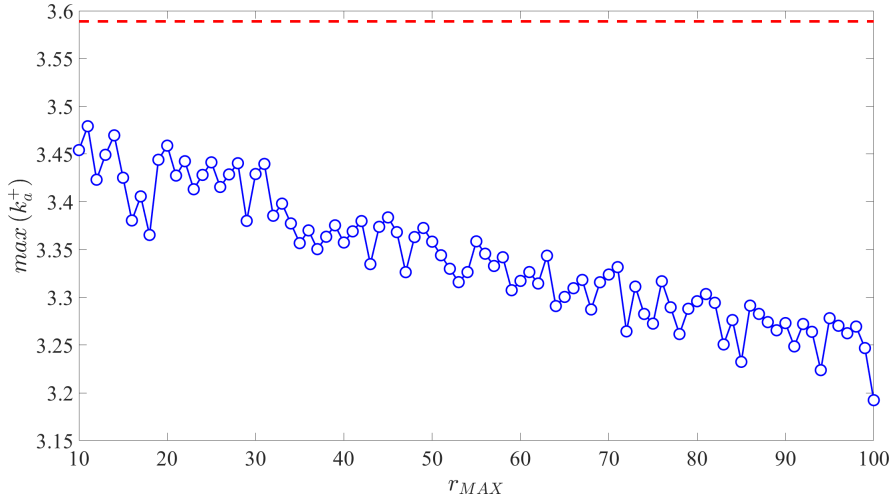
FIGURE 17. Maximum eigenvalue of the propagative, downstream-travelling acoustic branch as a function of the wall distance using the confined vortex-sheet model. Flow conditions are the same reported in figure 5 downstream of the shock. Blue \circ represent the eigenvalue, dashed red line the position of the sonic line.
