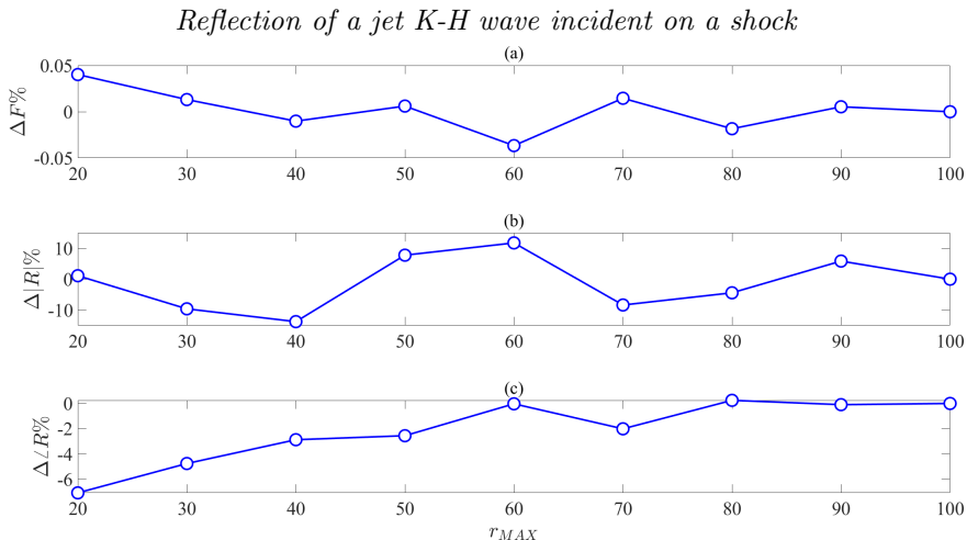
FIGURE 19. Variation of the objective function, amplitude and phase of the reflection coefficient as a function of the wall distance using the confined vortex-sheet model. Variations are relative to the results obtained for r_{MAX} = 100 presented throughout the manuscript. (a) objective function, (b) reflection coefficient amplitude, (c) reflection coefficient phase.
