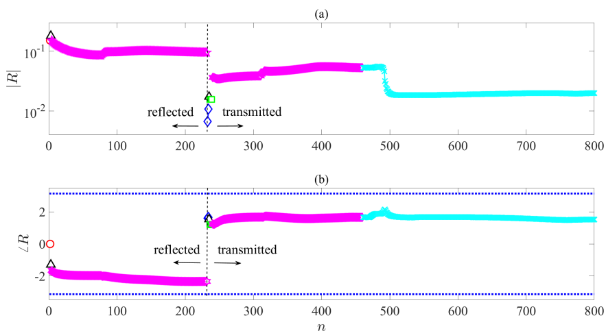
FIGURE 10. Evolution of the amplitude and phase of the reflection coefficient computed using the finite-thickness model as a function of the number of modes considered. Markers and colours are the same as those used in figures 4 and 6 to identify the mode families. (a) amplitude, (b) phase. Blue dotted lines indicate \pm\pi in the phase plot.
