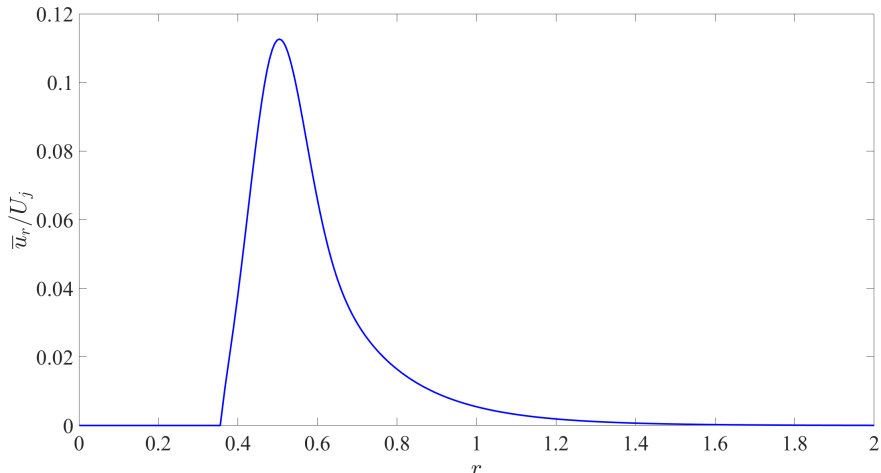
FIGURE 16. Mean radial velocity profile along the radial direction downstream of the shock for M_{j1} and M_{j2} equal to 1.1 and 0.91, respectively.
