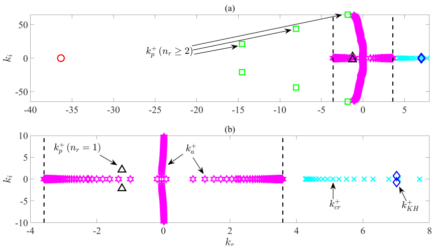
FIGURE 6. Eigenspectrum downstream of the shock obtained using the finite-thickness model for \omega \in \mathcal{R} , azimuthal mode m = 0 , T \approx 0.85 and M_{j2} = 0.91 (which corresponds to M_{a2} = 0.84 ): (a) global view, (b) zoom around the origin. Markers and colours are the same used in figure 5 to identify the modes in the case of the VS. The modes that are only supported by the finite-thickness model, that is the k_{cr}^+ modes, are here indicated by cyan \times . Dashed lines refer to the sonic speed \pm c_\infty . Transmitted waves are indicated with arrows and labelled.
