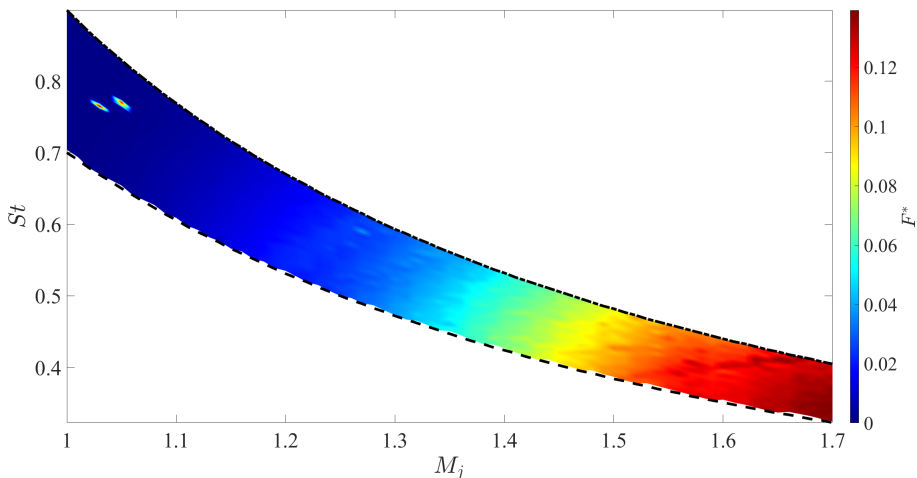
FIGURE 14. Normalised error objective function as a function of Strouhal and jet Mach numbers for the finite-thickness model. Dashed and dash-dotted lines refer to the branch- and saddle-point locations, respectively.
