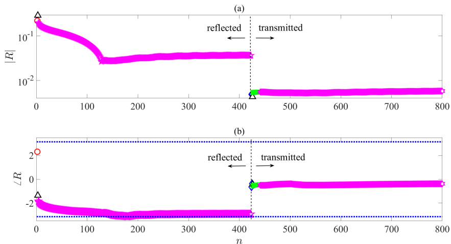
FIGURE 9. Evolution of the reflection coefficient computed using the VS as a function of the modes considered in the calculation (markers and colours are the same as those used to identify the modes in the eigenspectra in figures 3 and 5): (a) amplitude, (b) phase. Blue dotted lines indicate \pm\pi in the phase plot.
