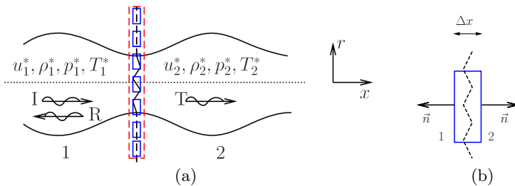
FIGURE 1. Schematic representation of the jet model: (a) sketch of the shock-containing jet, (b) control volume representation with identification of the normal to the inlet and outlet surfaces.
