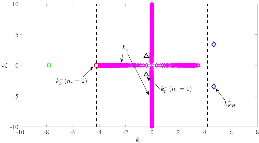
FIGURE 3. Eigenspectrum upstream of the shock obtained using the vortex-sheet model for azimuthal mode m = 0 , T \approx 0.81 , M_{j1} = 1.1 and \omega \in \mathcal{R} . Blue \diamond represent k_{KH}^+ and k_{KH}^{*+} waves, red \circ represents propagative k_p^- mode with n_r = 2 , black \triangle represent evanescent k_p^\pm modes with n_r = 1 , green \square represent k_p^+ modes with n_r \geq 2 , magenta * represent k_a^\pm waves. Dashed lines refer to the sonic speed \pm c_\infty . Incident and reflected waves are indicated with arrows and labelled.
