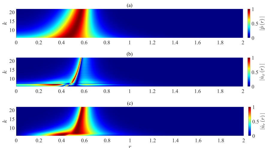
FIGURE 11. Normalised eigenfunctions of k_{cr}^+ modes computed using the finite-thickness model as a function of wavenumber k and radial distance r : (a) pressure, (b) axial velocity, (c) radial velocity.
