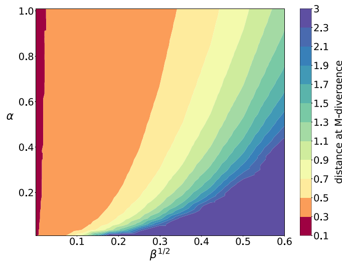
Figure 5. Distance of singularity at divergence time as function of \alpha and \beta^{1/2} : because the initial condition is now u(x,0) = 0 and u_t(x,0) = +\exp(-30x^2) , all divergences seem to be of M-type (see theorem B.1, which only asserts divergence in finite type, but the proof suggests divergence at near the advancing front). Note that for all \alpha and \beta > 10^{-6} considered in this graph, the distance of the singularity from x = 0 at blowup is at least 0.1795 (in the interval [-\pi, \pi] ). For this initial condition and the \alpha, \beta , considered, blowup always happens before the wave hits the boundary.
