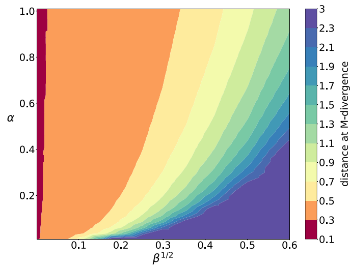
Figure 5. Distance of singularity at divergence time as function of \alpha and \beta^{1/2} : because the initial condition is now u(x,0) = 0 and u_t(x,0) = +\exp(-30x^2) , all divergences seem to be of M-type (see theorem B.1, which only asserts divergence in finite type, but the proof suggests divergence at near the advancing front). Note that for all \alpha and \beta > 10^{-6} considered in this graph, the distance of the singularity from x=0 at blowup is at least 0.1795 (in the interval [-\pi, \pi] ). For this initial condition and the \alpha, \beta , considered, blowup always happens before the wave hits the boundary.
