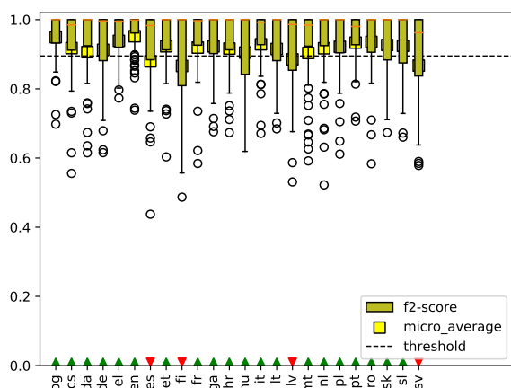
Figure 5: Distribution of F2-score of <*-PERSON> detection across documents for each language (translated documents).
