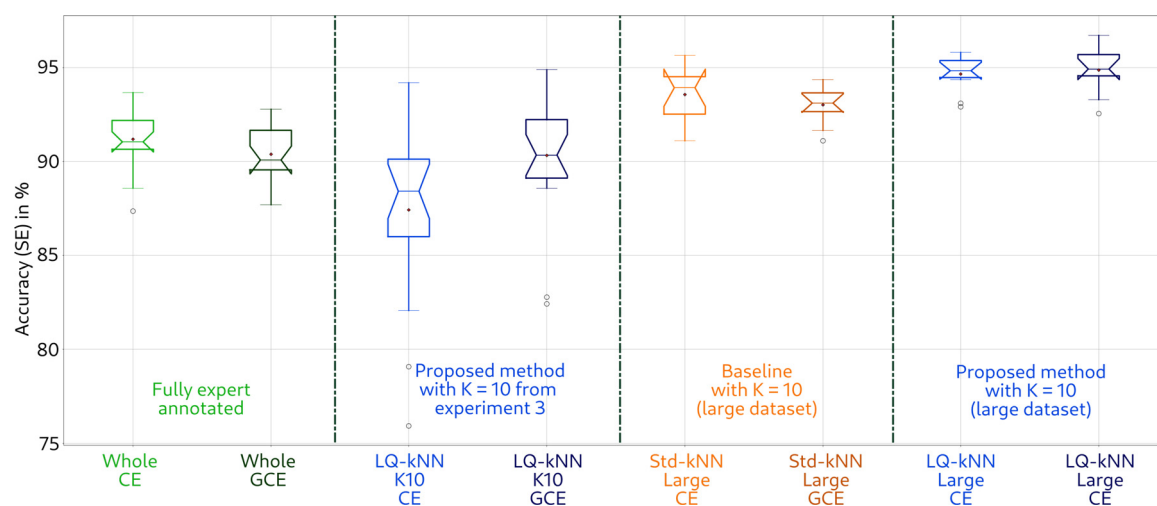
Fig. 13. Experiment 4: Solid emboli test accuracies as comparisons using semi-automatically labeled HITS datasets with unknown label noise. We propagate the labels from 1545 manually labeled samples to part of the remaining 66 947 unlabeled samples. Based on the label propagation method used, we obtain datasets with different numbers of samples (however, the classes are always balanced): 15 198 samples when using the baseline Std-KNN with K = 10 , and 16 515 when using LQ-KNN with K = 10 and \tau = 0.1 .
