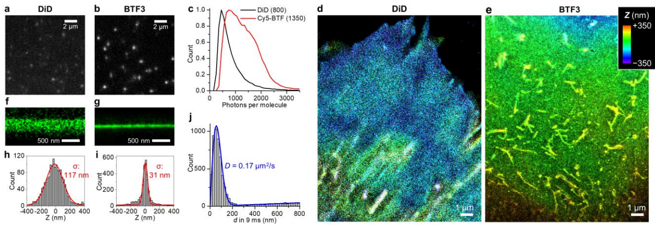
Figure 6. Single-molecule and 3D-PAINT characterizations of BTF3 in comparison to the Cy5-based DiD dye. (a,b) Representative frames of single-molecule images of DiD (a) and BTF3 (b) in the plasma membrane of a live COS-7 cell, under continuous 647 nm illumination at \sim 1 kW/cm 2 and recorded at 110 frames per second with an \sim 9 ms exposure time. (c) Distributions of the single-molecule photon counts recorded in each frame for the two dyes. (d) Example 3D-PAINT images of DiD (d) and BTF3 (e) of the plasma membrane of live COS-7 cells. (f,g) Typical vertical cross-sections of the 3D-PAINT data of the two dyes at the plasma membrane. (h,i) Spread in Z values for local flat regions. Gaussian fits (red curves) give standard deviations of 117 and 31 nm, respectively. (j) Typical distributions of single-molecule displacements in successive frames for BTF3 . Blue curve: fits to our model, 48 yielding a diffusion coefficient D of 0.17 \mu\text{m}^2/\text{s} .
