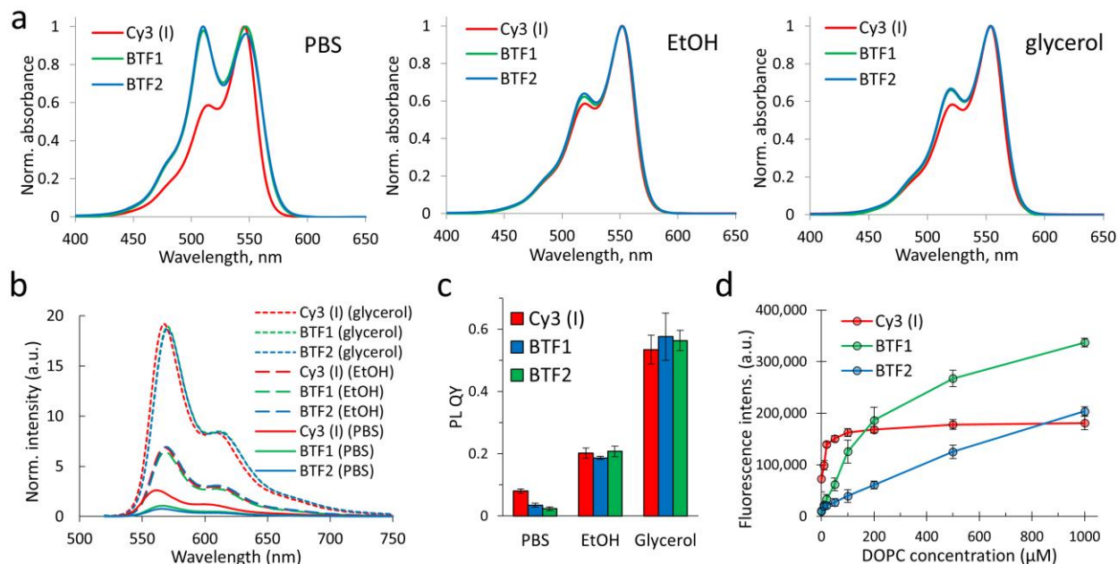
Figure 2. Photophysical characterization of the probes BTF1 , BTF2 and monomeric Cy3 ( I ). (a) Normalized absorption spectra measured at 4, 2 and 2 μM, correspondingly. (b) Fluorescence spectra of BTF1 , BTF2 and Cy3 ( I ) at 0.2 μM, 0.2 μM and 0.4 μM, respectively, measured in PBS, ethanol, and glycerol. (c) Fluorescence quantum yields. (d) Titration of BTF1 and BTF2 (100 nM) and Cy3 ( I ) (200 nM) with increasing concentrations of DOPC lipid vesicles (phosphate buffer, pH 7.4): peak fluorescence intensity, excitation at 510 nm.
