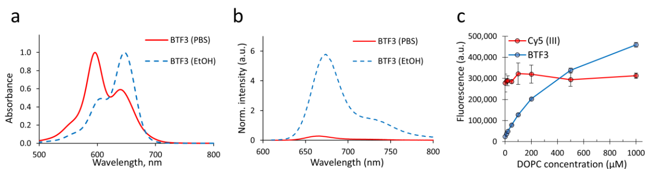
Figure 3. Absorption (a) and fluorescence (b) spectra of BTF3 in different media measured at 0.2 \mu\text{M} concentration. Excitation wavelength: 600 nm. Fluorescence spectra are normalized with respect to absorptivity at 600 nm. (c) Titration of BTF3 (100 nM) and Cy5 (III) (200 nM) with increasing concentrations of DOPC lipid vesicles (phosphate buffer, pH 7.4): peak fluorescence intensity, excitation at 600 nm.
