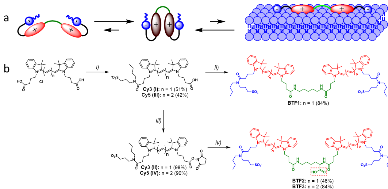
Figure 1. (a) Concept of switchable cyanine-based dimeric probe that lights up after reversible binding to biomembranes. (b) Synthetic scheme for Cy3-based BTF1 , BTF2 and Cy5-based BTF3 probes. Red rectangle highlights polar carboxylic group. Conditions: i ) 3-(butylamino)propane-1-
