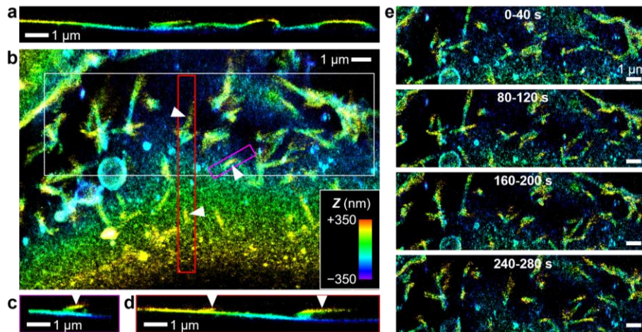
Figure 5. 3D-PAINT with BTF2 unveils rich 3D structures and dynamics of the plasma membrane in living cells. The sample was continuously illuminated with 560 nm at \sim 1 kW/cm 2 in the wide field and recorded at 110 frames per second with an \sim 9 ms exposure time. (a) Vertical cross-sectional view of the 3D-PAINT data of the plasma membrane of a COS-7 cell with undulating membrane heights. (b) In-plane view of another cell, highlighting numerous nanoscale tubules. (c,d) Vertical cross-sectional views along the magenta (c) and red (d) boxes in (b), showing tubules protruding away from the cell surface (arrowheads). Note that in the vertical cross-sectional views shown in (a,c,d), the vertical dimension corresponds to depth into the sample. (e) Time-divided 3D-PAINT data in 40 s brackets at 4 time points, for the white box in (b). See Movie S2 for the full sequence. For all images, color presents depth ( Z ) according to the color scale in (b).
