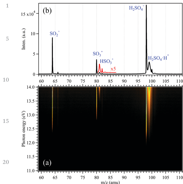
Fig. 1 (a) Synchrotron photoionization mass spectra matrix in the 11–14 eV energy range and (b) their integrated mass spectrum, together with 5 times magnified data in red.
