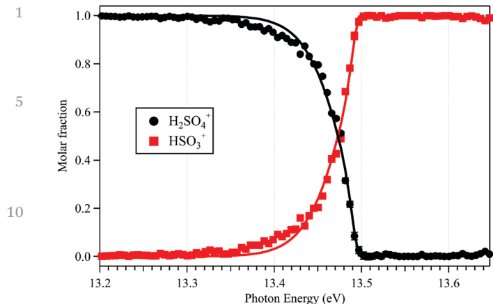
Fig. 4 Breakdown diagram of the \text{H}_2\text{SO}_4^+ parent ion ( m/z = 98 ) and \text{HSO}_3^+ fragment ion ( m/z = 81 ). Solid circles represent the experimental data, while lines correspond to the statistical model (see text for details).
