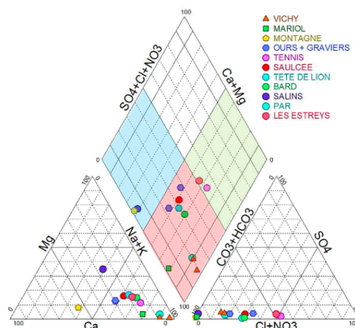
Figure 2: Piper diagram illustrating the variety of chemical properties observed in the spring waters.
