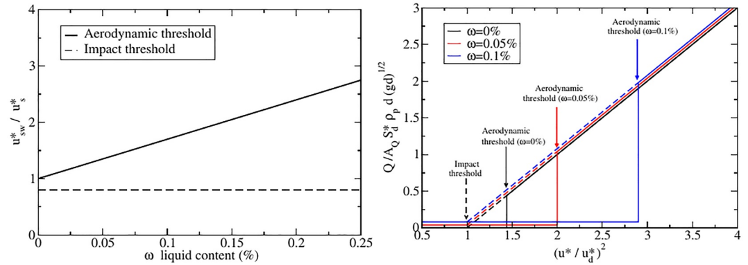
Figure 6. (a) Aerodynamic and Impact thresholds as a function of the liquid content. (b) Conjectured mass transport rate at equilibrium and bi-stable domain for various liquid content: This graph illustrates the increase of the range of the bi-stable domain (i.e., u_d^* < u^* < u_{sw}^* ) with increasing cohesion. Here we conjectured that the mass transport law at equilibrium is unchanged for cohesive granular beds (see Equation 5).
