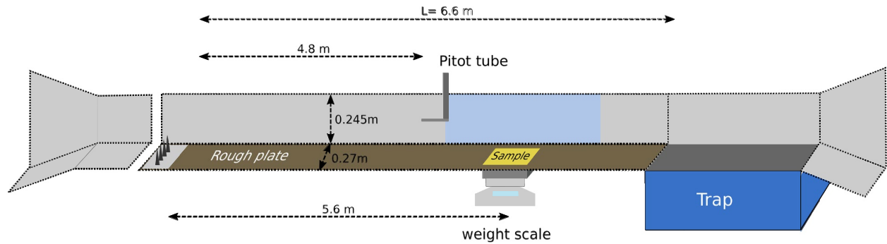
Figure 1. Wind-tunnel facility.
