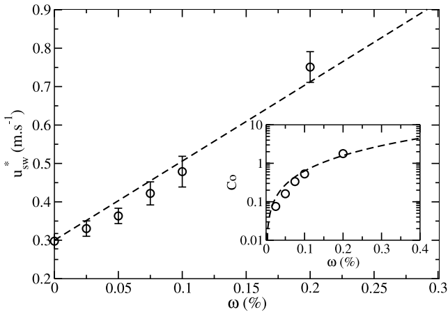
Figure 3. Static threshold u_{sw}^* as a function of the liquid content \omega . The dash line corresponds to a linear fit to the data (see Equation 10). Inset: The cohesion number Co as a function of the liquid content. The cohesion number Co is obtained from Equation 4. The dash line corresponds to the predicted cohesion strength computed from the linear relationship between the threshold friction velocity and the liquid content: Co = (a_{\omega} \omega / 3)(2 + a_{\omega} \omega) .
