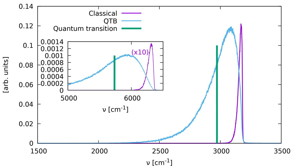
FIGURE 4: C_{vv}(\omega) spectra for the mildly anharmonic Morse potential, for the classical MD simulation (magenta), the QTB (blue) and the first quantum transition between the ground state and first excited state (green). The inset shows show the overtones (the classical spectrum is multiplied by a factor of 10).
