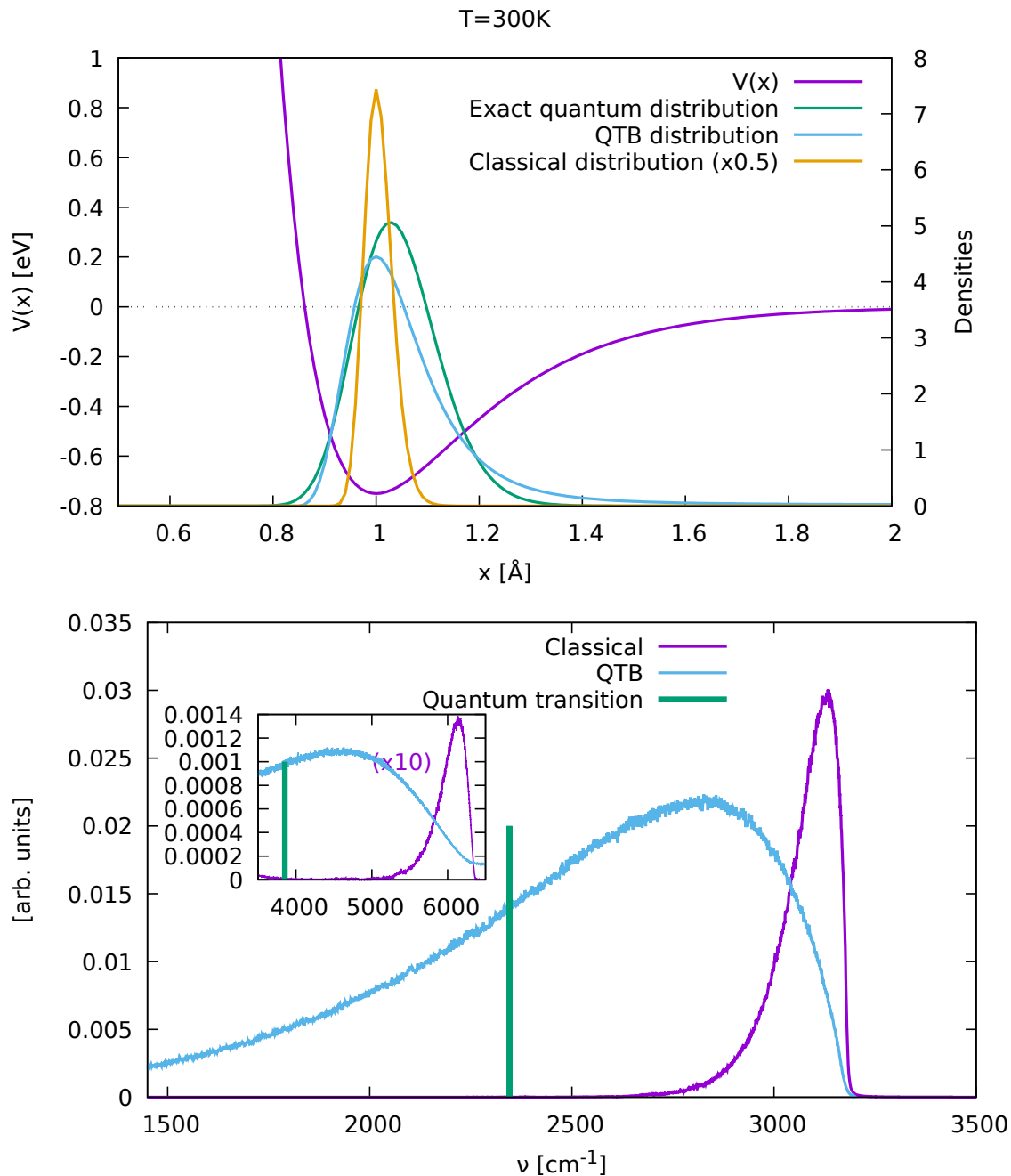
FIGURE 5: Distributions (top) and C_{vv}(\omega) spectra (bottom) for the strongly anharmonic Morse potential, for the classical MD simulation (magenta), the QTB (blue) and the first quantum transition between the ground state and first excited state (green). The inset shows show the overtones Note that the classical spectrum is multiplied by a factor of 10.
