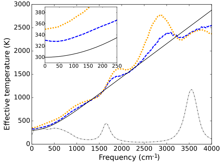
FIGURE 11: Plot of the effective temperature defined by eq. (33) in liquid water at 300 K described with the q-TIP4P/F model and simulated with the QTB method using \gamma = 20 \text{ ps}^{-1} . The blue dashed line corresponds to oxygen (it is average over all O atoms and over all three directions x , y and z ), the dotted orange line to hydrogen, and the black continuous line is the reference k_B^{-1}\theta(\omega, T) that corresponds to the first kind FDT. The simulations were performed using Tinker-HP software [Lagardère et al., 2018] and parameters similar to that in Ref. [Mauger et al., 2021]. The inset represents a zoom on the low-frequency region and the vibrational power spectrum mC_{vv}(\omega) is shown as a dashed-dotted grey line.
