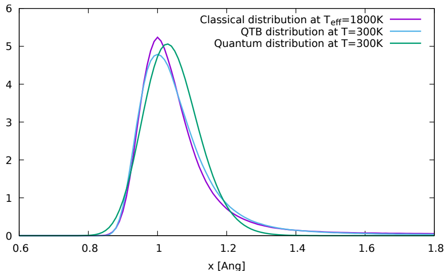
FIGURE 6: Comparison of the particle position distributions for a classical Langevin simulation at the QTB effective temperature T_{\text{eff}} = 1800\text{K} with the corresponding QTB distribution at T = 300\text{K} and the exact quantum distribution at the same temperature.
