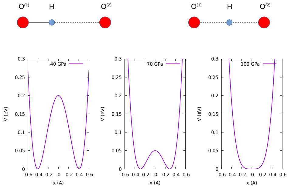
FIGURE 9: The one-dimensional proton effective potential energy V(x; P) for ice under increasing pressure P . The variable x is the difference between the distances from H to its two O neighbors: x = d(\text{O}^{(1)} - \text{H}) - d(\text{O}^{(2)} - \text{H}) . At P = 40 GPa, the proton forms a short covalent bond and a long hydrogen bond (left panel); at P = 100 GPa, according to the classical picture, V(x) shows a single minimum at x = 0 and the two bonds are equivalent (right panel).
