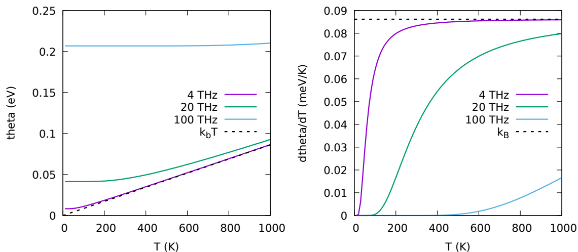
FIGURE 2: Left: \theta(\omega, T) (left panel) and its temperature derivative d\theta(\omega, T)/dT for three representative frequencies \nu = \omega/2\pi . \nu_1 = 4 THz is typical of acoustic modes in crystals; \nu_2 = 20 THz is in the range of optical modes in crystals formed by light mass elements, as well as of OH and CH bending modes; \nu_3 = 100 THz could correspond to C-H and O-H stretching modes. For the latter frequency, one can see that the classical behavior is never reached for T \leq 1000 K.
