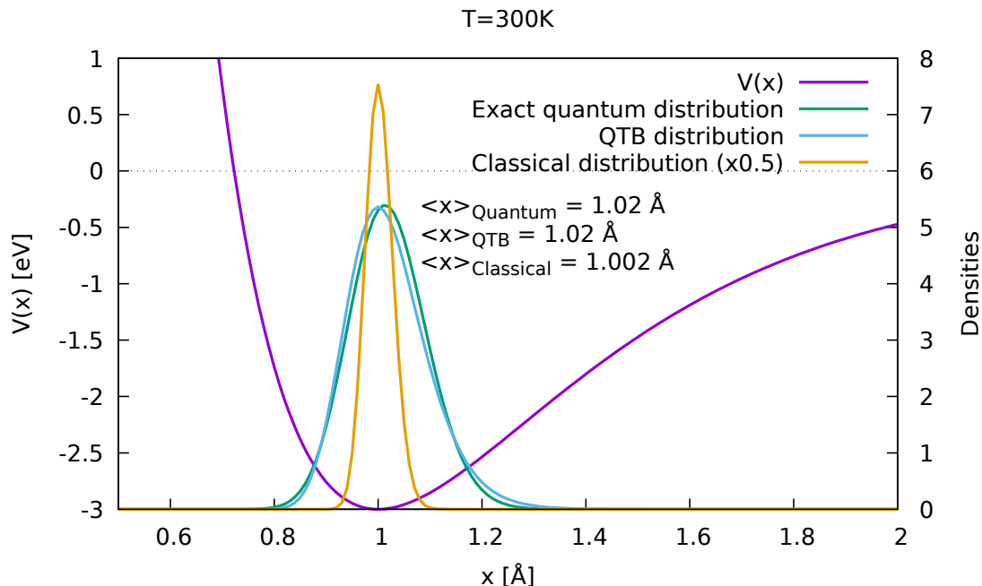
FIGURE 3: A one-dimensional mildly anharmonic Morse potential (magenta, left-hand scale), with the position distributions (right-hand scale) for a classical simulation (yellow), a quantum solution through Schrödinger's equation (green) and the Quantum Thermal Bath (light blue).
