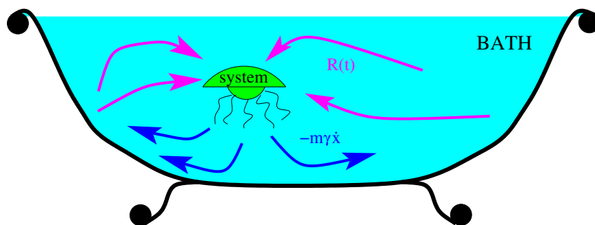
FIGURE 1: The Langevin equation (4) & (5) as a thermal bath in classical molecular dynamics simulations: the random force R(t) (magenta arrows) pumps energy from the bath into the system, while the friction force -m\gamma\dot{x} (blue arrows) extracts energy from the system. The balance between the two produces the correct thermal equilibrium. These forces can be modified to generate generalized baths with different given properties.
