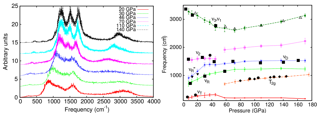
FIGURE 10: Left panel: ice spectra obtained through the Fourier transform of the velocity-velocity autocorrelation function from QTB simulations at several pressures, by using the data from [Bronstein et al., 2014]. Right panel: the peaks extracted from the QTB ice spectra (lines) are compared to the experimental infrared and Raman scattering data (triangles and circles).
