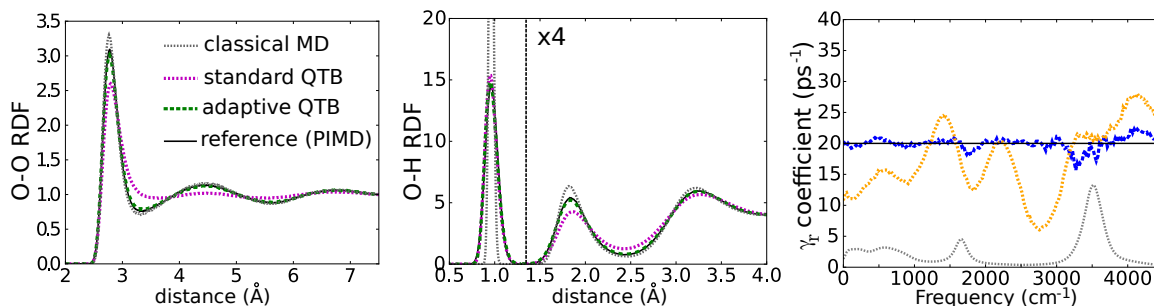
FIGURE 13: Plot of the radial distribution functions in liquid water at 300 K described with the q-TIP4P/F model and simulated with different molecular dynamics methods (left: oxygen-oxygen, middle: oxygen-hydrogen). The friction coefficient used for QTB and adQTB methods is \gamma = 20 \text{ ps}^{-1} , the adapted random force coefficients \gamma_r(\omega) are plotted on the right panel for oxygen (dashed blue) and hydrogen (dotted orange) atoms. The simulations were performed using Tinker-HP software [Lagardère et al., 2018] and parameters similar to that in Ref. [Mauger et al., 2021].
