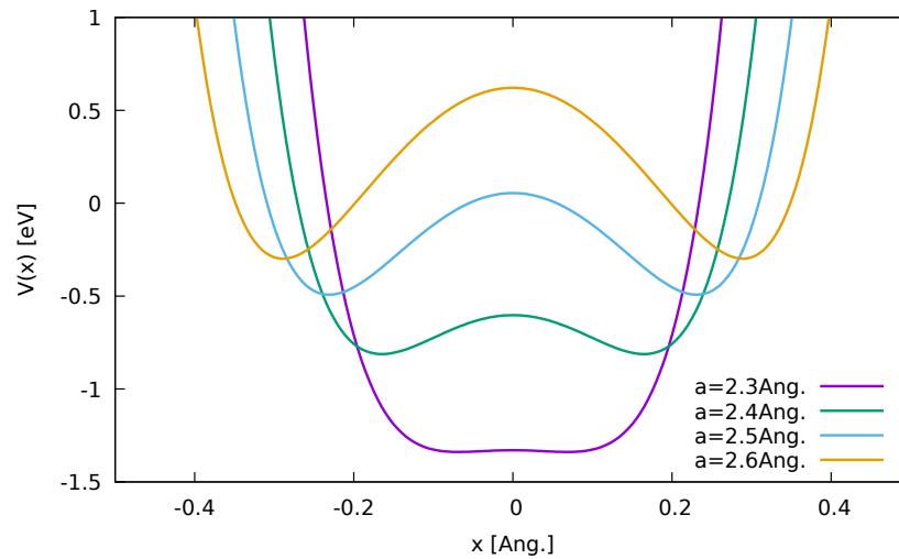
FIGURE 14: Double well potential (equation (41)) for several interatomic distances.
