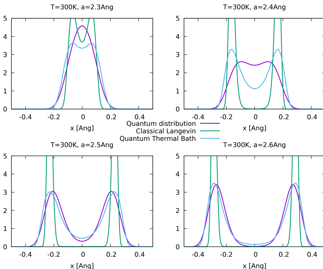
FIGURE 15: Quantum probability distribution (magenta), classical distribution (green) and QTB probability distribution (blue), at T = 300\text{K} for several interatomic distances. The damping coefficient here is \gamma = 0.1\text{THz} . Setting \gamma to 1\text{THz} or 10\text{THz} does not change the resulting probability distributions significantly.
