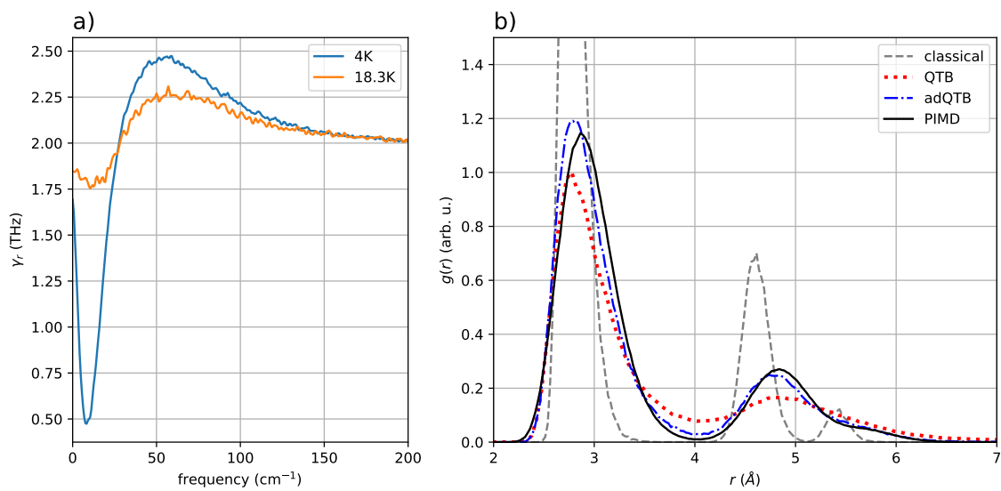
FIGURE 12: a) Adapted \gamma_r(\omega) for the \text{Ne}_{13} clusters of [Mangaud et al., 2019] at 4K (blue) and 18.3K (orange). b) Radial pair distribution function for the QTB (dotted red) and adQTB (dash-dotted blue) compared to classical (dashed grey) and PIMD (solid black) at 4K (results converged using 32 beads). The friction coefficient was set to \gamma = 2 \text{ ps}^{-1} in all simulations.
