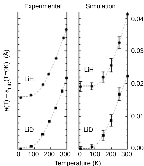
FIGURE 8: Variation of the lattice parameters of cubic LiH and LiD vs. temperature, with respect to the LiD lattice parameter at T = 0 K. Left: experimental; right: QTB simulations.
