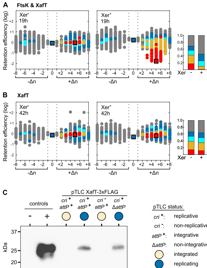
Figure 6. Retention efficiency of the different possible n_8gtg XaFT + mini-TLC \Phi libraries. (A) Retention efficiency from the natural difI locus after growth in LB in conditions of production of XerCD ( Xer^+ ) or not ( Xer^- ). Bar plots show the proportion of n_8gtg motifs belonging to the red, orange, cyan, blue and grey categories within the integrated motifs. Retention efficiencies of the n_{5a_2n_3g} and tagn_8 XaFT + mini-TLC \Phi libraries are shown in Supplementary Figure S6. (B) Excision from the lacZ locus after growth in LB, in conditions of production of XerCD ( Xer^+ ) or not ( Xer^- ). (C) Anti-FLAG immunoblot of XaFT-3xFLAG expression in integrated vs replicative pTLC conditions. The predicted molecular weight of XaFT-3xFLAG C-terminal fusion protein (220 aa) is 25.5 kDa (EMBOSS Pepstats). Immunoblot contains normalized whole-cell samples of V. cholerae strain EPV369 over several plasmid conditions. Negative control is EPV369. Positive control is EPV369 containing an (induced) arabinose-inducible XaFT-3xFLAG expression plasmid. Subsequent lanes contained cell extracts from either integrated or replicative versions of pTLC synthetic phage plasmids. White and blue illustrated colonies indicate samples derived from integrated (into the lacZ-difI reporter cassette) or replicative V. cholerae clones, respectively. cri^- and \Delta attP denote pTLC variants which are unable to replicate, or unable to integrate, respectively. Supplementary Figure S6C contains uncropped source images of the original SDS-PAGE, transfer, and immunoblot.
