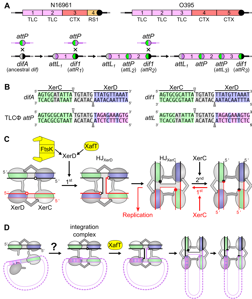
Figure 1. Xer recombination. (A) Schematic representation of the IMEX arrays found on chr1 of a V. cholerae strain from the 7 th (N16961) and the 6 th (O395) pandemics (top) and of the successive integration of TLCΦ leading to the formation of those arrays (bottom). The arrays result from successive lysogenic conversion events, a new dif site being generated on the right side of each newly-integrated IMEX. Pink, red, orange blocks: TLCΦ, CTXΦ and RS1 prophages; Coloured disks: difA (grey/black), TLCΦ attP (green/pink), TLCΦ attL1 (grey/pink), dif1 (green/black) and current dif site of the strains (black disk). Numbers indicate the order of integration of the phage, which can be directly deduced from their position relative to the current dif site. (B) V. cholerae difA and dif1 , TLCΦ attP and attL1 sequences. Green: XerC-binding site; Light grey: central region and non-canonical bp of difA ; Blue: XerD-binding site; Pink: non-canonical bp of attP . The top and bottoms are cleaved by XerC and XerD, respectively. The positions of cleavage are indicated by triangles. (C) Xer recombination pathways. XerC and XerD are shown in light and dark grey, respectively. The central region, XerC and XerD-arms of the recombination sites are shaded in grey, green and blue, respectively. Black arrows: conventional recombination pathway; Red arrows: non-conventional asymmetric recombination pathway. The XerD and XerC cleavage points are depicted by empty and filled disks. (D) TLCΦ integration. Black and pink lines: V. cholerae chr1 and TLCΦ DNA, respectively. Question mark: the low affinity of XerD for the XerD-arm of TLCΦ attP poses questions about the possible formation of integration complexes.
