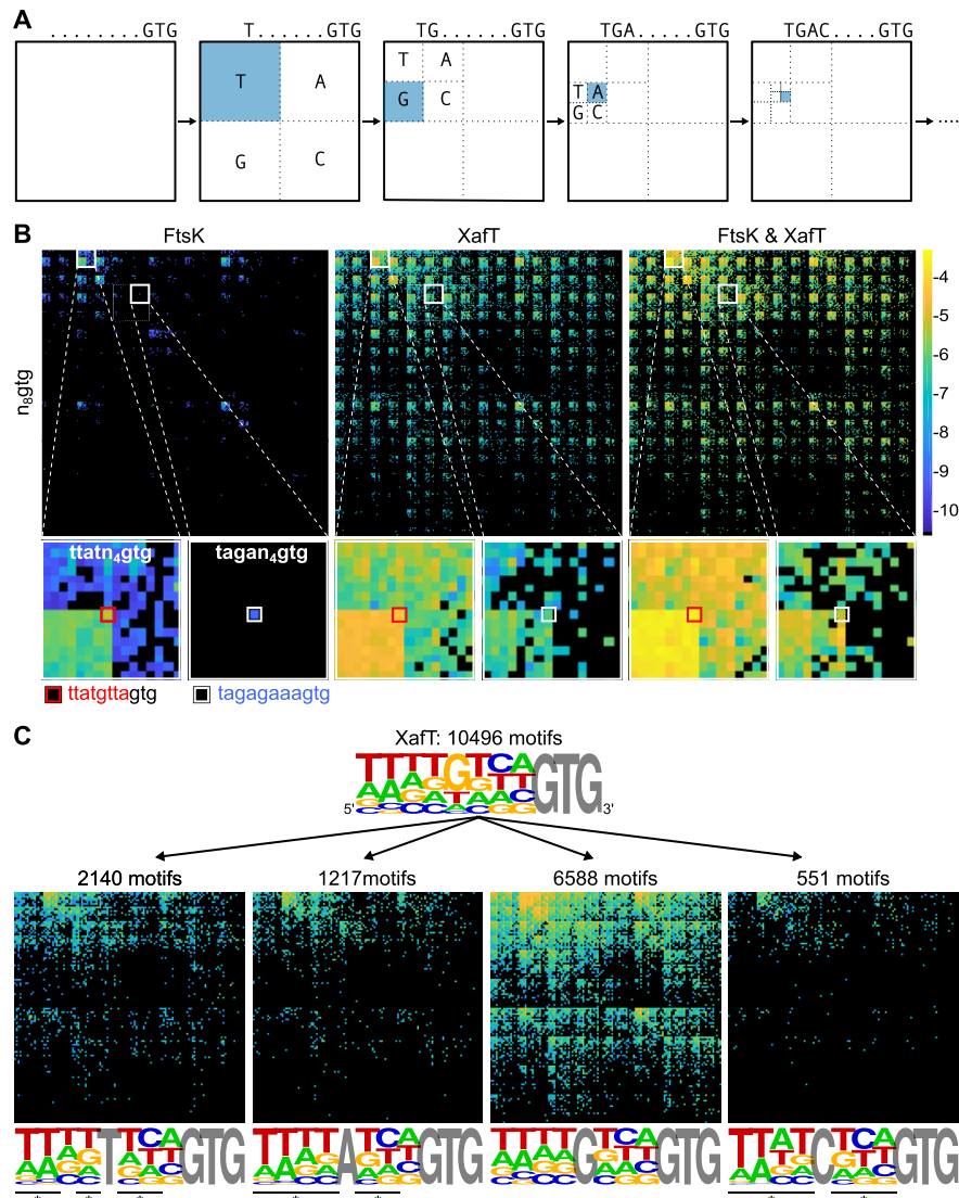
Figure 4. 2D-maps representation of the integration results. (A) 2D-map representation methodology: Different [x, y] coordinates are assigned to each nucleotide for the 2^8 possible motifs as follows: the [x, y] coordinates are initially set to [1, 1] . Then, [\frac{+1}{2^n}, \frac{+1}{2^n}] , [\frac{-1}{2^n}, \frac{+1}{2^n}] , [\frac{-1}{2^n}, \frac{-1}{2^n}] or [\frac{+1}{2^n}, \frac{-1}{2^n}] are added to [x, y] for each n position of the degenerate motif if the n th base is A, T, G or C, respectively. Relative integration efficiencies are represented with a dark-blue to bright yellow colour scale. Positions that were not found in the integration libraries are shown in black. (B) 2D-maps of the integrated n_8\text{gtg} motifs. FtsK: results from the conjugation of the n_8\text{gtg} XafT - mini-TLC \Phi library in the strain harbouring lacZ-dif1 at the natural dif1 locus; XafT: results from the conjugation of the n_8\text{gtg} XafT + mini-TLC \Phi library in the strain harbouring lacZ-dif1 at lacZ locus; FtsK & XafT: results from the conjugation of the n_8\text{gtg} XafT + mini-TLC \Phi library in the strain harbouring lacZ-dif1 at the natural dif1 locus. Below each 2D-maps are shown zooms of the regions corresponding to the 2^4 motifs that carry the same first innermost bases as the XerD arm of TLC \Phi attP (tagan 4 gtg) and dif1 (ttatn 4 gtg). The position of the TLC \Phi attP XerD motif and of the motif most similar to the XerD arm of dif1 are highlighted by white and red squares, respectively. Their sequences are indicated below the panels. Bases identical to the XerD-arms of TLC \Phi attP and dif1 are written in blue and red, respectively. 2D-maps of the integrated n_5a_2n_3\text{g} and tag 8 motifs are shown in Supplementary Figure S4. (C) Sequence logo of the XerD-arm of the attP sites of the n_8\text{gtg} XafT + mini-TLC \Phi plasmids that were found integrated in lacZ-dif1 at lacZ locus. The total number of n_8\text{gtg} integrated motifs is indicated. 2D-maps of the integrated n_4\text{tn}_3\text{gtg} , n_4\text{an}_3\text{gtg} , n_4\text{gn}_3\text{gtg} and n_4\text{cn}_3\text{gtg} motifs, as indicated. The number of integrated motifs from each category is indicated. The sequence logo the XerD-arm of the integrated sites from each category is shown below each 2D-map. Positions in which the bases of the integrated n_4\text{tn}_3\text{gtg} , n_4\text{an}_3\text{gtg} , and n_4\text{cn}_3\text{gtg} XerD-arm motifs are significantly different from the integrated n_4\text{gn}_3\text{gtg} XerD-arm motif are indicated by a star ( \chi^2 -test, P -value < 0.001).
