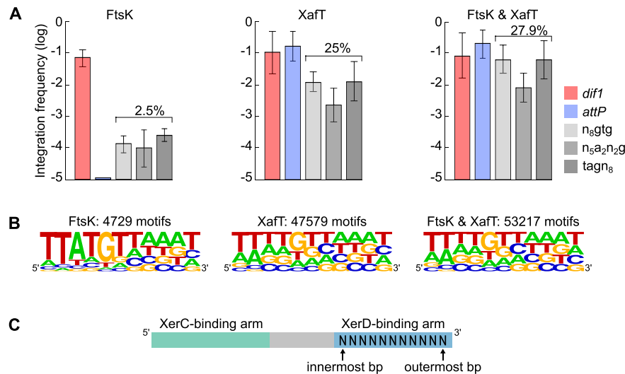
Figure 3. Non-replicative mini-TLC \Phi plasmid integration. (A) Integration frequencies of mini-TLC \Phi plasmids harbouring dif1 or TLC \Phi attP , and global integration frequencies of n8gtg , n5a2n3g and tagn8 plasmid libraries ( f_{int} ). FtsK panel: XafT - plasmids conjugated in a strain harbouring dif1 at its natural locus; XafT panel: XafT + plasmids conjugated in a strain harbouring dif1 at the lacZ locus; FtsK & XafT panel: XafT + plasmids conjugated in a strain harbouring dif1 its natural locus. Mean and standard deviations of at least 3 independent assays. (B) Combined sequence of the XerD-arm from the n8gtg , n5a2n3g and tagn8 integration libraries. The logos show the frequency of each base at the degenerate positions. The number of integrated motifs top which each logo corresponds is indicated. Individual logos are shown in Supplementary Figure S3. (C) Illustration of our naming scheme for bases of the XerD-binding arm.
