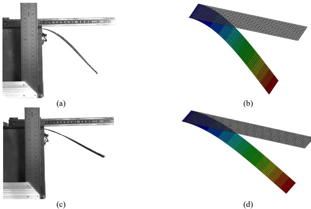
Fig. 7. Cantilever test of G1151 interlock fabric. (a) Bending experiment along warp yarn (b) Bending simulation along warp yarn (c) Bending experiment along weft yarn (d) Bending simulation along weft yarn
