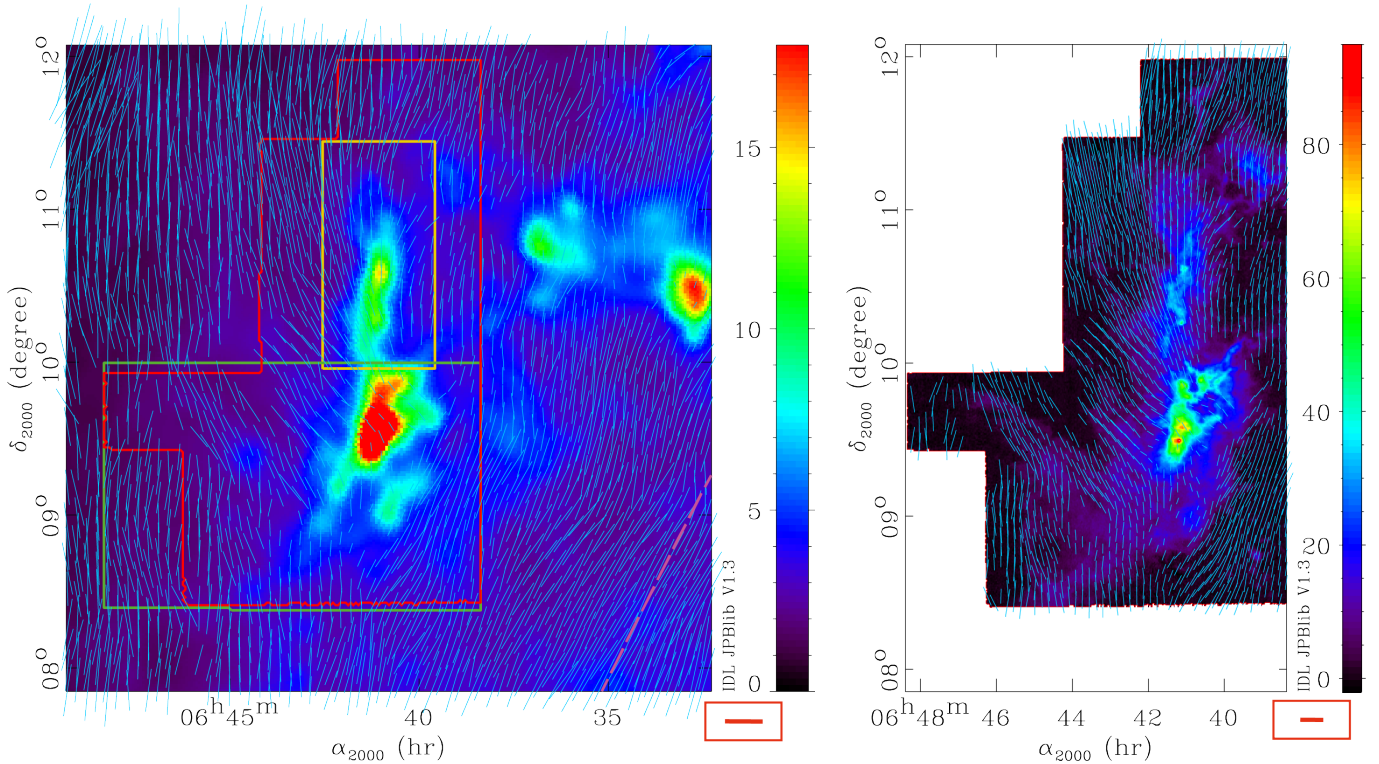
Fig. 3. Monoceros OB 1 east region observed by Planck and TRAO. Left panel: Planck 353 GHz intensity map in MJy sr -1 at the angular resolution of 7' with the POS magnetic field orientation overlaid as blue segments. The length of the segments corresponds to polarization fraction, with the reference length of 15' corresponding to p = 0.05 (shown in the red box in the bottom right corner). Only data satisfying S/N(p) \geq 2 and \sigma_\psi < 10^\circ are used for polarization studies. Red, yellow, and green lines show contours of the TRAO map used in this analysis, the northern region (Fig. 5), and the southern region (Fig. 10) respectively. The pink dashed line shows the isolatitude b_{||} = 0^\circ . Right panel: TRAO 12 CO (J=1–0) integrated (between v_{lsr} = -3 and 17 km s -1 ) T_a^* intensity map in K km s -1 at angular resolution of 47'' with the POS magnetic field orientation derived from the Planck data overlaid as blue segments. Red contour corresponds to the red contour in the left panel.
