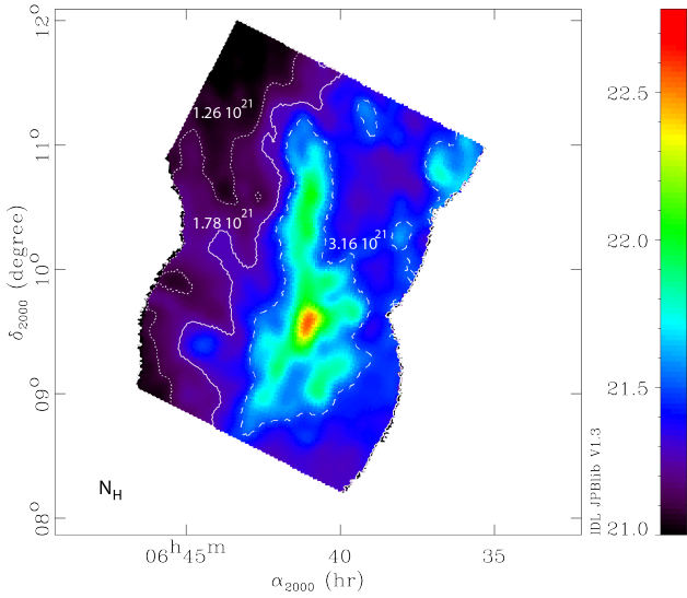
Fig. 2. Column density ( N_H ) map derived using the Planck and IRIS data, in the logarithmic scale and in \text{cm}^{-2} . The contours correspond to 1.26 \times 10^{21} , 1.78 \times 10^{21} , and 3.16 \times 10^{21} \text{ cm}^{-2} .
