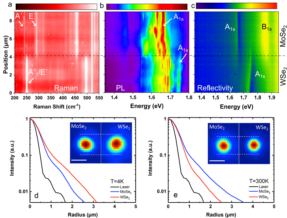
Fig. 2 Far field optical study. Contour plot of (a) Raman ( \lambda_L = 633\text{nm} ), (b) PL ( \lambda_L = 633\text{nm} ) and (c) white light reflectivity spectra scans across a \text{WSe}_2 - \text{MoSe}_2 heterojunction at T = 5\text{ K} . The black horizontal dashed line indicates the position of the heterojunction. Color bars for panels (a), (b) and (c) are normalized from 0 to 1. d Exciton diffusion measurements at a temperature of T = 4\text{ K} for the \text{MoSe}_2 monolayer region (blue) and \text{WSe}_2 (red). In the inset we show the \text{MoSe}_2 diffusion PL profile compared to the \text{WSe}_2 one. The laser intensity profile (black) is shown to indicate over which area excitons are initially generated, with small intensity oscillations due to Airy discs visible in logarithmic scale. e Same as d but at T = 300\text{ K} .
