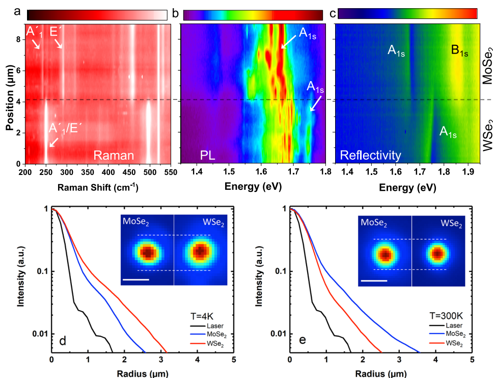
Fig. 2 Far field optical study. Contour plot of (a) Raman ( \lambda_L = 633\text{nm} ), (b) PL ( \lambda_L = 633\text{nm} ) and (c) white light reflectivity spectra scans across a WSe 2 -MoSe 2 heterojunction at T = 5\text{ K} . The black horizontal dashed line indicates the position of the heterojunction. Color bars for panels (a), (b) and (c) are normalized from 0 to 1. d Exciton diffusion measurements at a temperature of T = 4\text{ K} for the MoSe 2 monolayer region (blue) and WSe 2 (red). In the inset we show the MoSe 2 diffusion PL profile compared to the WSe 2 one. The laser intensity profile (black) is shown to indicate over which area excitons are initially generated, with small intensity oscillations due to Airy discs visible in logarithmic scale. e Same as d but at T = 300\text{ K} .
