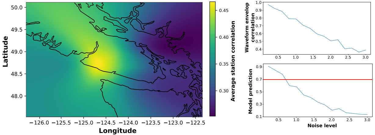
Fig. 3. Tremor location and robustness. (Left) Example tremor location. We compute the envelope of the cleaned signals; these envelopes are then sliced around each identified STA/LTA pick, and cross-correlated for all station pairs. This figure shows the stacked correlation plotted over the lat/lon grid for one tremor. If a number of criteria are met (see below), the maximum of the stacked correlation function is returned as the tremor’s location. (Right) Impact of noise on located signals. We overlay input tremor waveforms with seismic noise at different coefficients. We then perform the attribution analysis of the original and corrupted signals, and compare both extracted waveforms by computing their (top right) envelope correlation. We also compute the associated (bottom right) model prediction. In both plots, the blue line corresponds to the average value computed from approximately 5000 examples. When strong levels of noise are added, both the model’s prediction and the envelope correlation decay. Because we only try to locate signals above a “confidence” threshold of 0.7 (red line in bottom), our algorithm would not attempt to locate signals for which the added noise has strongly impacted the attribution analysis.
