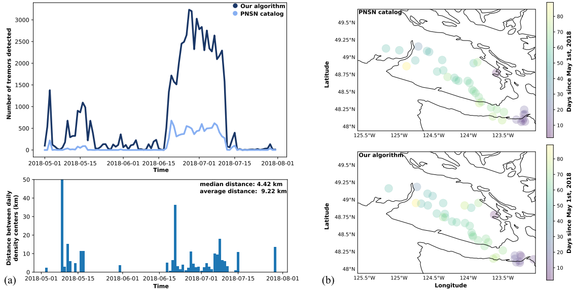
Fig. 6. Comparison with the PNSN catalog. (a) (Top left) Number of tremors detected by our algorithm (dark blue), compared to the number of detected tremors in the PNSN catalog (light blue). The timing of detections is consistent between both catalogs, with a high number of tremors detected between June 18th and July 11th. (Bottom left) Distance between daily tremor patches detected by our algorithm and by the PNSN catalog. For most days, the patches have similar locations (with a median distance of 4.42 km). The two days where the distance is high correspond to patches in the PNSN catalog that are on the border or outside of our seismic array. (b) Evolution of the center of daily tremor patches over the period analyzed, in (top right) PNSN catalog and (bottom right) in our analysis. Tremor migration patterns are similar with both algorithms.
