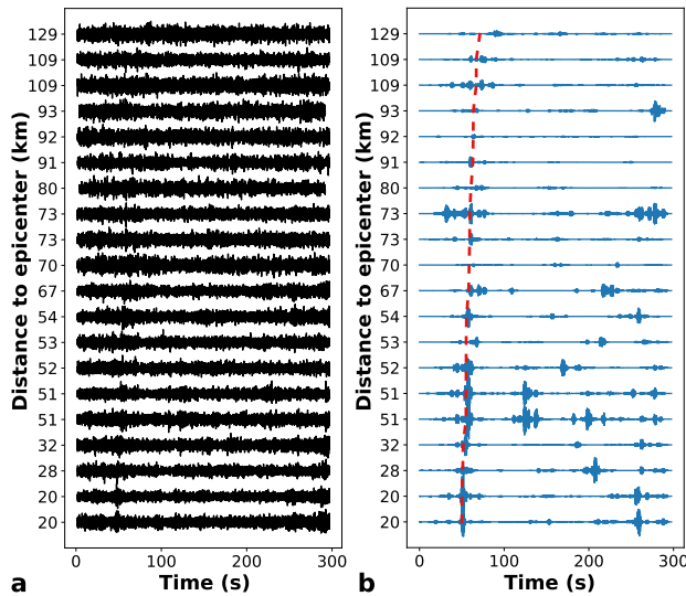
Fig. 2. Application to an array of seismometers. (a) Raw waveforms bandpassed between 1 and 8 Hz. (b) Result of the neural network attribution analysis to denoise the waveforms (in blue). The extraction procedure is performed on each station independently. Clean move-out patterns can be seen across the network, which can be compared to shear wave theoretical travel times (red line). The move-outs match theoretical wave speed to first order. Note that in order to visualize the moveout, waveforms are ordered according to the epicenter of one particular tremor (occurring at 50 s).
