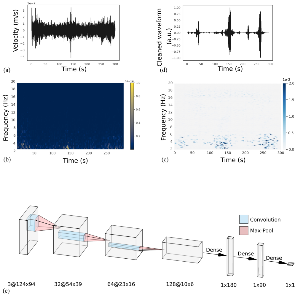
Fig. 1. Extraction of tremor waveforms with neural network attribution. Raw waveforms (a) are turned into spectrograms (b) and fed to a classic CNN. We rely on a standard network (three convolution+max pool and three dense layers). From these spectrograms, the CNN is tasked with classifying tremor from nontremor. Once the model is trained (with tremors identified from the PNSN catalog), we rely on Integrated Gradients [41] attribution to interpret its results. (c) Result of the positive attribution for the same waveform; the blue areas correspond to the parts of the spectrogram that carry core tremor information according to the attribution analysis. We can then select exclusively these areas to inverse-Fourier transform, to get a clean tremor signal. (d) These cleaned waveforms correspond to the core tremor signals, as seen by our model, and have clear structure compared to the original waveforms; our goal here is to rely on these clean waveforms to locate tremors. (e) Architecture of the network.
