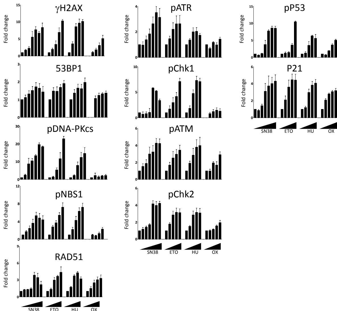
Figure 4. Dose-dependent DDR response of HCT116 cells to DNA damaging agents. Cells were treated overnight with increasing concentrations of SN38 (0, 0.2, 1, 5, 16, 80, 2000 nM), Etoposide (0, 1, 2, 6, 30, 150 \mu M), Hydroxyurea (0, 0.12, 0.6, 3, 15 mM), or Oxaliplatin (0, 0.4, 2, 10, 50 \mu M) and DDR markers were evaluated as indicated in figure 3. The results show the ratios of the average number of fluorescent cells following SN38 treatment as compared to untreated cells for each DDR marker. Results are the mean \pm SEM of 2-4 independent experiments.
