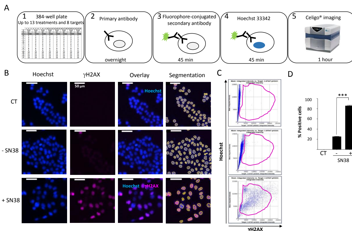
Figure 2. (A) Celigo® imaging flow chart used for DDR evaluation. (B) Representative fluorescence images of H2AX phosphorylation obtained for HCT116 cells in the absence or in the presence of SN38 (2 \mu M, 24 h). Hoechst was used for nuclear staining and total cell count using the dedicated segmentation protocol (right panel). Images were acquired and analysed using the Target + Mask application. CT: control cells stained with the secondary antibody alone. (C) Representative flow-like analyses of the images obtained in (B). The dot-plots show Hoechst integrated intensity as a function of \gamma H2AX integrated intensity. A gate (in purple) was defined for the control condition (CT) and applied to all other conditions to determine the percentage of positive cells and the fluorescence intensity in each cell. (D) Percentages of fluorescent positive cells for \gamma H2AX labelling are plotted as a function of cell treatment. The bar graphs represent the quantitative analyses (mean \pm SD ; n=3) of the fluorescent images from one representative experiment. Statistical analysis was carried out using Student's t -test; (***) : p<0.0001.
