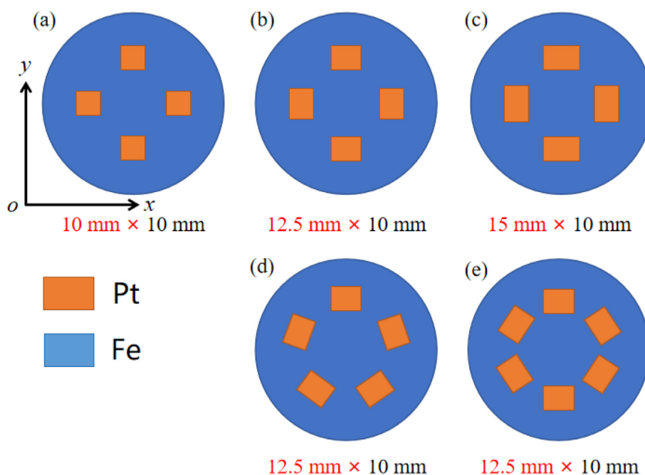
Fig. 2 – Schematic diagrams of the targets used to produce compositionally homogeneous FePt films indicating the position and size of Pt foils on a base Fe target: (a) target #4, (b) target #5, (c) target #6, (d) target #7, (e) target #8.
