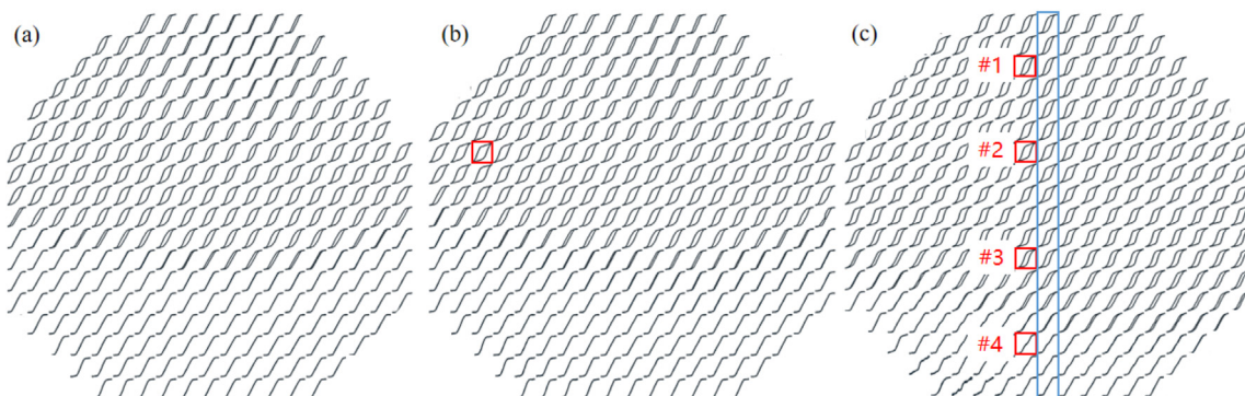
Fig. 7 – 2D Scanning polar MOKE maps of wafers, made from target #2, annealed at 600 °C for (a) 1 min, (b) 10 min (c) 30 min. Reference samples at the positions #1 to #4 were diced out of the wafer to make SQUID-VSM measurements.
