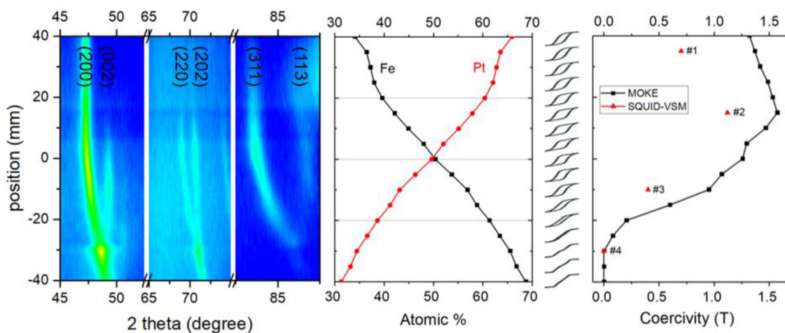
Fig. 11 – 2D Select sections of XRD patterns together with the film composition from EDX, MOKE loops and coercivity values (black symbols), plotted as a function of position along a vertical section of the film annealed at 600 °C for 30 min. Coercivity values estimated from SQUID-VSM measurements of select samples are overlaid on the MOKE coercivity graph (red symbols). (For interpretation of the references to colour in this figure legend, the reader is referred to the Web version of this article.)
