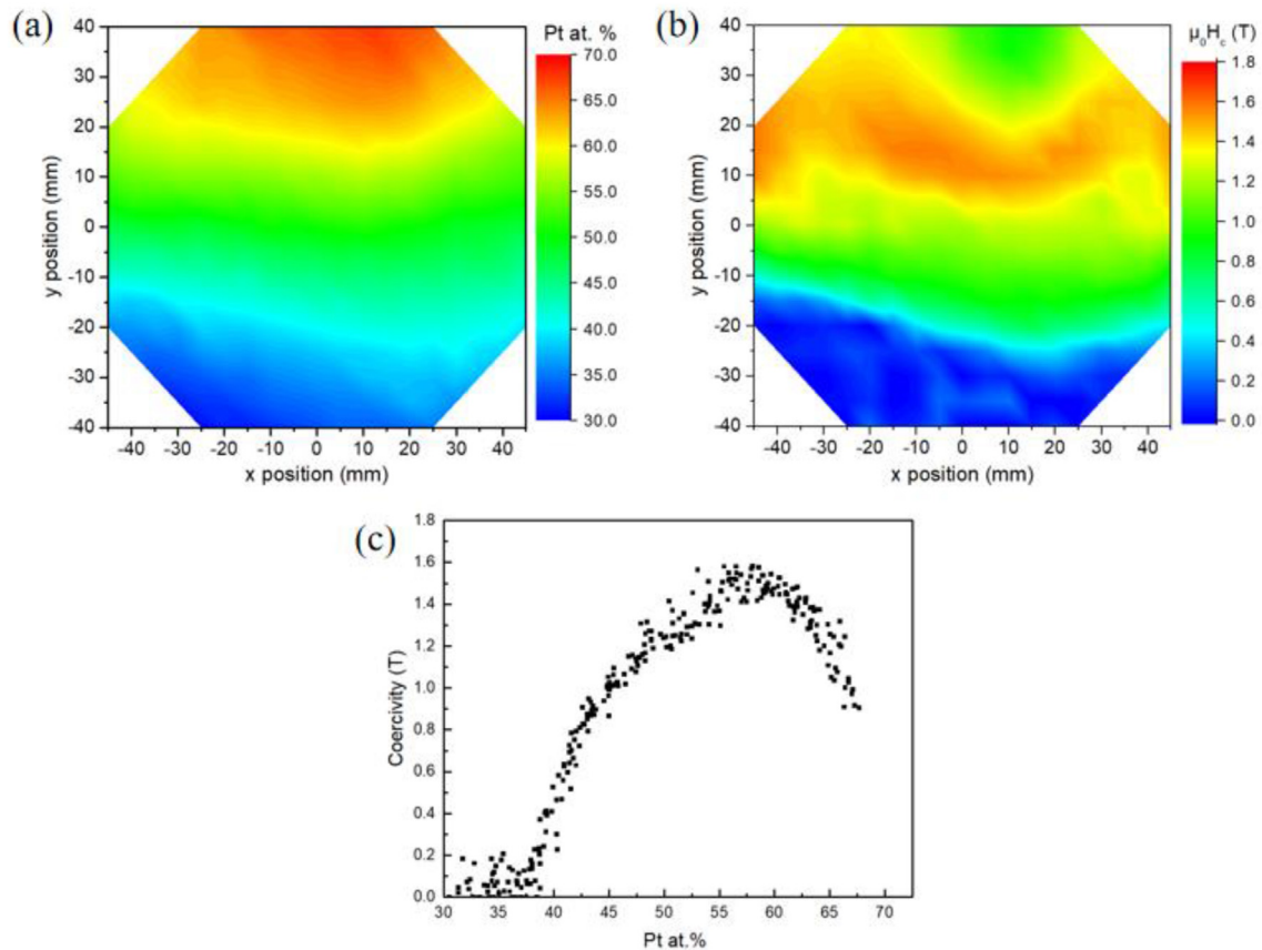
Fig. 6 – Comparison of (a) the Pt content EDX map of an as-deposited film made using target #2, and (b) a coercivity map extracted from MOKE loops measured on such a film annealed at 600 °C for 30 min (see Fig. 5b); (c) plot of coercivity as a function of Pt content, measured over the entire wafer.
