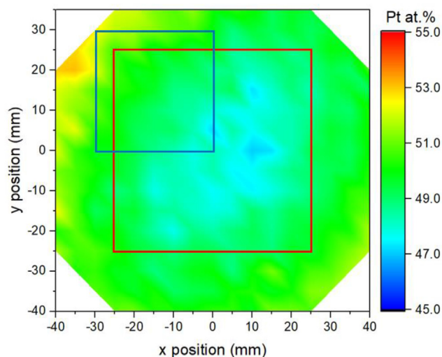
Fig. 13 – 2D EDX map of Pt content measured over a full wafer of a film made using target #6. The red box indicates the 50 \times 50 \text{ mm}^2 wafer zone probed in Fig. 12, the blue box the 30 \times 30 \text{ mm}^2 region probed in Fig. 14. (For interpretation of the references to colour in this figure legend, the reader is referred to the Web version of this article.)
