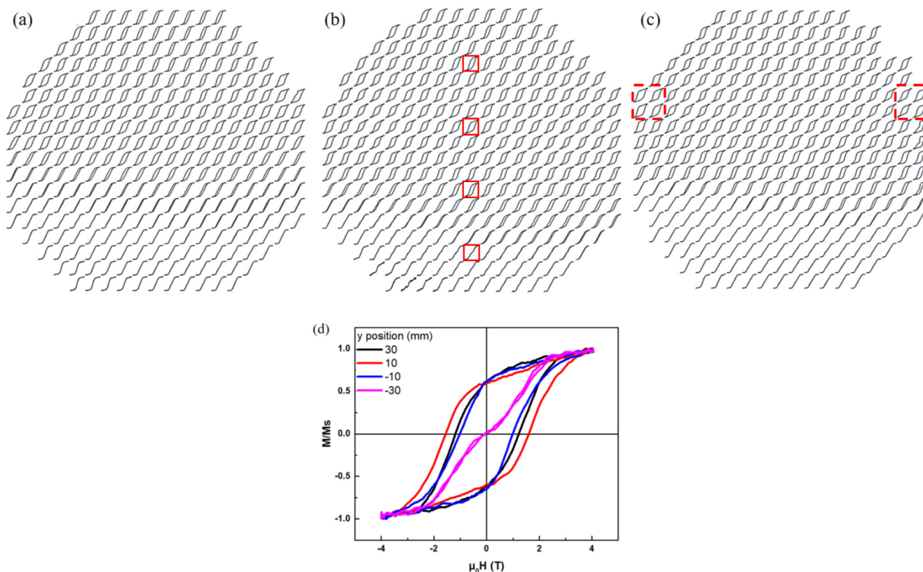
Fig. 5 – 2D Scanning polar MOKE maps of wafers, made from target #2, annealed at (a) 500 °C, (b) 600 °C and (c) 700 °C for 30 min (maximum applied field = 4 T; MOKE intensity values are normalised), (d) Enlarged typical MOKE loops from Fig. 5b at the regions identified by red boxes. (For interpretation of the references to colour in this figure legend, the reader is referred to the Web version of this article.)
