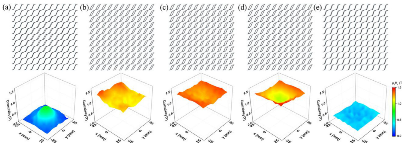
Fig. 12 – Polar MOKE loops and coercivity maps on a 50 \times 50 \text{ mm}^2 region of Fe–Pt films sputtered using targets #4 - #8 and then annealed at 600^\circ \text{C} for 10 min.
