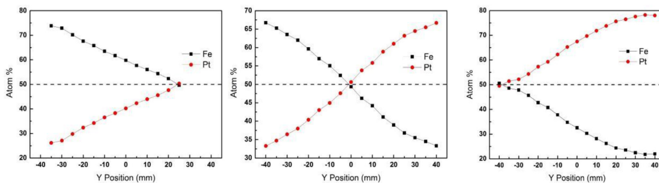
Fig. 3 – 1D EDX line scans of Fe and Pt content measured along the horizontal bi-sector (i.e., parallel to the y-axis) of samples fabricated using targets (a) #1, (b) #2 and (c) #3.
