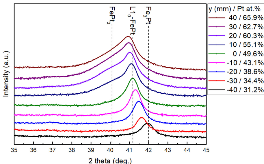
Fig. 9 – Zoom of the XRD patterns of the (111) reflection of Fig. 8. The experimental data is overlaid with dashed lines indicating the position of the (111) peak of chemically ordered L1 2 -FePt 3 , L1 0 -FePt and L1 2 -Fe 3 Pt.
