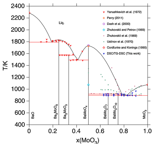
Fig. 12. BaO-MoO 3 pseudo-binary phase diagram computed from the thermodynamic model, and comparison with the experimental data.
