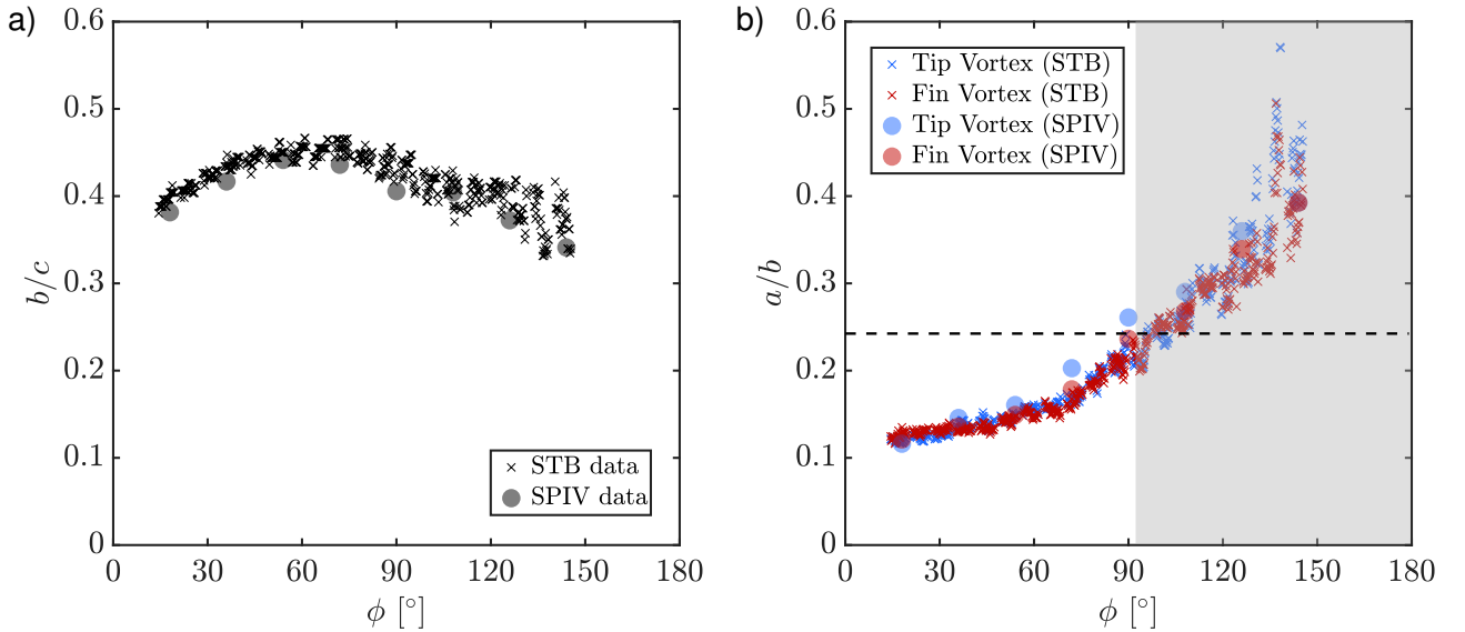
Figure 5 – (a) Development of the vortex core distances for STB and SPIV data. (b) Evolution of the relation between Gaussian core radii and vortex distance a/b for different rotor phases (dashed black line marks the critical ratio of a/b = 0.24 determining the onset of vortex merging).
