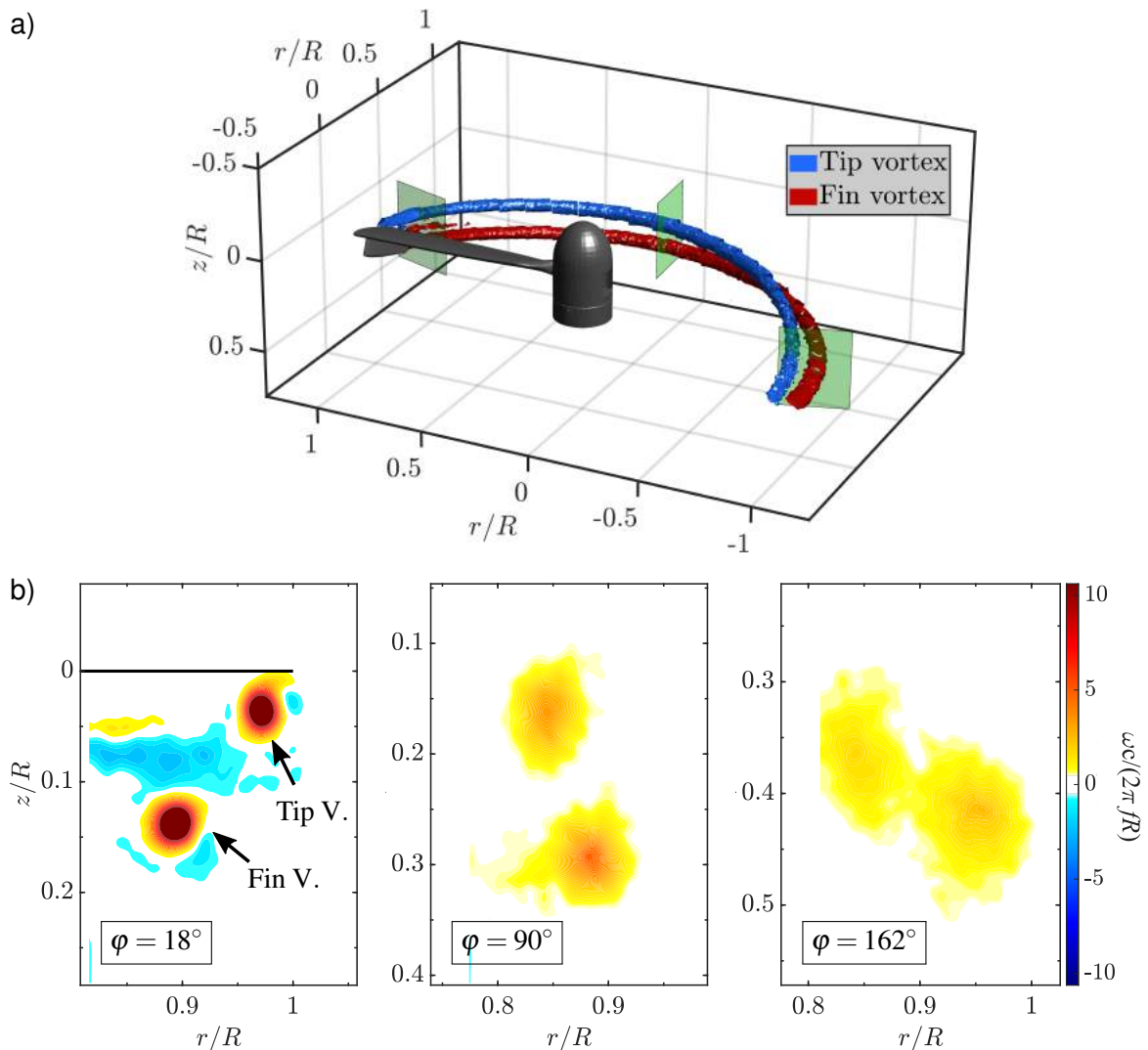
Figure 2 – (a) Volumetric isosurfaces of the normalised azimuthal vorticity component up to a rotor phase of \varphi = 185^\circ for the modified blade (green slices indicate the position of the fieldcuts shown in (b)). (b) Phase-averaged vorticity contours at \varphi = 18^\circ , \varphi = 90^\circ and \varphi = 162^\circ , black line represents the trailing edge of the blade.
