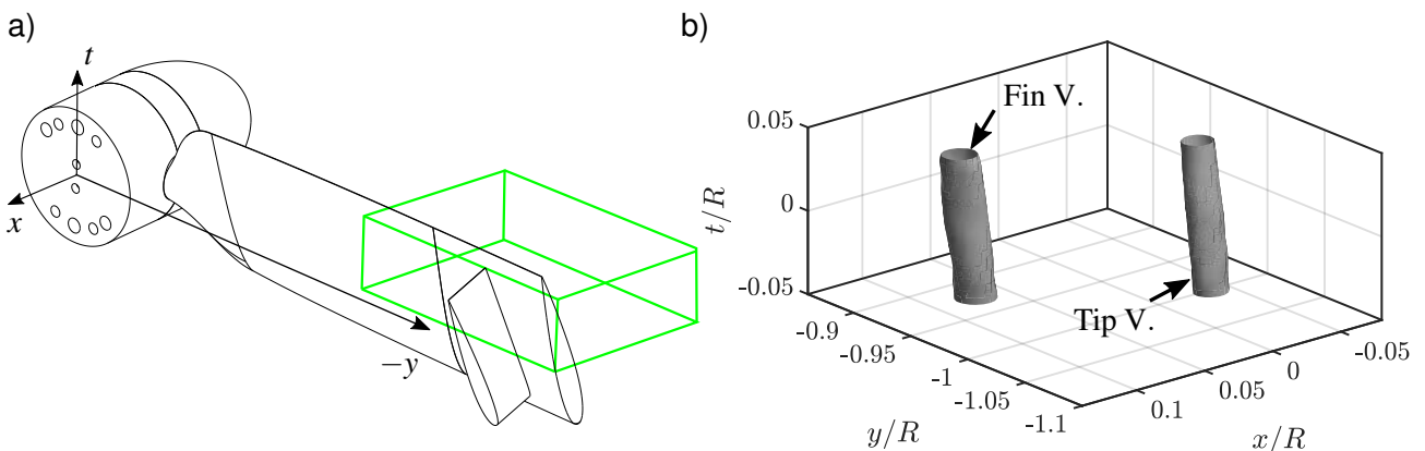
Figure 6 – (a) Sketch of the STB measurement volume in relation to the rotor blade and local coordinate system used for subsequent analysis. (b) Isosurface of the Q-criterion at a rotor phase \varphi = 24^\circ for phase-averaged data.
