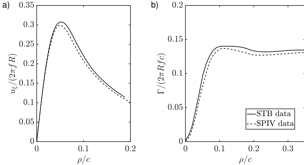
Figure 3 – (a) Radial swirl velocity and (b) radial circulation profiles for the tip vortex at a rotor phase of \varphi = 18^\circ . Profiles extracted from both STB and SPIV data.
