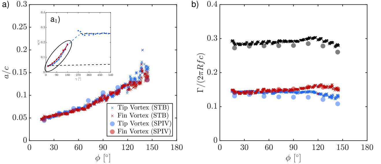
Figure 4 – (a) Gaussian core radii evolution of both vortices in the region of rapid growth (marked with the black ellipse within the full SPIV diagram ( a_1 )) for STB and corresponding SPIV data. (b) Circulation values obtained for the distinct vortices and the total field (black).
