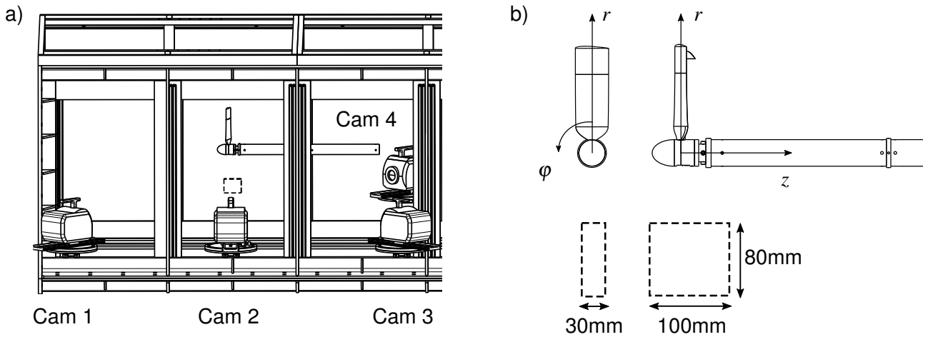
Figure 1 – (a) Schematic of the experimental setup for the particle tracking velocimetry measurements. (b) Global coordinate system for the rotor geometry (free stream is in z -direction) and measurement volume dimensions.
