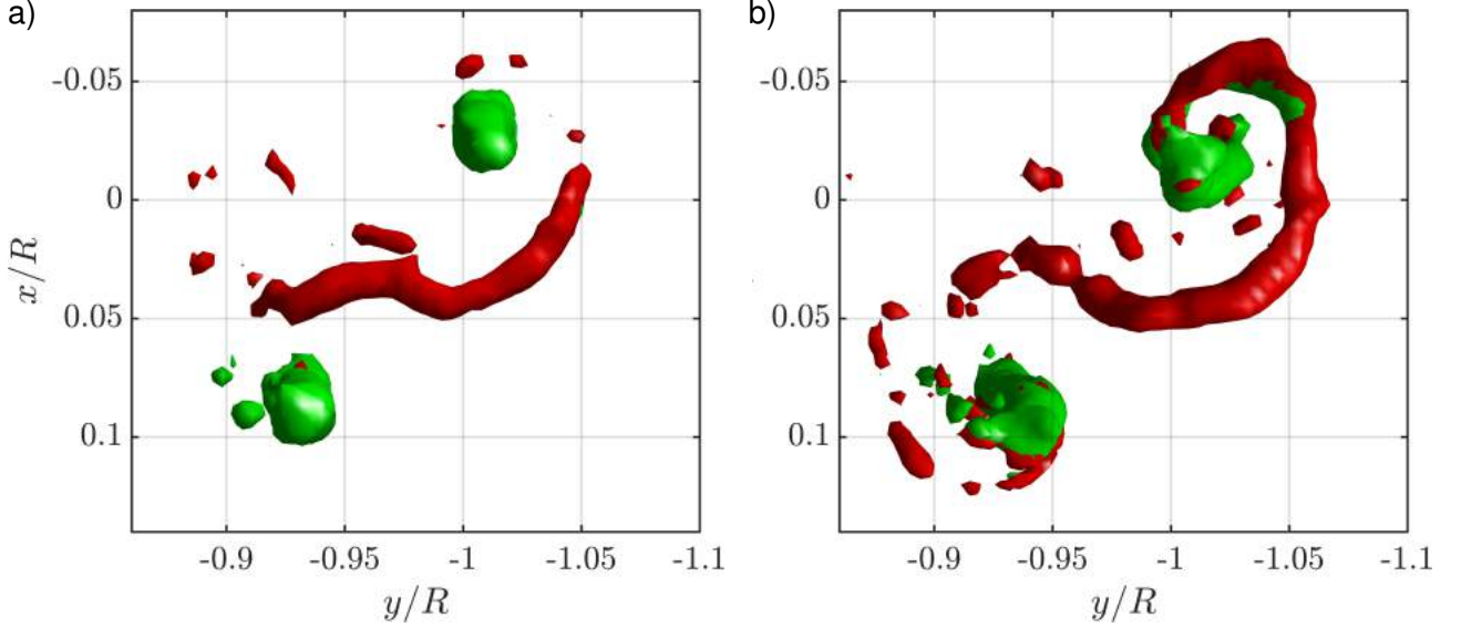
Figure 8 – (a-b) Top view of the decomposed criteria shown in Fig. 7(b-c).
