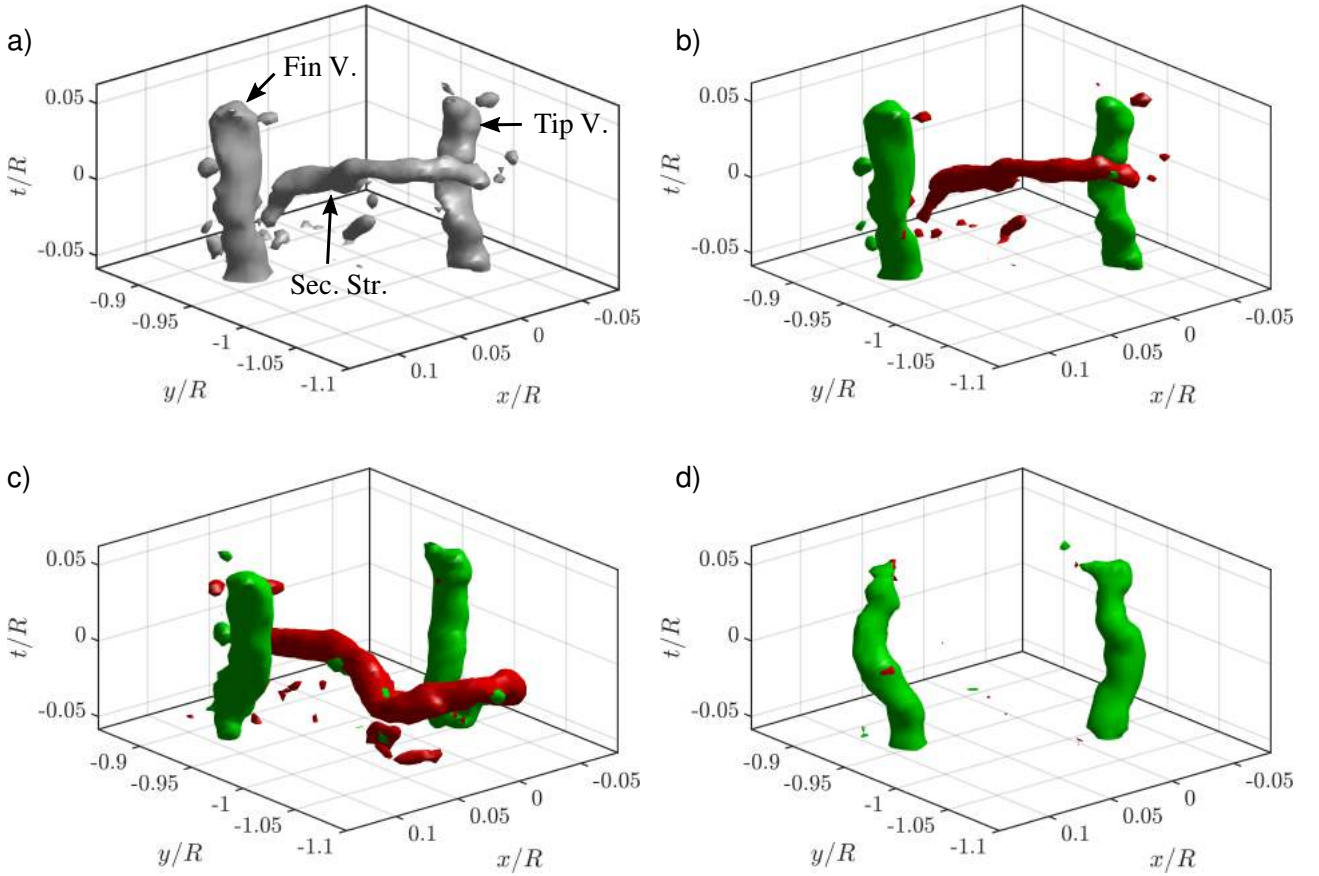
Figure 7 – (a) Instantaneous isosurfaces of the Q-criterion at a rotor phase \phi = 24^\circ . (b) Decomposition of the instantaneous Q-criterion into Q_{tip} (green) and Q_{sec} (red). (c-d) Additional examples for instantaneous isosurfaces using the decomposed criteria.
