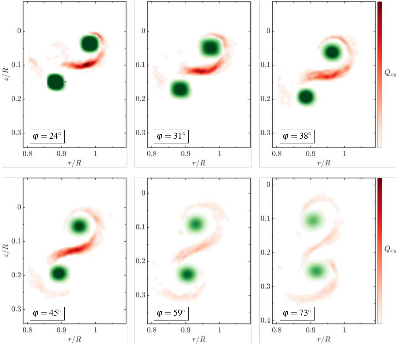
Figure 9 – Phase-averaged volumes showing the development of the primary vortices Q_{tip} (green) and the secondary vortex structures Q_{sec} (red) for different phase angles \varphi (volumes are averaged in t -direction).
