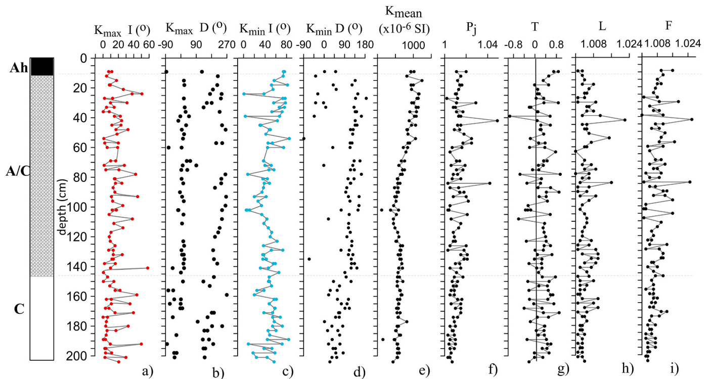
Fig. 7. Variations with depth of declination and inclination of K_{\max} and K_{\min} (a–d); mean volume susceptibility ( K_{\text{mean}} ) (e) and anisotropy parameters: corrected degree of anisotropy (Pj), shape parameter (T), lineation (L) and foliation (F).
