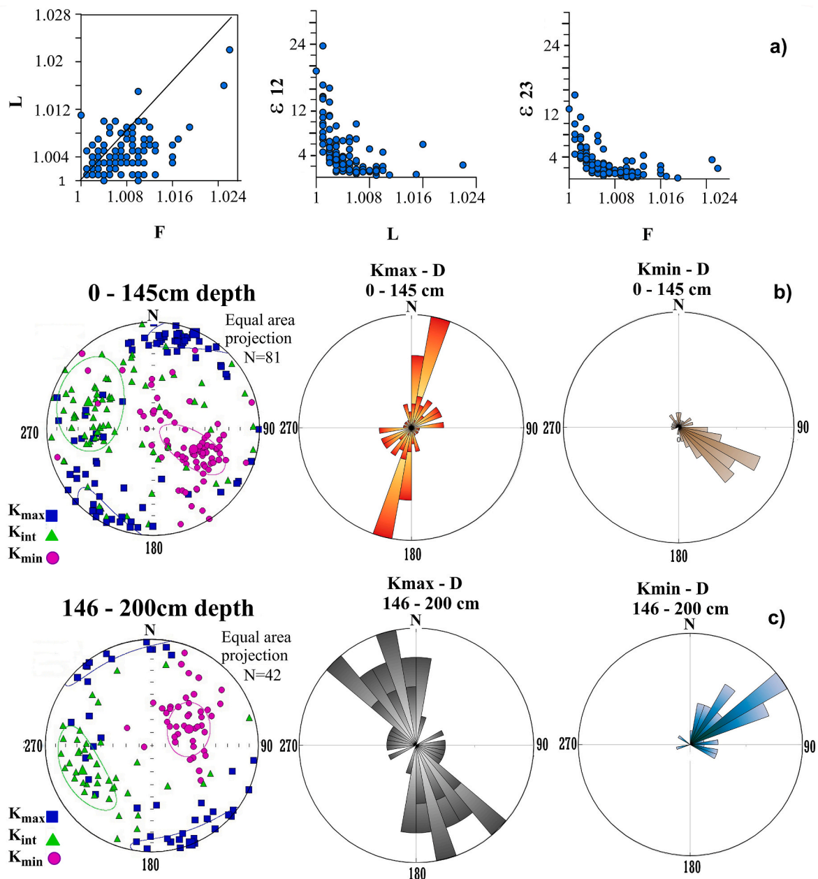
Fig. 6. Results from anisotropy of magnetic susceptibility measurements. A) bi-plots of lineation (L) versus foliation (F); 95% confidence half angle around K_{max} and K_{int} within the K_{max} - K_{int} plane ( \epsilon_{12} ) versus magnetic lineation L, and around K_{min} and K_{int} within the K_{min} - K_{int} plane ( \epsilon_{23} ) versus F; b) lower hemisphere stereographic projection (geographic coordinates) of the maximum ( K_{max} ), intermediate ( K_{int} ) and minimum ( K_{min} ) AMS principal axes of samples from the soil Ah and A/C horizons developed in deluvial clays; rose diagram of the K_{max} declinations and plunge of the poles to the imbrication plane (D- K_{min} ). c) the same as b) for samples from the alluvial clays in the C horizon.
