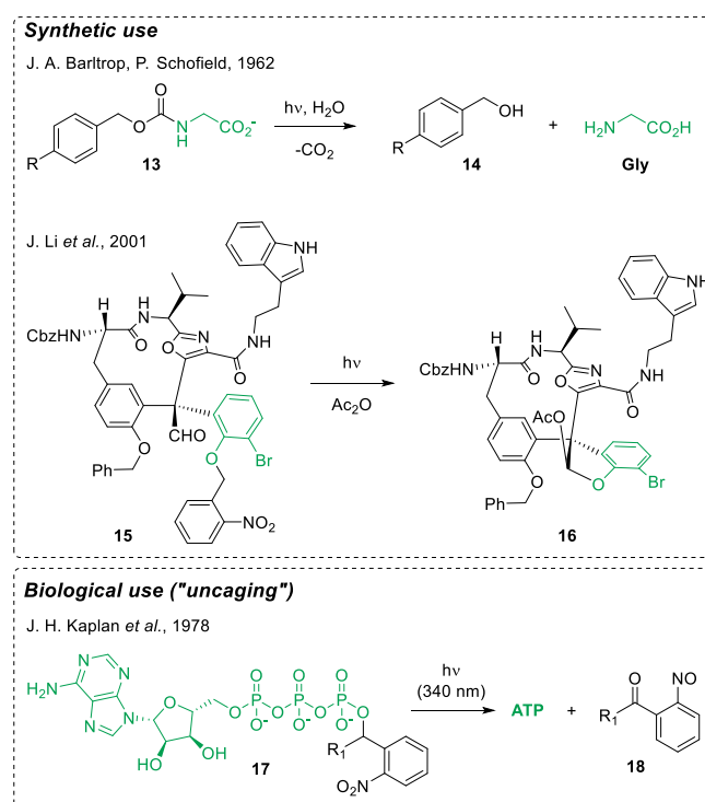
Scheme 1. Early examples of photo-deprotection of glycine[48] and of phenol intermediate 15 [50] for synthetic purposes, and of ATP in biological applications.[51]
