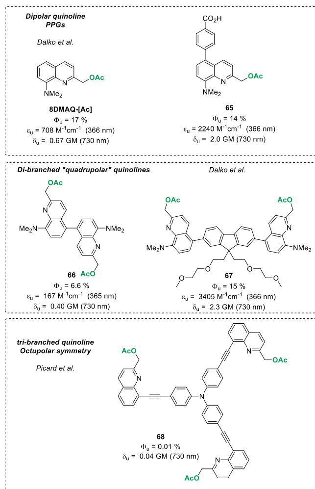
Figure 13. Examples of dipolar, quadrupolar and octupolar quinoline derivatives and the resulting effect on the 2PU properties.
