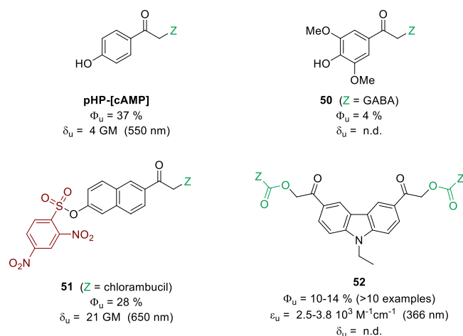
Figure 10. Structures of PPGs containing the phenacyl photosensitive unit and corresponding 1P and 2PU properties.
