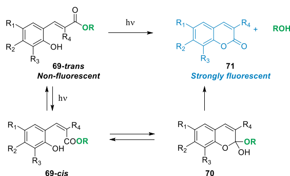
Scheme 8. Reported mechanism for the photorelease of alcohols with o HC derivatives involving sequential E-Z photo-isomerisation and lactonisation.
