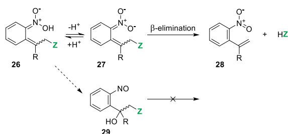
Scheme 3. \beta -elimination mechanism occurring during the photofragmentation of ortho -nitrohomobenzyl derivatives.
