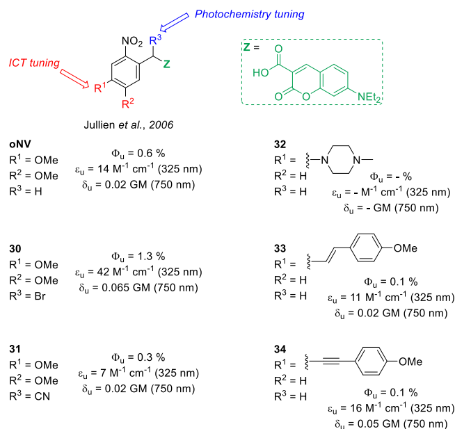
Figure 7. Examples of modified o NB derivatives reported by Jullien and co-workers for the photorelease of a caged fluorophore, and their photochemical properties in MeCN:TRIS buffer (1:1, v:v).[67]
