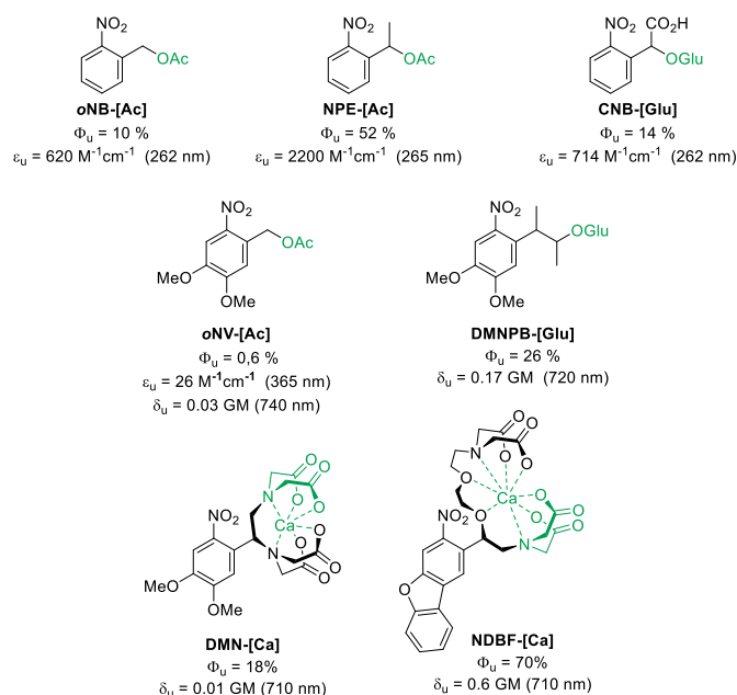
Figure 6. Structures and key photophysical properties of the first PPGs of the nitrobenzyle family cleaved by 1P or 2PE.
