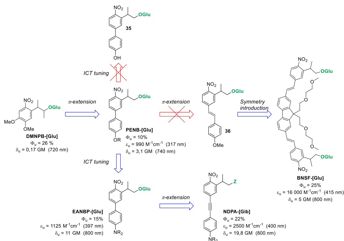
Figure 8. Roadmap of the structural modifications performed on NPPOC derivatives in order to optimise their 2PU cross-section. R = di(ethyleneglycol) ; Z = gibberellic acid.
