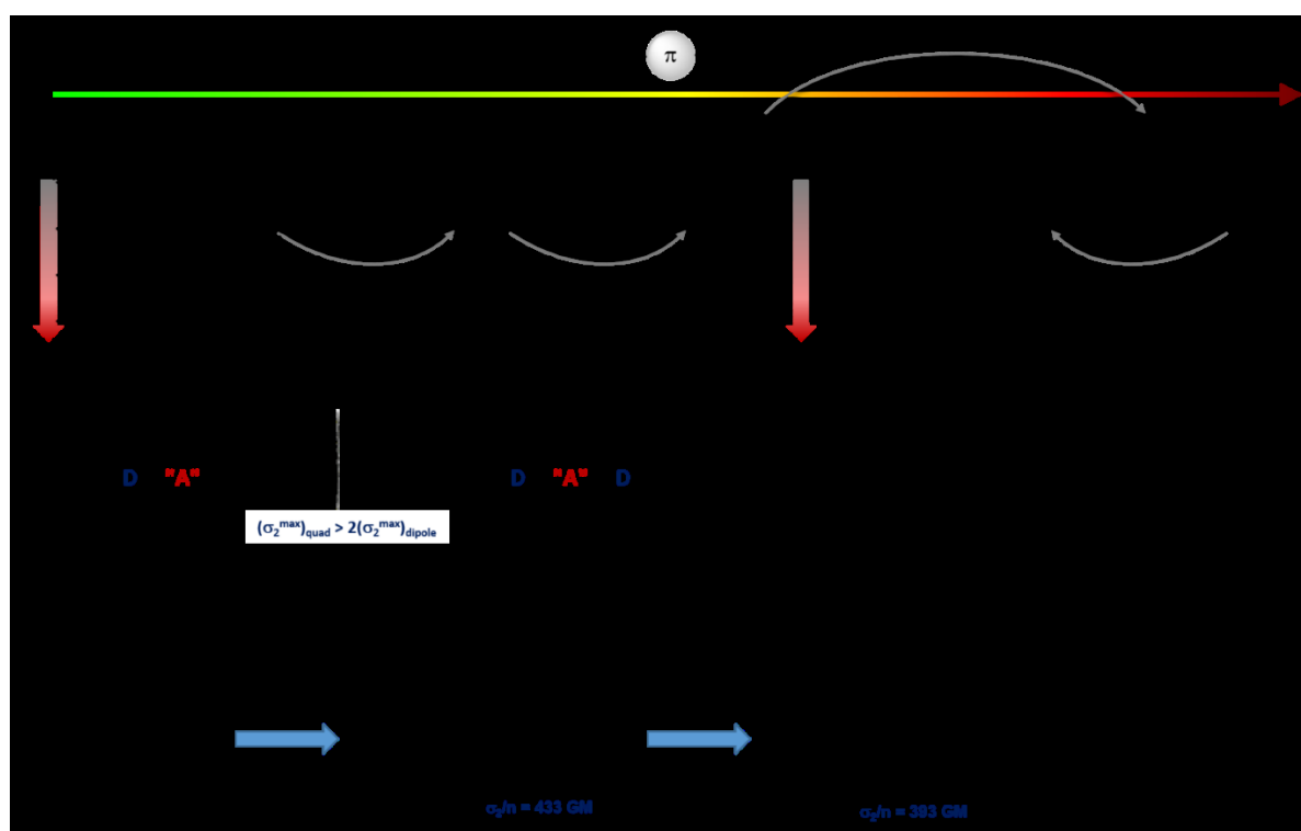
Figure 4. a) Roadmap of the structural modifications performed on centrosymmetric chromophores and stilbene derivatives, and evolution of the \sigma_2 as a function of ICT, and conjugation (length and planarity).[31,39,40] b) Comparison of \sigma_2^{max} and \lambda_{2PA}^{max} values in dipole 9 quadrupole 10 of equivalent strength.[41] c) Effect of the degree of branching on \sigma_2 and \sigma_2/n values in compound 3 , corresponding octupole D(- \pi -D) 3 11 [39] and multibranch compound 12 . [42]
