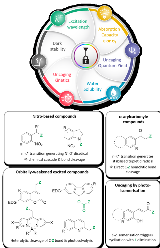
Figure 5. Summary of the specifications required for use of PPGs in biology, and of the main families of photosensitive moieties classified by type of mechanism.
