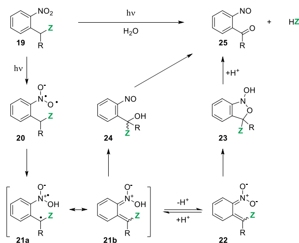
Scheme 2. Photofragmentation mechanism reported for o NB derivatives in aqueous media.
