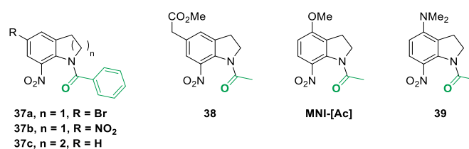
Figure 8. First examples of ortho -nitroanilides compounds studied for the photorelease of carboxylic acids by Amit et al. ( 37a,c )[80] then Papageorgiou and Corrie ( 38, 39 and MNI-[Ac] ).[81,82]
