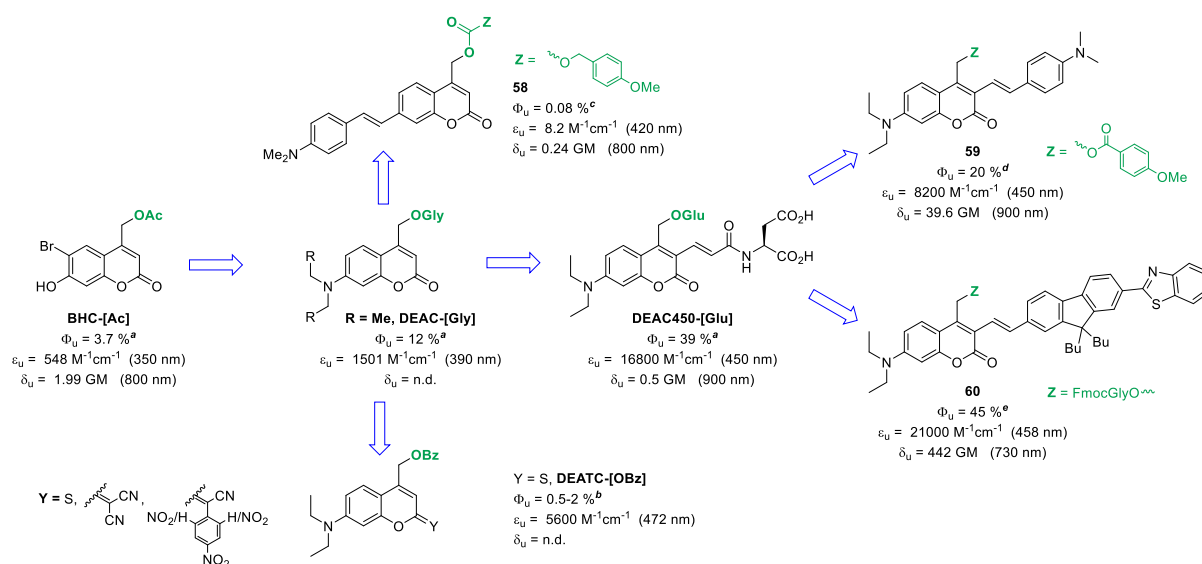
Figure 11. Roadmap of the structural modifications performed on the coumarin backbone, and their consequences on the 1P and 2PU properties. Values are reported for photolysis in a phosphate buffer; b phosphate buffer with 50% MeCN; c phosphate buffer with 90% MeCN d MeOH:H 2 O (9:1, v:v) e MeCN:H 2 O (9:1, v:v).
