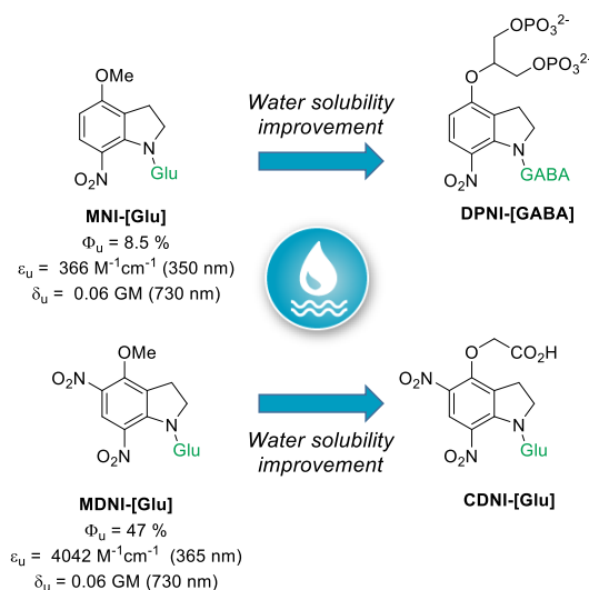
Figure 9: Structures of the most common 2P-sensitive NI-caged neurotransmitters.
