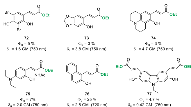
Figure 14. Structures and photochemical properties of o HC compounds uncaging model alcohols.
