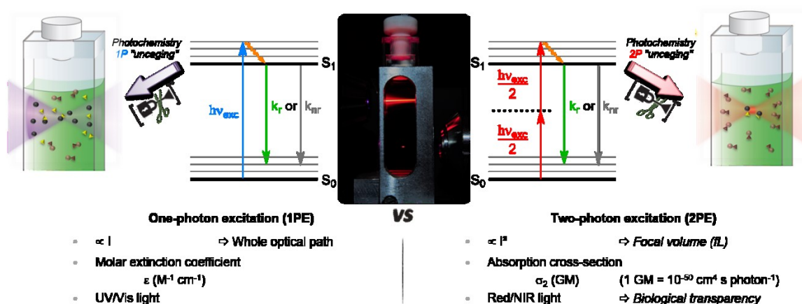
Figure 1. Simplified Jablonski diagrams and key features of the 1PA (left) and 2PA phenomena (right) in the case of an active substrate (triangle) protected with a PPG (circle), and the resulting volume of photorelease in each case. The center picture illustrate the difference in spatial resolution between both types of excitation with the example of red-
