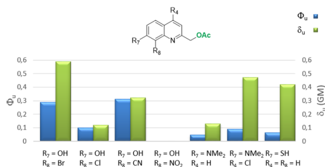
Figure 12. Evolution of the uncaging quantum yield (blue) and the 2PU cross-section (green) in substituted quinoline PPGs for the release of acetic acid.[152]
