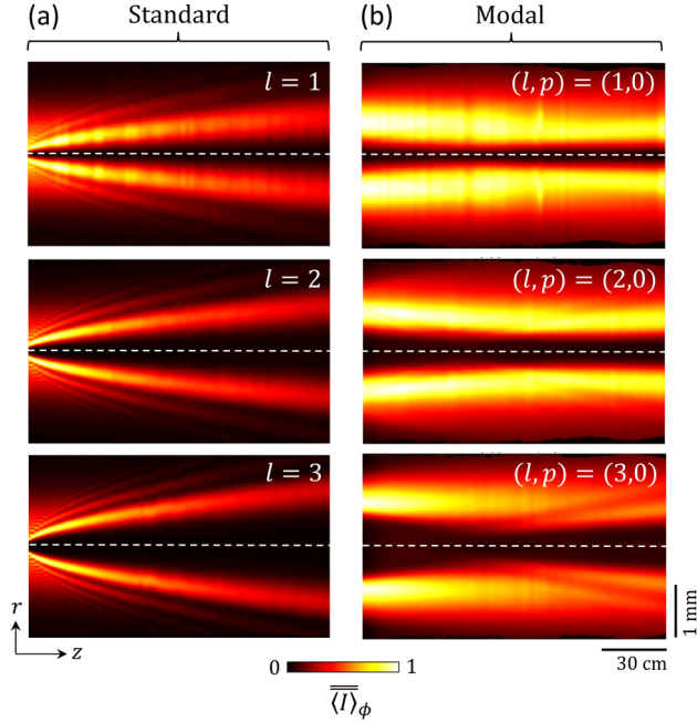
Figure 3: Beam propagation.
