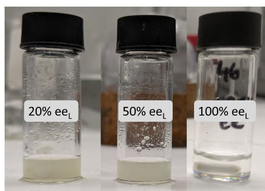
Figure 3. Reaction medium (Ligand, substrate, diethylzinc, toluene) as function of the optical purity of the NPNE ligand. From left to right: 20% ee L ; 50% ee L ; 100% ee L .
