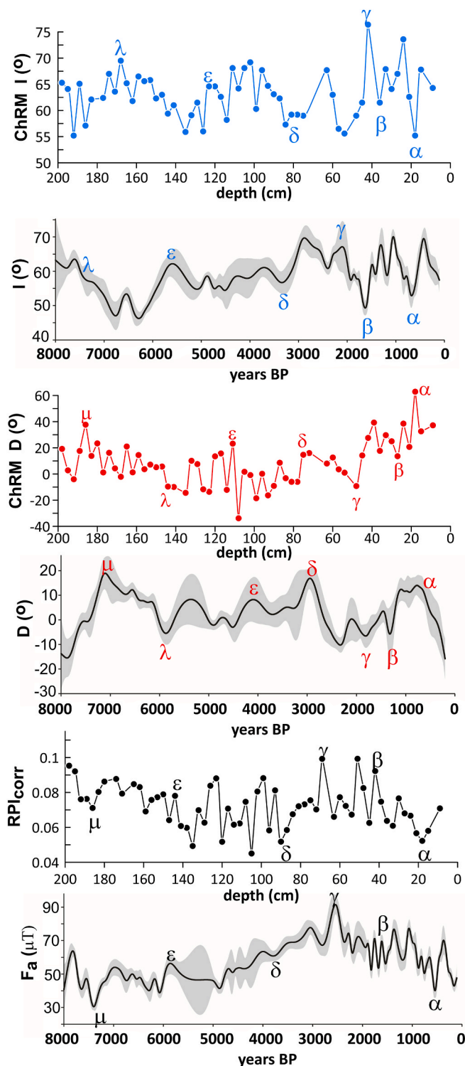
Fig. 8. Correlations between depth variations of the inclination ( I ) and declination ( D ) of the characteristic remanence (ChRM) and relative paleointensity (RPI) estimates with Bulgarian archaeomagnetic master curves (Kovacheva et al., 2014) of the secular variations of declination ( D ), inclination ( I ) and intensity ( F_a ) of the Earth's magnetic field for the last 8000 y BP. Tie points are marked by Greek letters of the same colour for the respective parameters compared.
