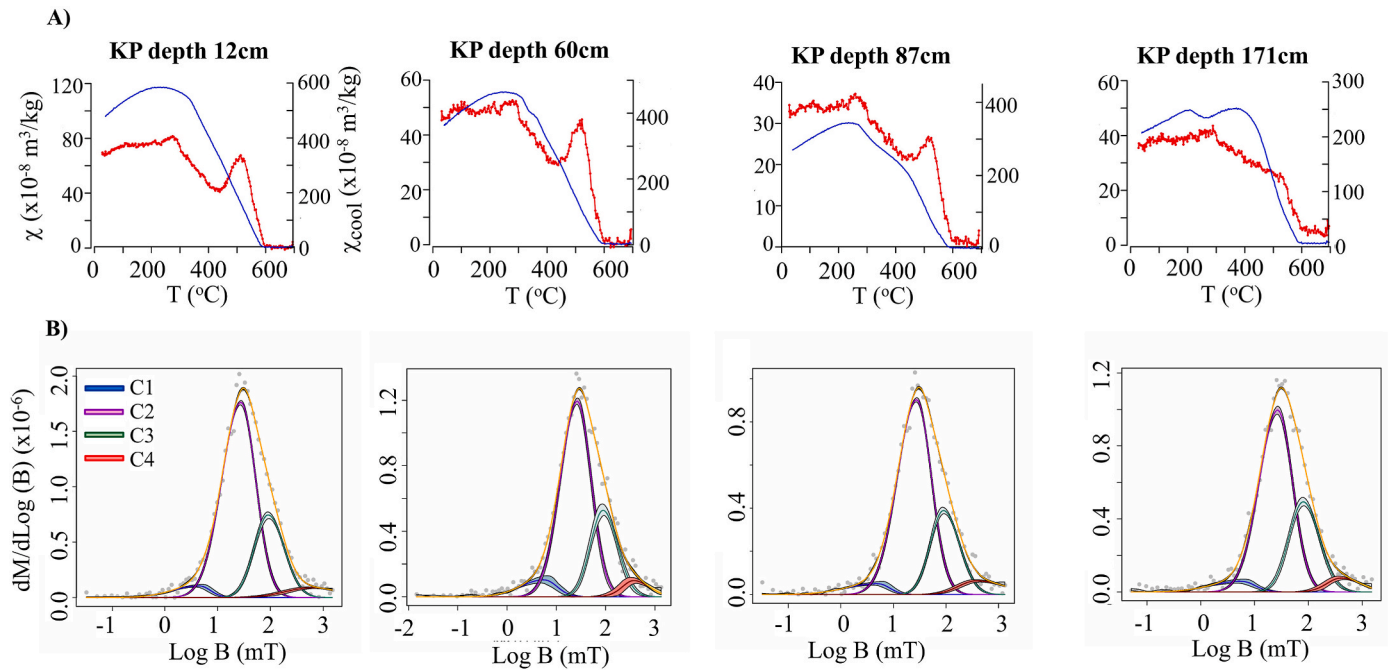
Fig. 3. A) Representative thermomagnetic analyses of magnetic susceptibility ( \chi(T) ) of samples from different depth intervals – heating in air at 11 °C/min; B) Unmixing of IRM stepwise acquisition curves for the same samples shown in (A) using the MaxUnMix software (Maxbauer et al., 2016). Data points are denoted by dots; cumulative fit together with its confidence band is shaded in yellow. Color coding of the fitted components C1, C2, C3 and C4 is given in the left panel of (B). (For interpretation of the references to color in this figure legend, the reader is referred to the Web version of this article.)
