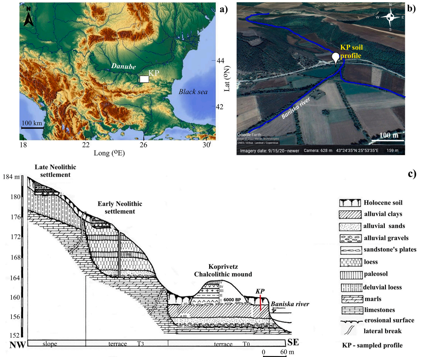
Fig. 2. (a) Location of Koprivetz (KP) site (indicated by white rectangle) in the lower Danube area (map from MFF maps (Braxmeier, 2017); b) map showing the position in the landscape of the sampled soil profile KP (shown by the white symbol). Map created in Google Earth (2022). Nearby Neolithic village is positioned at the slope of the hill from northwest and the Chalcolithic mound is next to the sampled soil profile at the flood terrace of Baniska river; c) geological section of the site (modified after Evlogiev, 2006).
