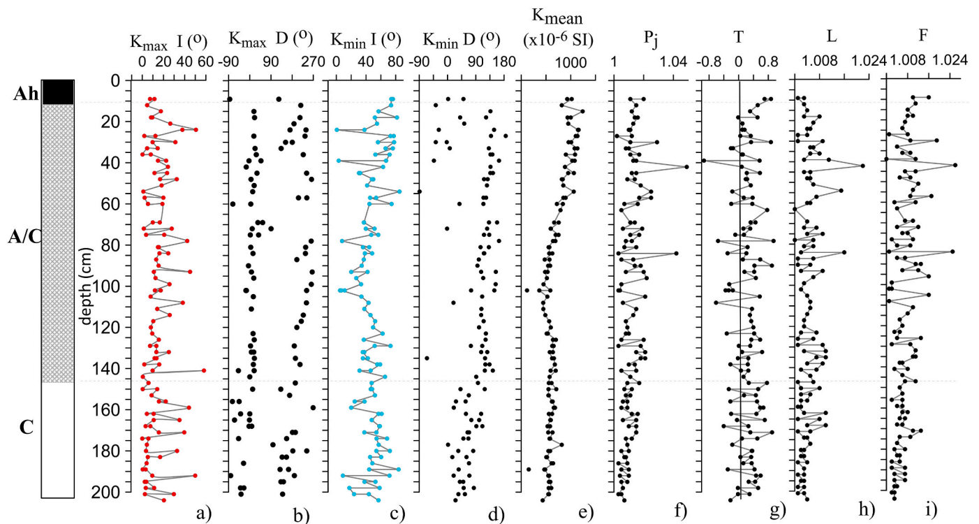
Fig. 7. Variations with depth of declination and inclination of K_{\max} and K_{\min} (a–d); mean volume susceptibility ( K_{\text{mean}} ) (e) and anisotropy parameters: corrected degree of anisotropy (Pj), shape parameter (T), lineation (L) and foliation (F).
