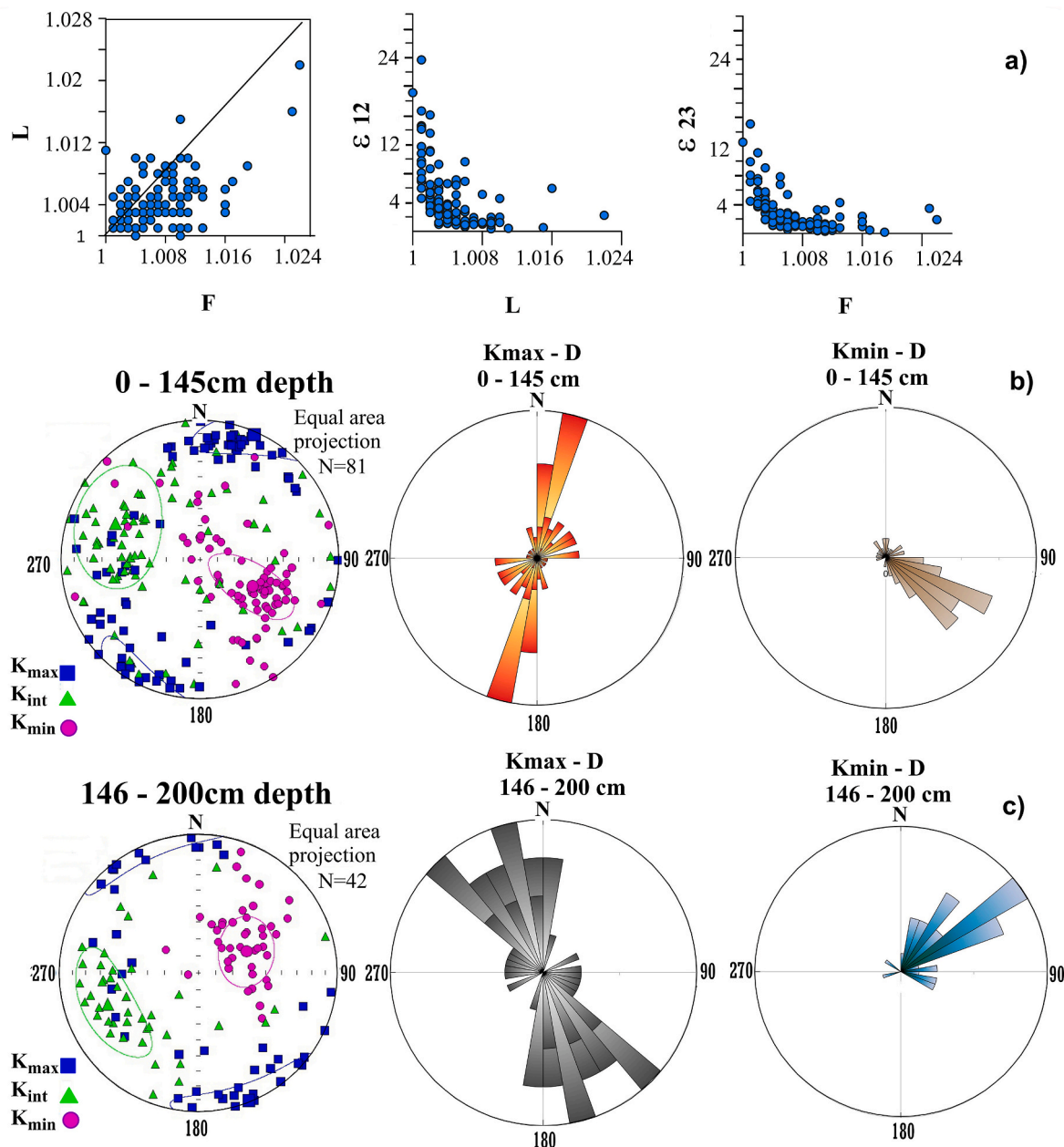
Fig. 6. Results from anisotropy of magnetic susceptibility measurements. A) bi-plots of lineation (L) versus foliation (F); 95% confidence half angle around K_{max} and K_{int} within the K_{max} - K_{int} plane ( \epsilon_{12} ) versus magnetic lineation L, and around K_{min} and K_{int} within the K_{min} - K_{int} plane ( \epsilon_{23} ) versus F; b) lower hemisphere stereographic projection (geographic coordinates) of the maximum ( K_{max} ), intermediate ( K_{int} ) and minimum ( K_{min} ) AMS principal axes of samples from the soil Ah and A/C horizons developed in deluvial clays; rose diagram of the K_{max} declinations and plunge of the poles to the imbrication plane (D- K_{min} ). c) the same as b) for samples from the alluvial clays in the C horizon.
