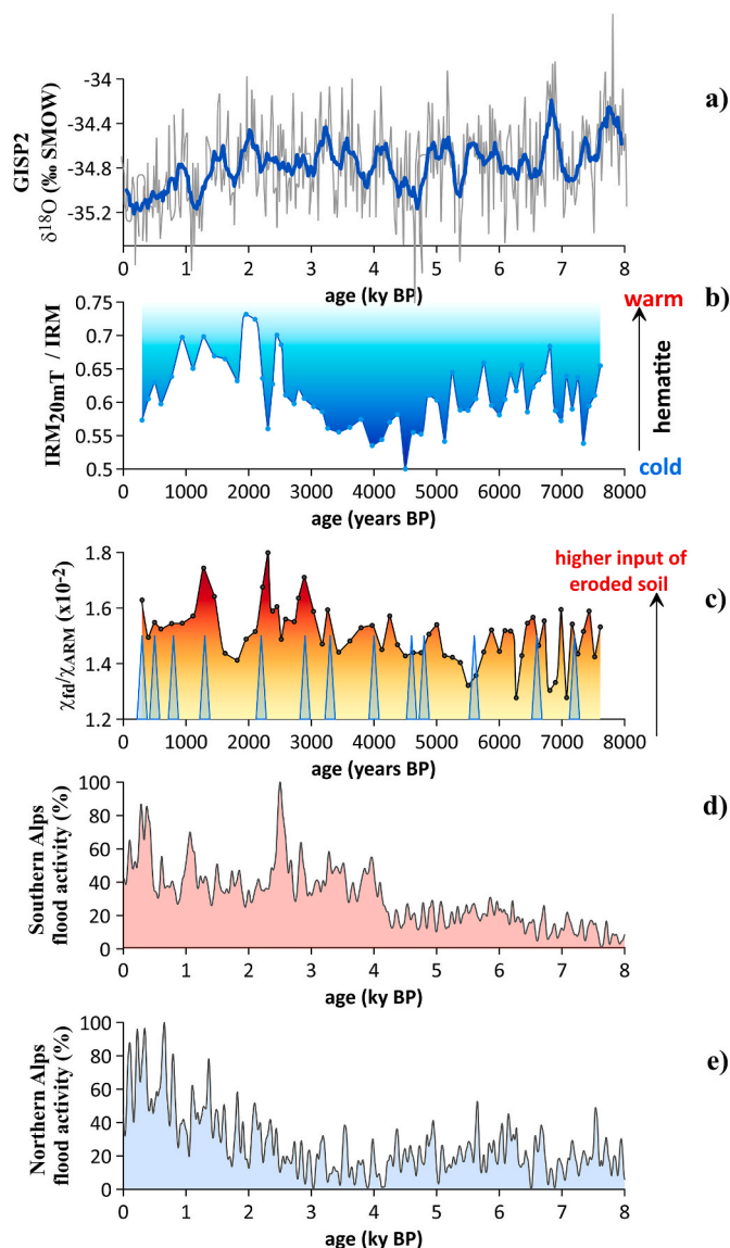
Fig. 9. Correlation of Greenland temperature record from GISP2 ice core (a) deduced from \delta^{18}O variability (data from Grootes and Stuiver (1999), defined relative to standard mean ocean water (SMOW) composition with 10-points running average) with environmental proxy ratio IRM_{20mT}/IRM (b) for soil profile KP; c) Variability of \chi_{fd}/\chi_{ARM} ratio as compared to Southern (d) and Northern (e) Alps flood activities from Wirth et al. (2013a). Blue cones in (c) depict the timing of major flood events at Romanian Carpathian rivers according to Radoane et al. (2019). (For interpretation of the references to color in this figure legend, the reader is referred to the Web version of this article.)
