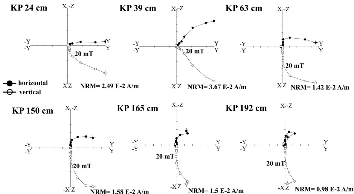
Fig. 5. Orthogonal vector plots of NRM AF stepwise demagnetization. 20 mT step is indicated as the first point of the isolated ChRM.
