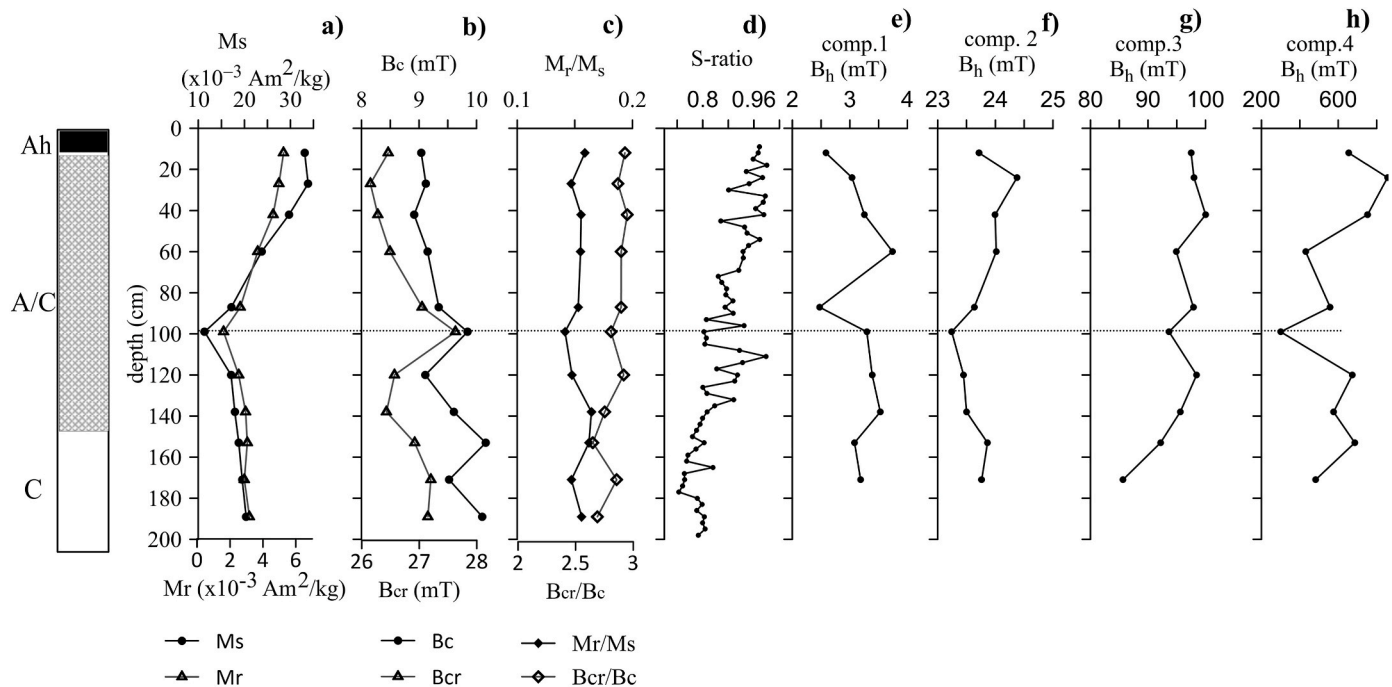
Fig. 4. Depth variations of hysteresis parameters and ratios (a–c); S-ratio (d), and mean coercivities ( B_h ) of the four IRM components fitted to IRM acquisition curves (e – h). Stratigraphic column with soil horizons is shown on the left.
