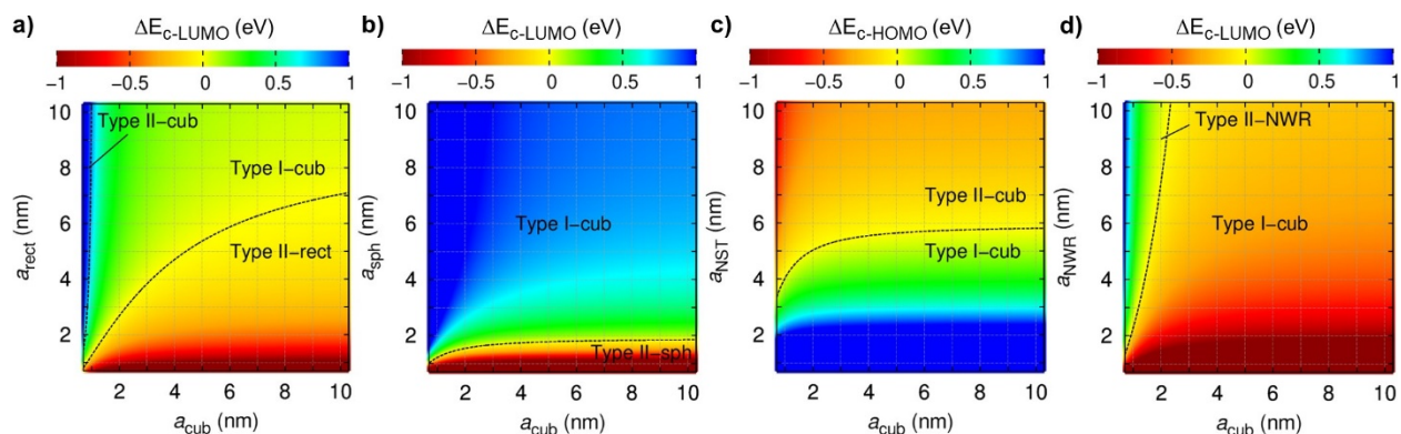
Figure 3. Energy maps for the electron/hole injection barriers as function of the NP characteristic length for the junctions formed by a cubic \text{WO}_3 ( x -axis) and the rest of \text{WO}_3 families ( y -axis) of NPs. Energy scales indicating the difference in c-HOMO/c-LUMO values ( \Delta E_{c\text{-HOMO}/c\text{-LUMO}} = E_{c\text{-HOMO}/c\text{-LUMO}}(x\text{-axis}) - E_{c\text{-HOMO}/c\text{-LUMO}}(y\text{-axis}) ) are presented on the top of the plots. The rest of the \text{WO}_3 NP based junction energy maps are collected in Figure S4.
