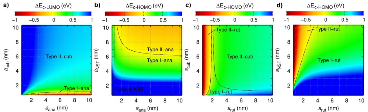
Figure 4. Energy maps for the electron/hole injection barriers as function of the NP characteristic length for the junctions formed by anatase (a- and b-) and rutile (c- and d-) \text{TiO}_2 NPs ( x -axis) with
