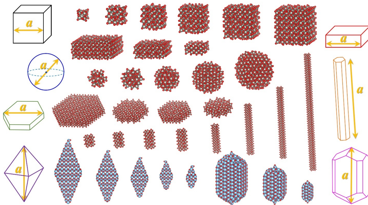
Figure 1. The full set of \text{WO}_3 and \text{TiO}_2 NPs investigated in this work (from the top to the bottom and from the left to the right): n=8, 27, 64, 125, 216, and 343 cubic (\text{WO}_3)_n particles; rectangular-shaped (\text{WO}_3)_n particles with n=400, 147, and 32 ; spherical-shaped (\text{WO}_3)_n particles with n=19, 32, 57, 80, 147 and 281 ; hexagonal nanosheet (\text{WO}_3)_n particles with n=420, 180, 144 and 84 ; cuboid nanowires (\text{WO}_3)_n particles with n=18, 24, 30, 36, 66, 126, 186 and 306 ; anatase (\text{TiO}_2)_n
