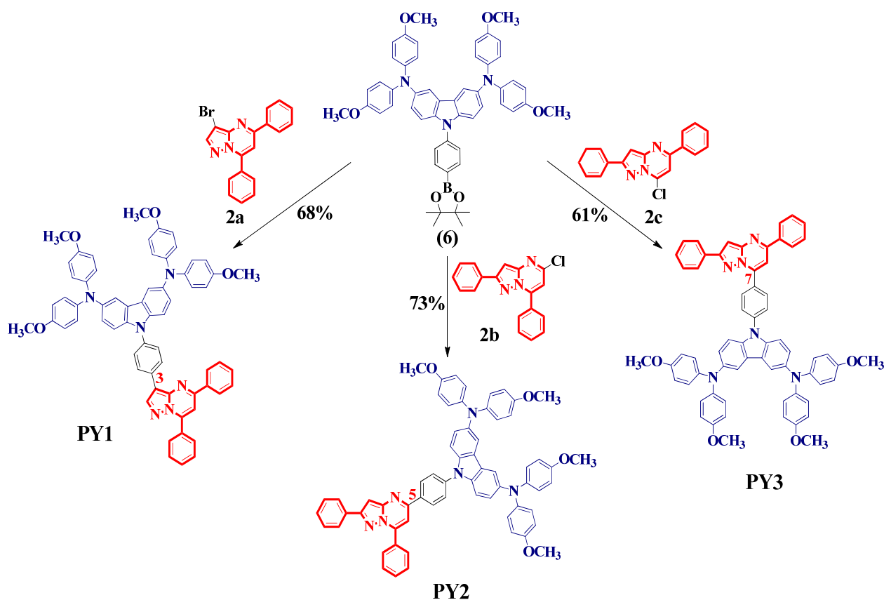
Figure 1. Synthetic route of PY1–PY3 molecules by Suzuki–Miyaura cross-coupling reaction. Reagents and conditions: 2a–c (1 equiv), compound 6 (1.1 equiv), \text{PddppfCl}_2 (0.1 equiv), \text{Na}_2\text{CO}_3 (5 equiv), 1,4-dioxane/water (5:1) under MW irradiation at 110 °C for 2 h.
