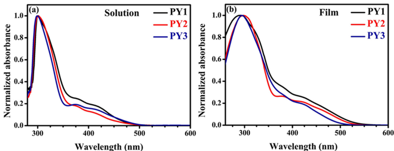
Figure 2. Normalized UV–visible absorption spectra in THF (a) and in thin film (b) of PY1 – PY3 .
