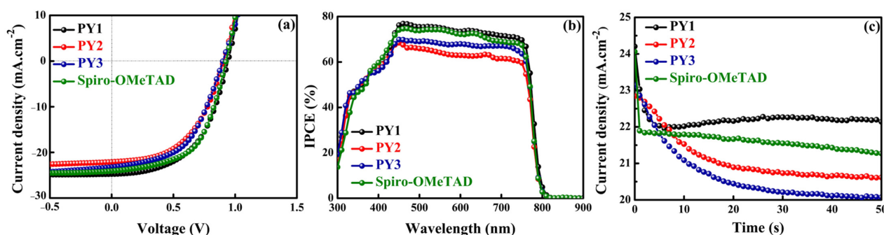
Figure 5. (a) Best J-V curves of the champion PSCs based on different doped HTMs measured under simulated AM1.5G illumination; active area = 0.20 cm 2 . (b) Corresponding IPCE spectra. (c) Stabilized photocurrent density obtained while holding the best PSCs at a bias voltage of 0 V and under continuous illumination.
