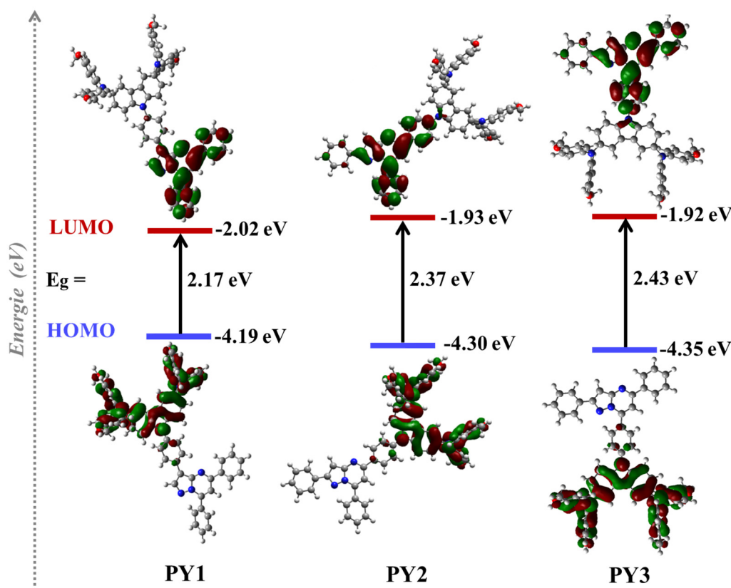
Figure 4. Optimized structures, HOMO and LUMO energy levels, energy gaps, and electron distributions of PY1 , PY2 and PY3 molecules calculated by DFT calculations at the B3LYP/6-31G level.
