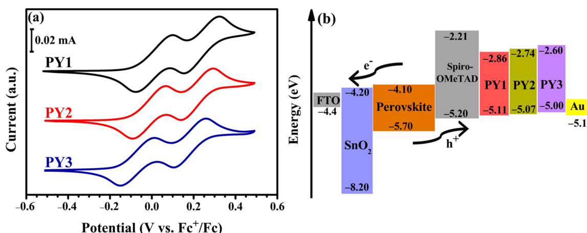
Figure 3. (a) CV of PY1 – PY3 in DCM ( 5 \times 10^{-3} M); potentials vs. \text{Fc}^+/\text{Fc} , 0.1 M \text{Et}_4\text{NBF}_4 at a platinum electrode, scan rate 5 \text{ mV s}^{-1} . (b) Energy level diagram of each material in the PSCs.
