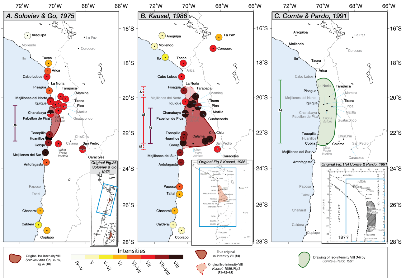
Figure 2: Comparison of intensities attributed by Soloviev and Go (1975) (A) ; Kausel (1986) (B) and Comte and Pardo (1991) (C). The same color scale for intensity is used for figures A and B. Insets depict the original figures from articles; in which light blue squares frame the region of interest in North Chile and Southern Peru. Lengths A0 in (A) and A0 & A1 in (B), later interpreted as "the rupture length", depict the N-S extension of the area of intensities larger than VIII. Lengths A2 & A3 in (B) depict the rupture length extensions to Pisagua to the North and to Mejillones to the South mentioned in Kausel (1986). Length A4 depicts the extended rupture length of Comte and Pardo (1991). All locations with intensity reports are indicated on maps A and B, but those ignored by a specific author are in light gray. Note Chiu-Chiu is mislocated in Comte and Pardo (1991) Fig 1e.
