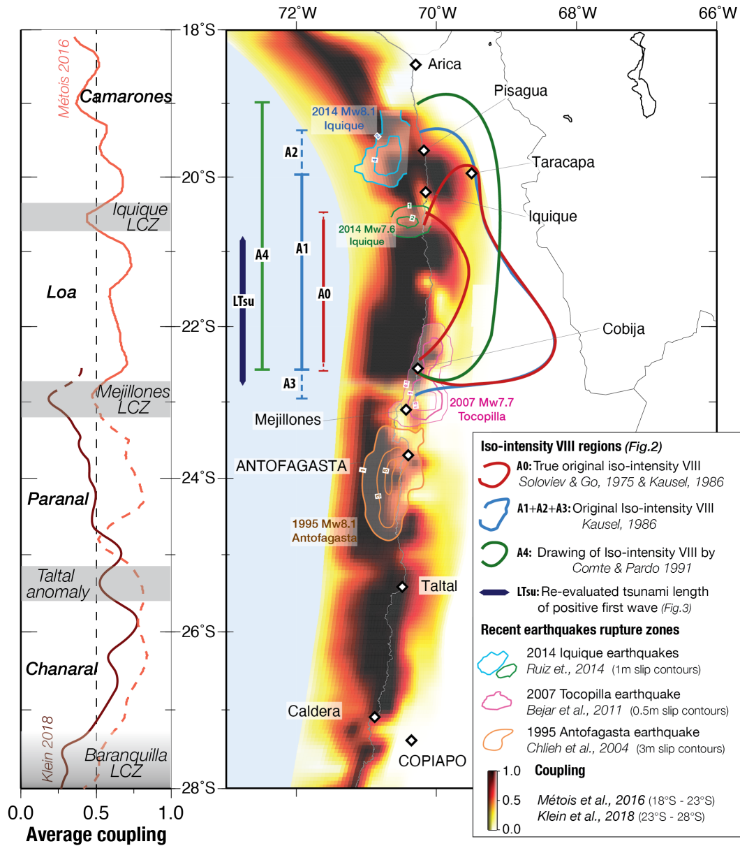
Figure 5: Comparison of iso-intensity VIII with geodetic coupling and rupture zones of modern earthquakes. Coupling maps (right panel) and average coupling curves (left panel) are from Métois et al. (2016) in-between 18°S and 23°S and from Klein et al. (2018) in-between 23°S and 28°S. Earthquake Slip models are depicted by colored contour lines. Antofagasta 1995 (Mw8.1, Chlieh et al. (2004) - orange), Tocopilla 2007 (Mw7.7, Béjar-Pizarro et al. (2013) - purple), Iquique 2014 (Mw8.1 & Mw7.8, Ruiz et al. (2014) - blue & green). Original iso-intensity VIII areas from Soloviev and Go (1975) and Kausel (1986) (red curves & red length A0); enlarged iso-intensity VIII by (Kausel, 1986) (blue curve & blue length A1+A2+A3) and (Comte and Pardo, 1991) (green curve & green length A4). Length LTsu (dark blue line) depicts the coastline length along which a positive first arrival was reported in (Geinitz, 1878) (Fig.3).
