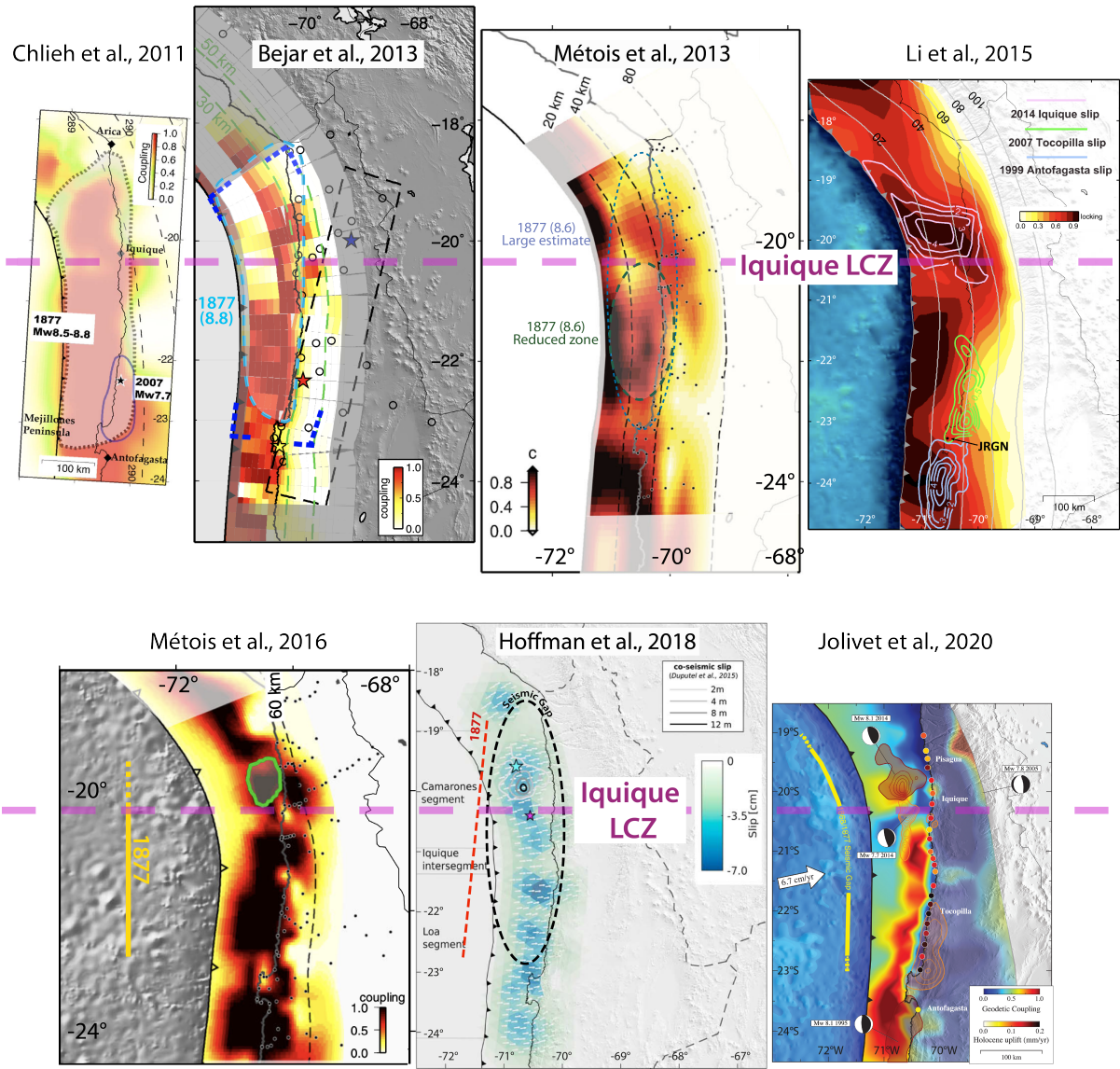
Figure 1: Comparison of coupling models inferred in North Chile from the present-day geodetic measurements. From left to right top row: elastic backslip 3-plates model inferred from GPS by Chlieh et al. (2011); elastic backslip 2-plates model inferred from combined GPS and InSAR by Béjar-Pizarro et al. (2013); elastic backslip 3-plates model inferred from GPS by Métois et al. (2013); visco-elastic coupling model inferred from GPS by Li et al. (2015); bottom row: elastic backslip 3-plates model inferred from GPS by Métois et al. (2016), elastic backslip 3-plates model inferred from GPS by Hoffmann et al. (2018) and elastic backslip 2-plates model inferred from combined GPS and InSAR by Jolivet et al. (2020). All figures, extracted from original publications, were rescaled and rotated to be aligned. Figures from Chlieh et al. (2011) and Jolivet et al. (2020) show the extension of the 1877 North Chile earthquake. When available, we reported the rupture zone exactly as it was drawn on other figures of the articles (from Fig.1 of Béjar-Pizarro et al. (2013), Fig.5 of Métois et al. (2013), Fig.2 of Métois et al. (2016) and Fig.1 of Hoffmann et al. (2018)). The purple dashed line is located at the same latitude on both rows and highlights the latitude of the Iquique LCZ.
