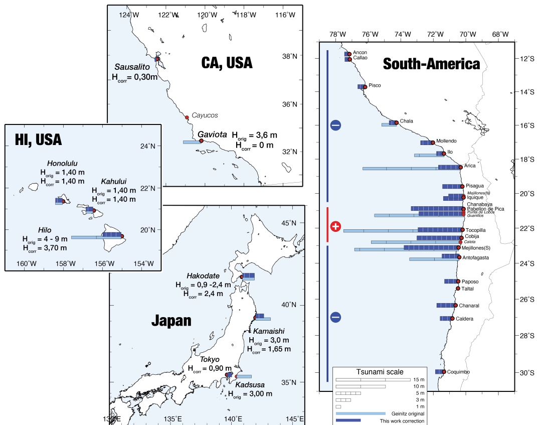
Figure 3: tsunami heights : original vs revised numbers. Original heights reported by Geintz (1878) are depicted in light blue (values listed in tables 1 and 2). Revised numbers according to discussion in section 3 are depicted in dark blue (values listed table 3). The same scale is used for all 4 maps. The plus symbol & red line and the minus symbol & blue line along the Chilean & Peruvian coastlines (South-America inset) depict the polarity of the first arrival : - correspond to the report of an initial withdrawal of the sea, + correspond to the report of a sudden flooding (cf. table 1).
