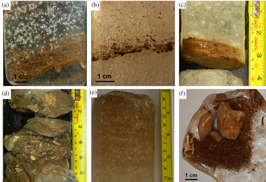
Fig. 8. Examples of the various forms of sediment inclusions found in the ice. (a) A band of suspended sediments at 45 cm depth in the upper section of IP1; (b) a thin layer of fine-grained sediments at 145 cm (lower section) depth in IP2; (c) a 2 cm thick band of compact fine-grained sediments at 135 cm depth (lower section) in IP2; (d) a 15 cm thick band of ice-bonded gravel and sand at 190 cm depth in IP1; (e) brown coloration of ice sample IS#2 collected in the seasonal fringe of IP1 due to suspended very fine sediments; (f) mix of gravels and fine-grained sediments frozen in the side of a supra-ice channel on IP1.
